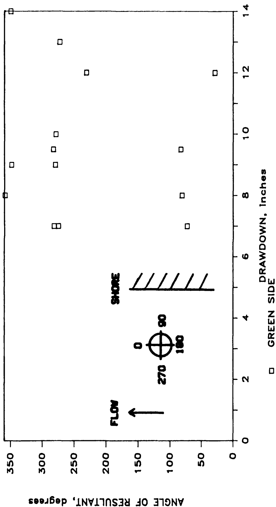
Figure 16. Resultant Direction of Sediment Movement from Trap Data in Relation to Measured Drawdown, Upbound Vessels
