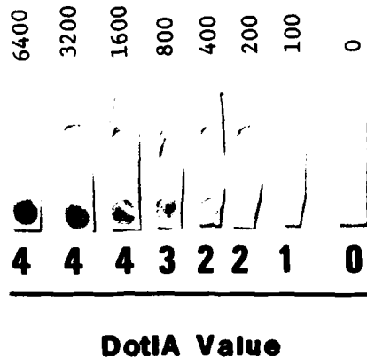
FIGURE 4. Multiple antigen DotIA assay strip for SLE/normal mouse brain/EEE (top to bottom). Each strip represents an assay of anti-EEE chicken sera of various EIA titers (serial two-fold from 6,400 to 100). Corresponding DotIA values are given.
