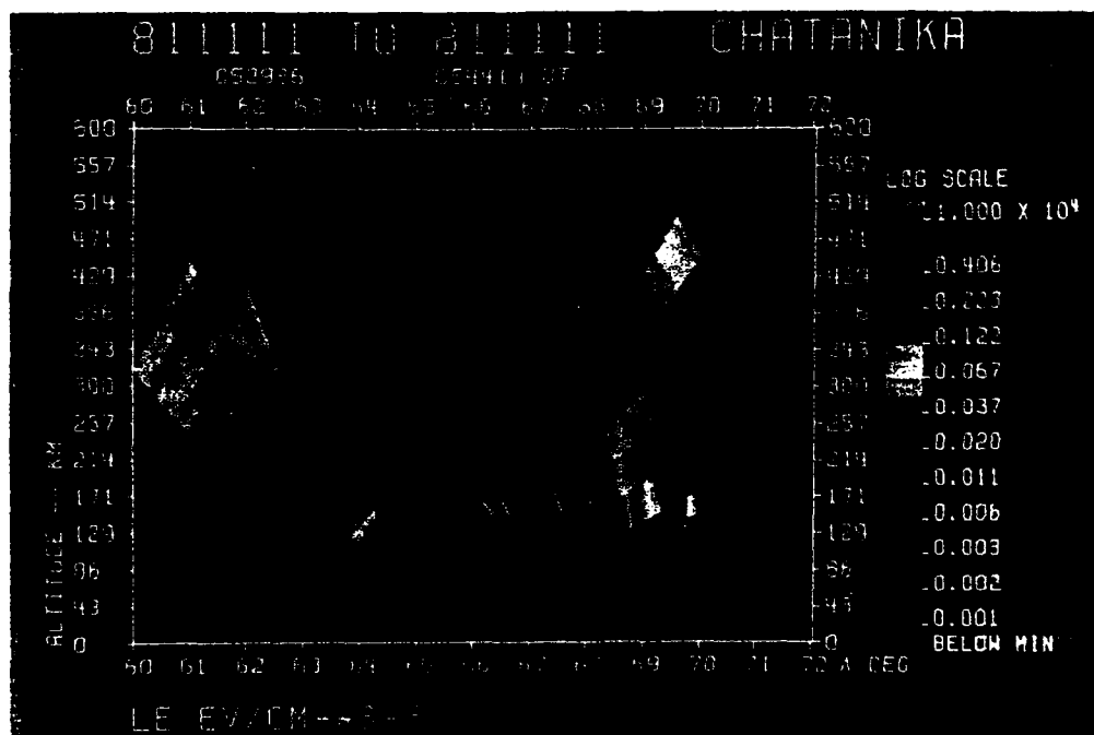
Plate 3. Energy input to the electron gas, L_e , deduced from the radar data for the scan simultaneous to the DE pass. L_e does not increase above the background inside the ionization channel at 66.2°.
