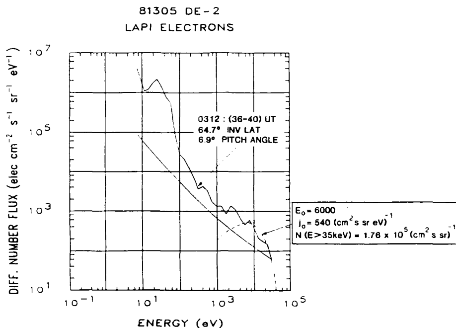
Figure 6. LAPI electron differential number spectrum measured at 0312:(36-40) UT. The Maxwellian (dashed) curve fitted to the measured spectrum contains an integral flux of 1.76 \times 10^5 \text{ cm}^{-2} \text{ s}^{-1} \text{ sr}^{-1} at energies exceeding 35 keV. This more than accounts for the flux of \sim 9 \times 10^4 \text{ cm}^{-2} \text{ s}^{-1} \text{ sr}^{-1} measured by the 0^\circ Geiger tube (see Fig. 5).
