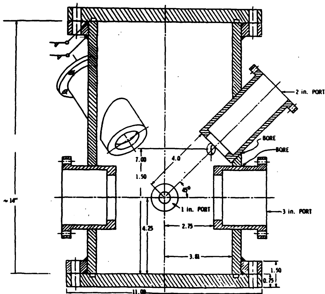
Figure 28. Side View of Window Bomb. The 45° viewing angle allowed us to survey the entire active surface of the strand.
