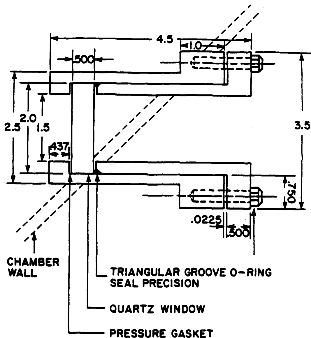
Figure 4. Reentrant Window Port . This design maximized optical access.
