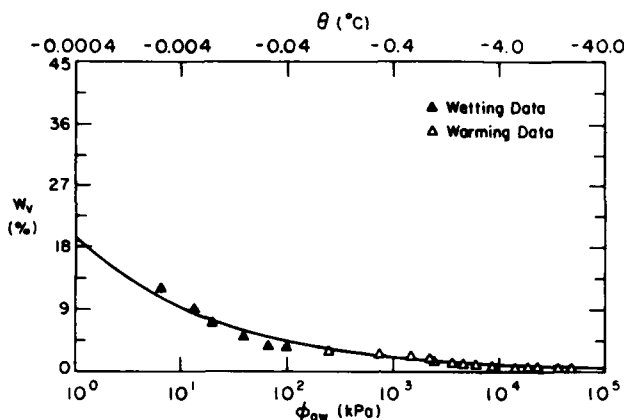
b. Wetting curve data from SWC of Iskandar et al. (1979). Warming curve data from SFC, \rho_d = 1.79 \text{ g/cm}^3 .
