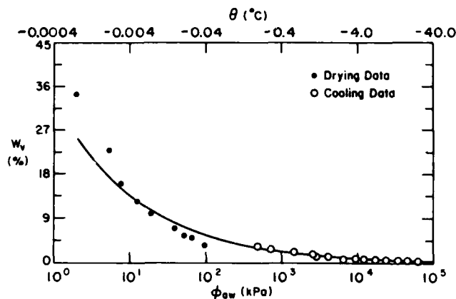
a. Drying curve data from SWC of Iskandar et al. (1979). Cooling curve data from SFC, \rho_d = 1.79 \text{ g/cm}^3 .
