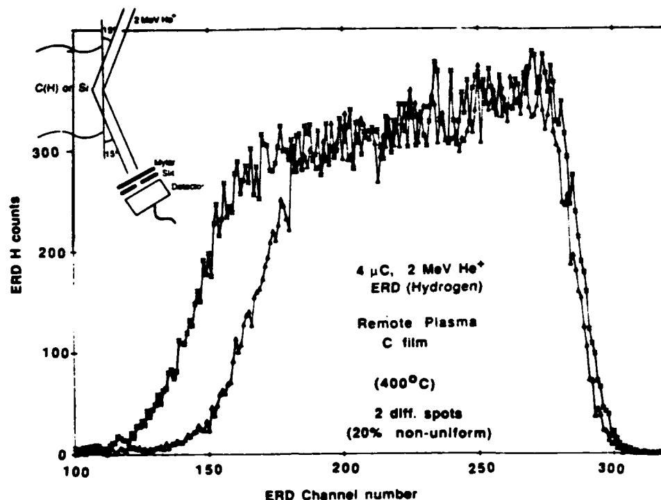
Fig. 1 Elastic recoil spectra recorded at 293K for two different spots on a RTI diamond-like C film, deposited by RPECVD at 400°C on a Si substrate. The incident He + energy was 2 MeV. The counted number of recoiled H + ions is plotted as a function of their energy (ERD channel number). The inset shows the sample vs detector configuration.
