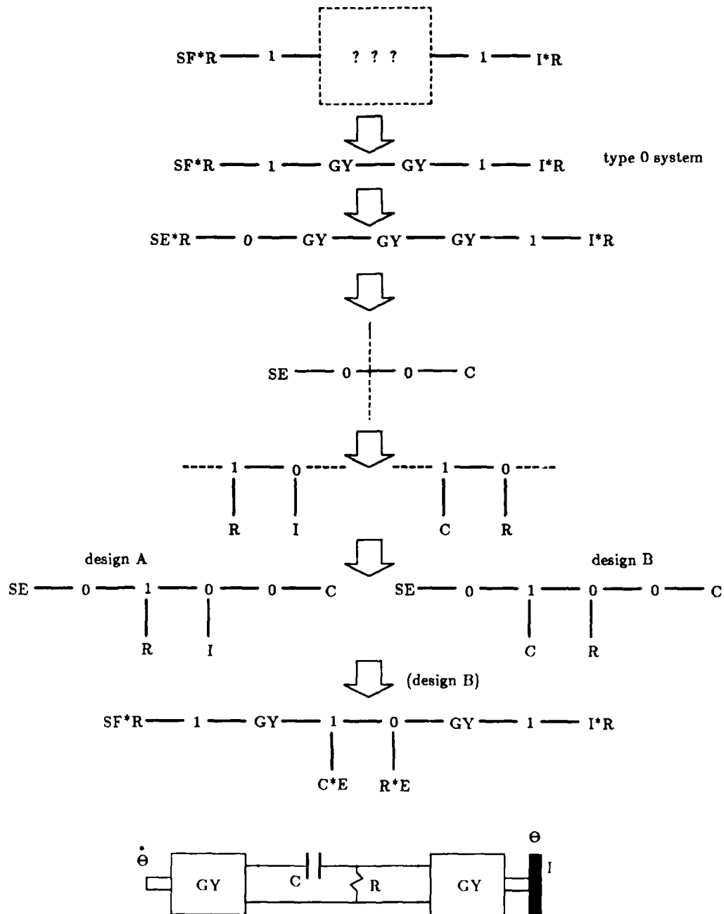
Figure 3.10: Speedometer synthesis
