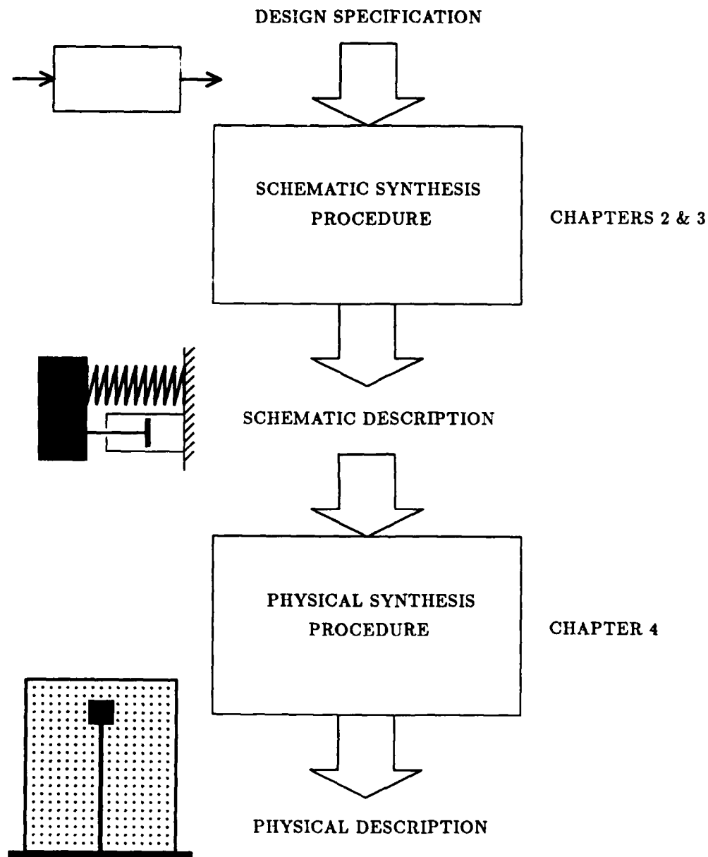
Figure 1.2: Problem decomposition
