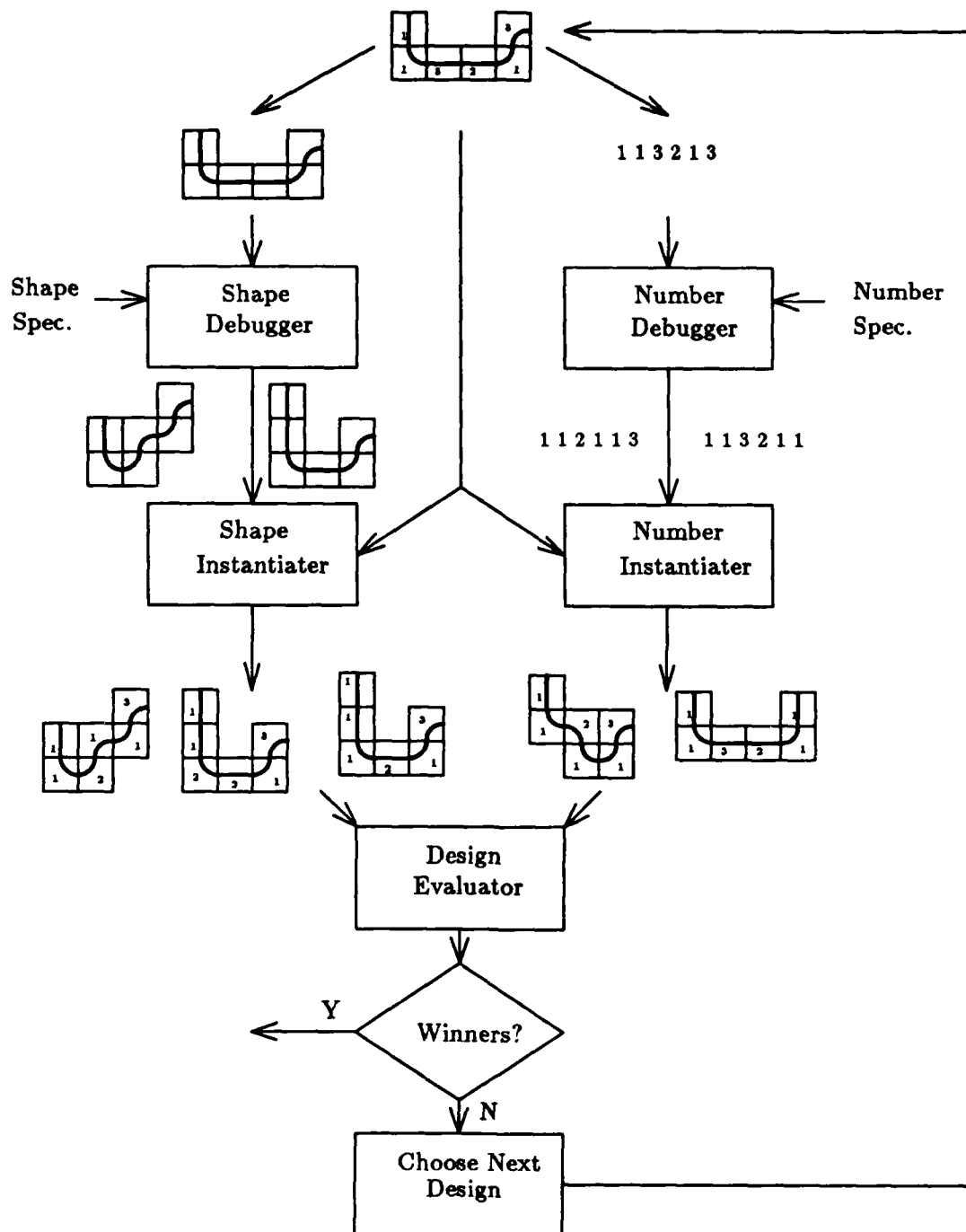
Figure C.4: Program architecture
