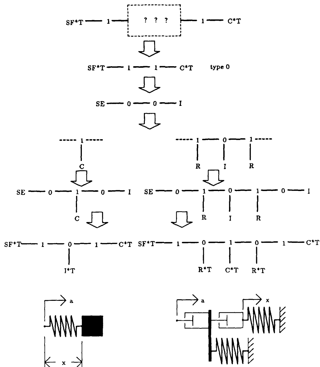
Figure 3.12: Accelerometer synthesis
