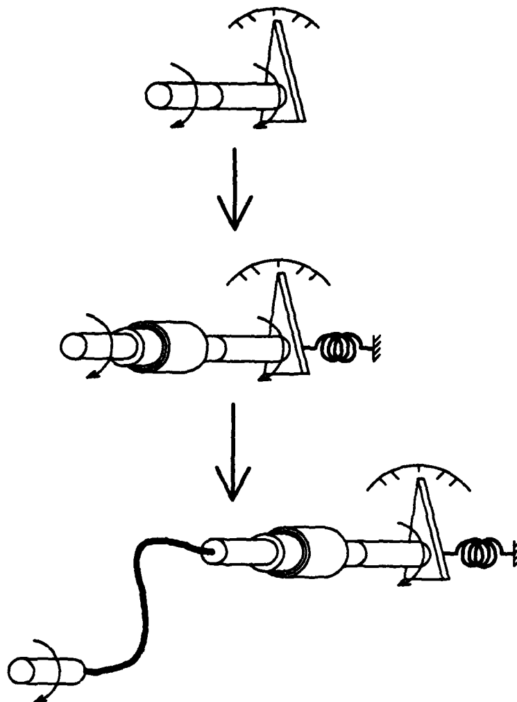
Figure C.5: Speedometer debugging
