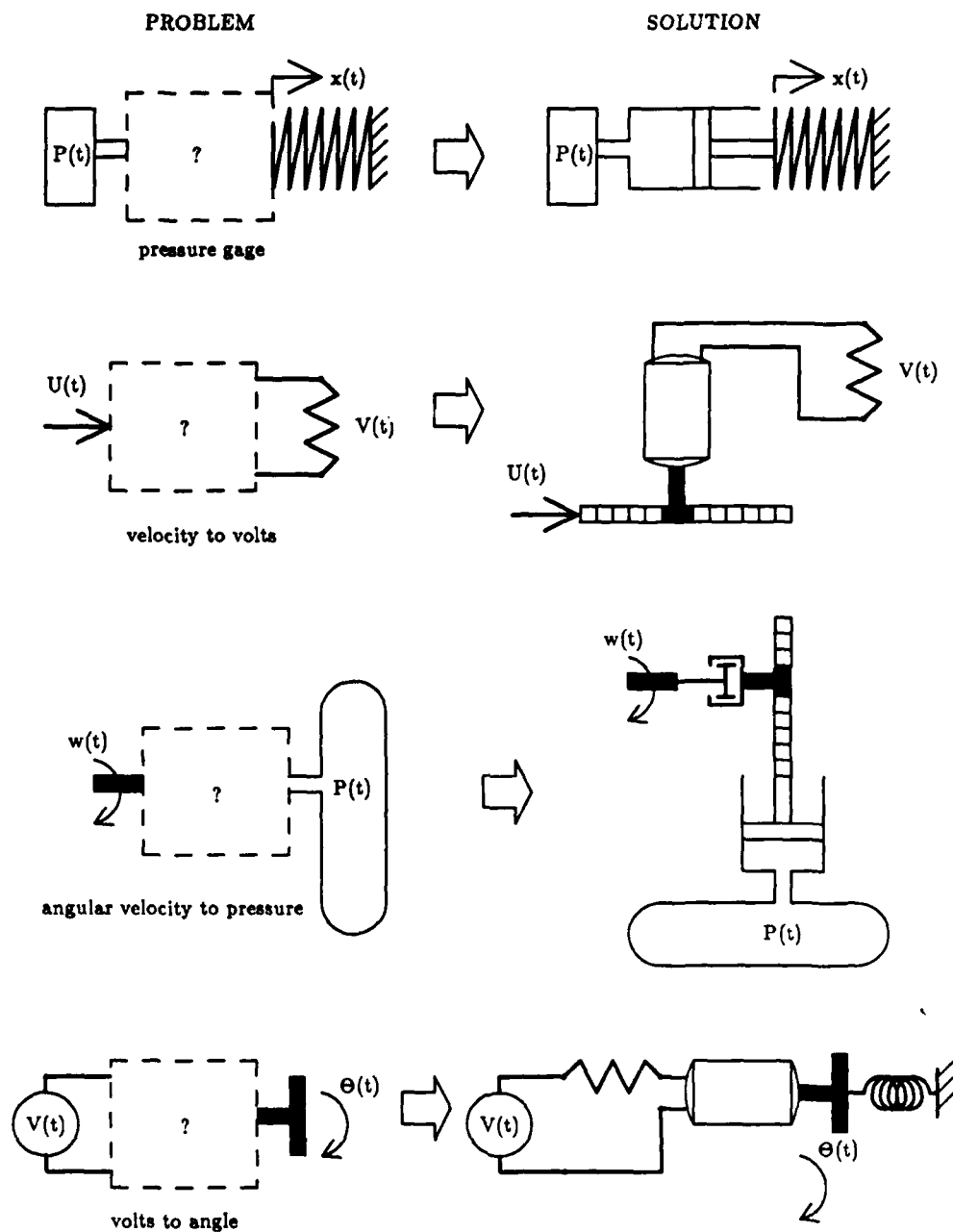
Figure 3.1: Example SISO dynamic systems problems and solutions.
