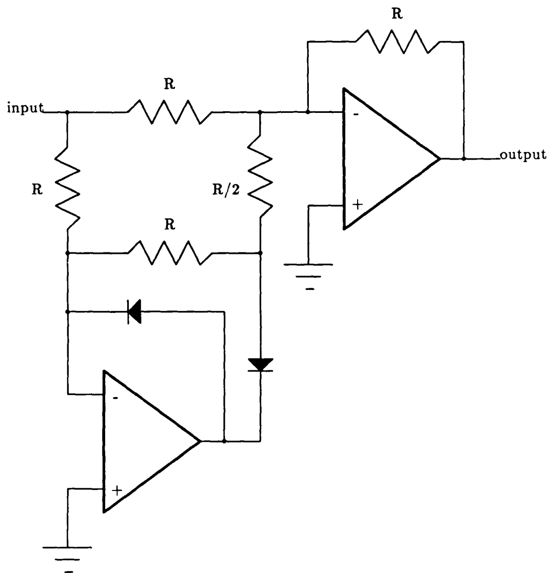
Figure 2.2: Schematic description of an analog circuit
