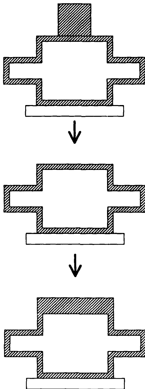
Figure 4.11: Accelerometer example 1.
