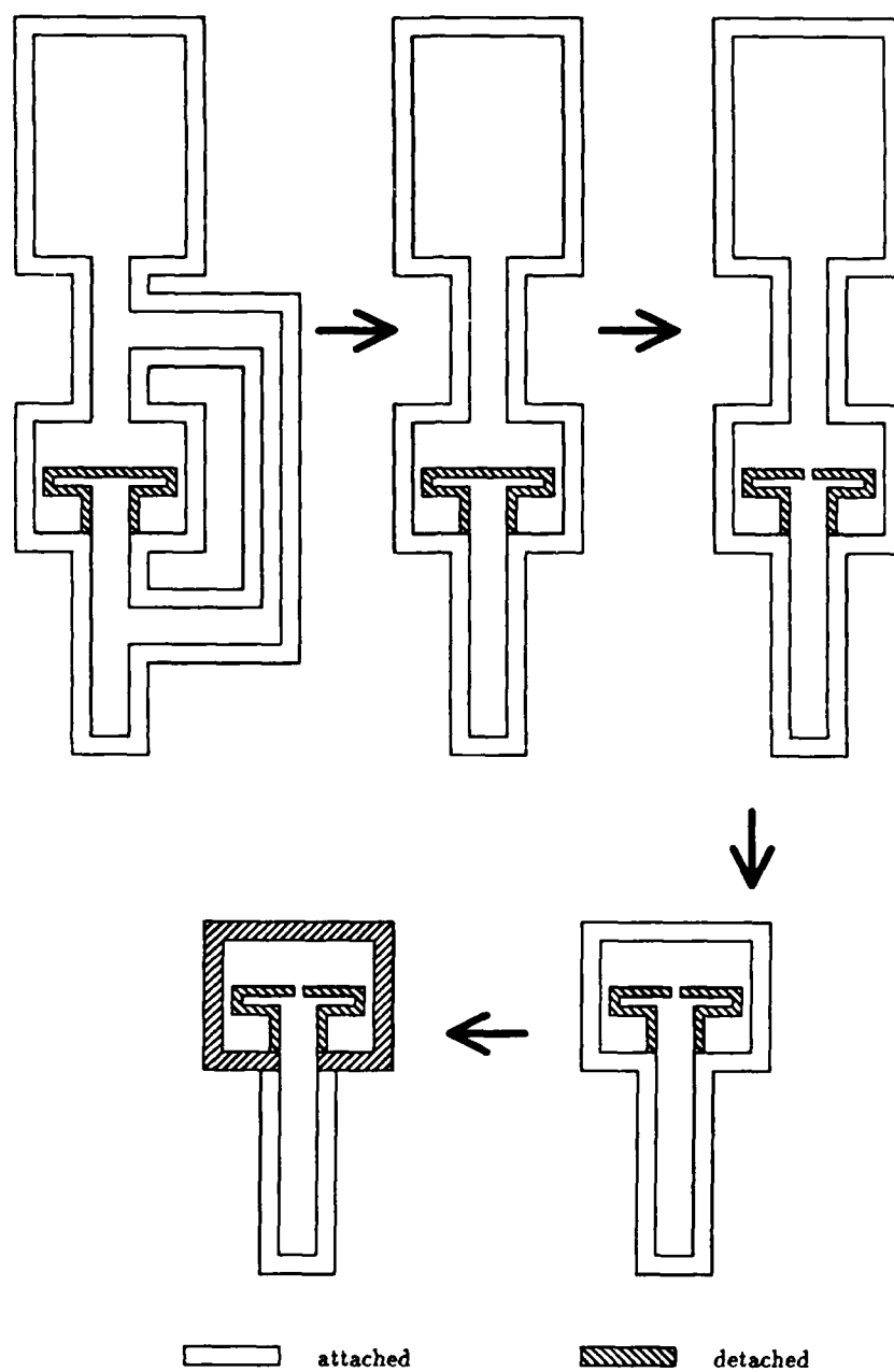
Figure 4.13: Rate-of-climb example 1.
