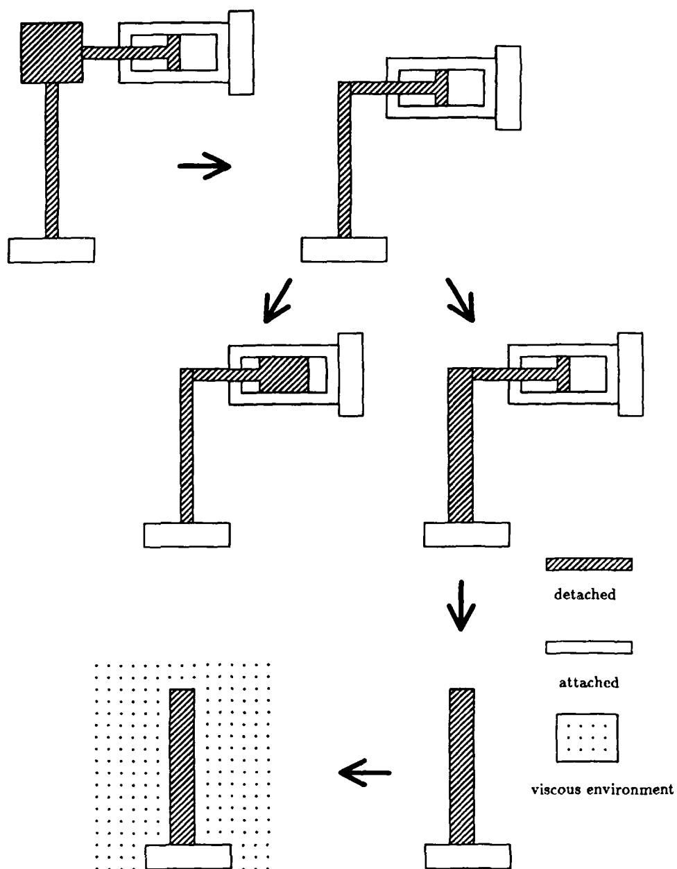
Figure 4.12: Accelerometer example 2.
