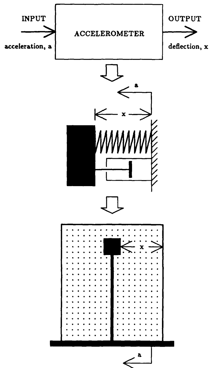
Figure 1.1: Scenario illustrating the design of an accelerometer
