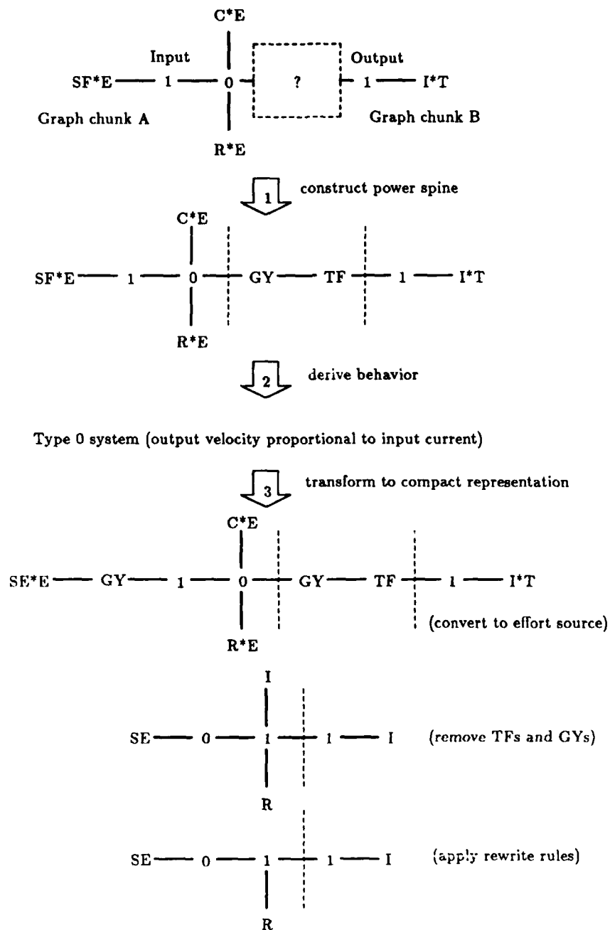
Figure 3.7: Current meter synthesis
