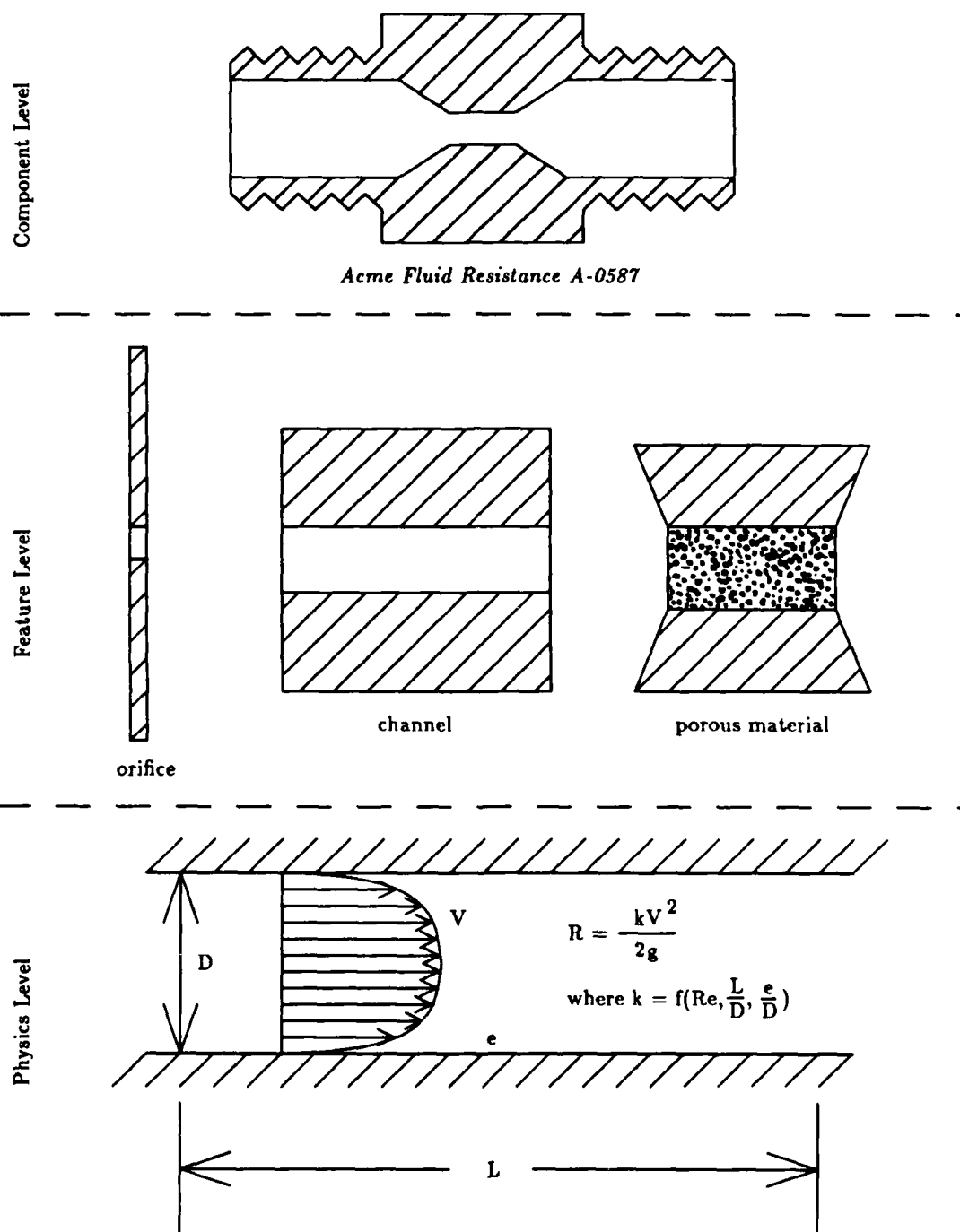
Figure 4.15: Knowledge level for fluid resistance.
