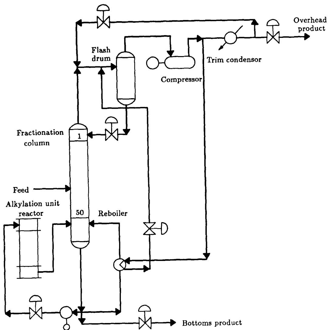
Figure 2.1: Schematic description of a process plant.
