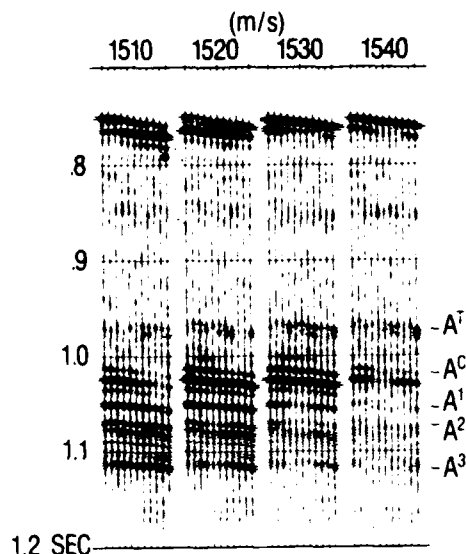
Fig. 5. CSP stacked traces from within region B-B' (Figure 2) are shown. The stacking velocities for the bottom reflection and for horizon A T are both ~1530 m/sec; this supports a low P-velocity gradient within the upper sediment column. The appropriate stacking velocity for horizon A 1 is ~1520 m/sec. This decrease in stacking velocity indicates a P-velocity inversion exists within the upper 300 m of the sediment column.
