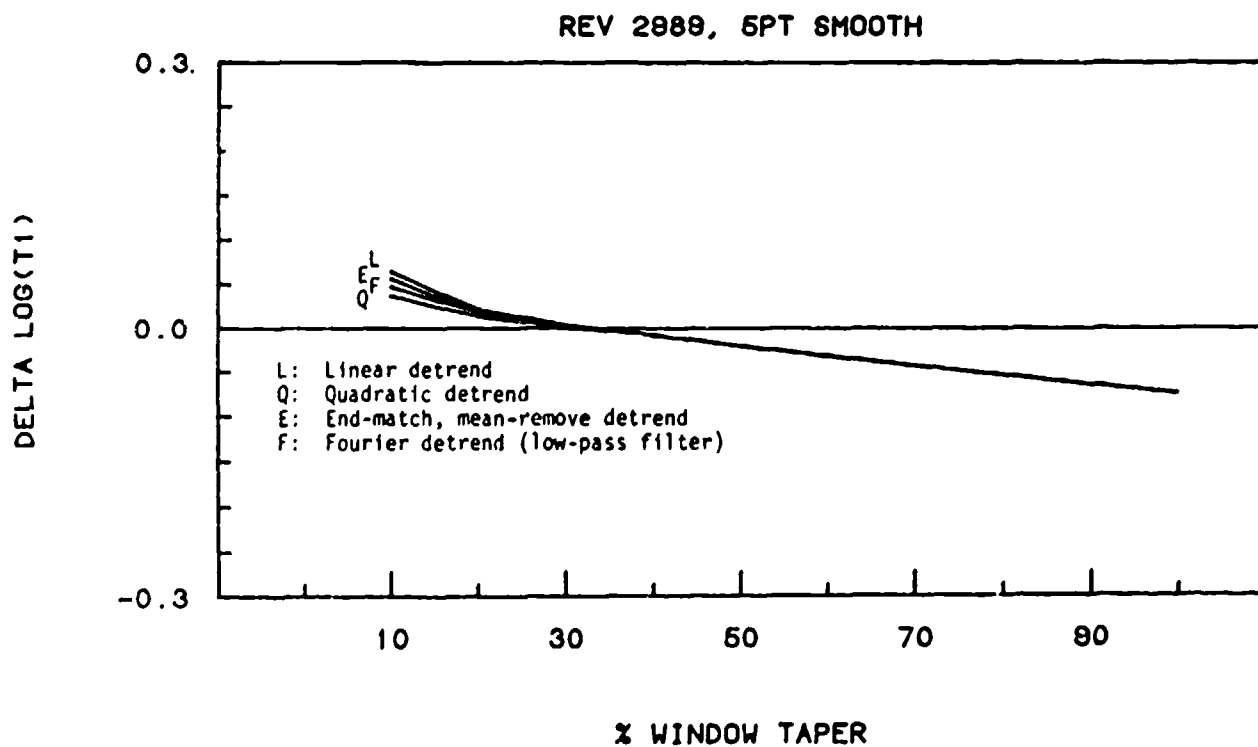
Figure 3. Detrender effects from analysis of data from Rev 2989. A five-point smoother was used in all cases.
