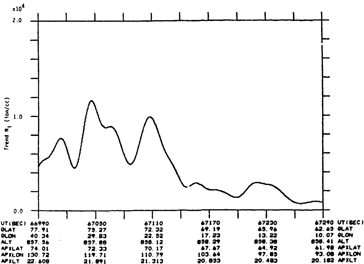
Figure A-01e. Ion density trend for AIO-EISCAT section of Rev 2862 (8 Jan 88). Detrender cutoff frequency of was 0.046875 Hz.
