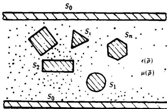
Fig. 1. Cross section of the transversely inhomogeneous multiconductor line with N conductors S_i and a conducting sheath S_0 . The unit vector \bar{u} and z coordinate are perpendicular to the plane.
