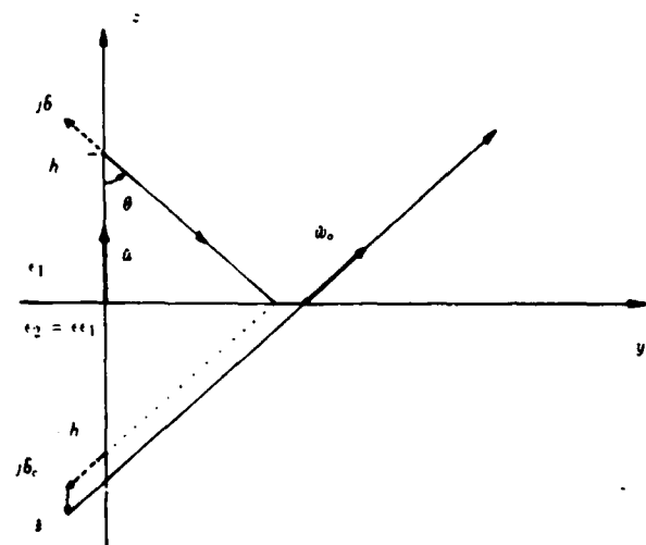
Fig. 1. Goos-Hänchen shift of the Gaussian beam arising from an approximate-image point source with a real shift vector \delta from the mirror-image point -\hat{u}h + j\delta_z .
