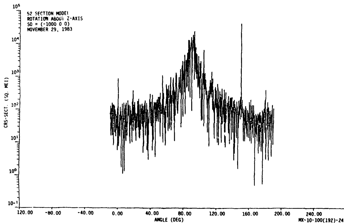
Figure 14. Helicopter Radar Cross-Section
