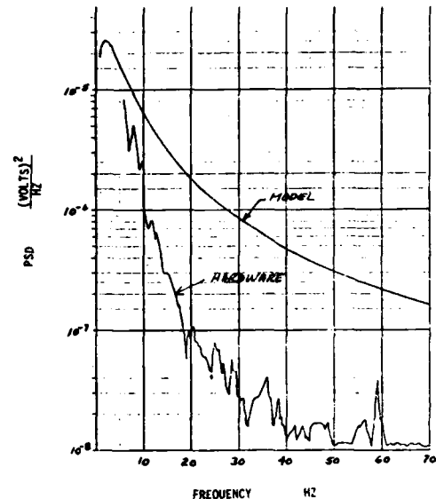
Figure 12 Gyro Noise
