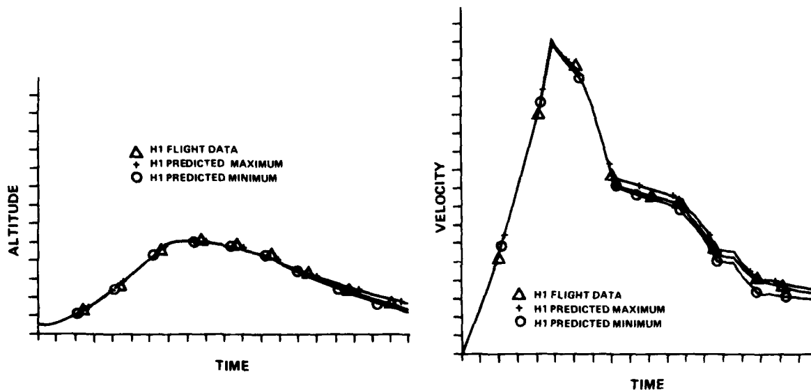
Figure 6. Typical System Level Validation Comparisons (Control Test Vehicle Flight).
