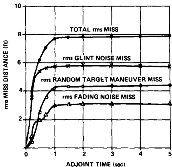
Figure 4. RMS Miss Distance Error Budget is Automatically Generated by Adjoint Method
