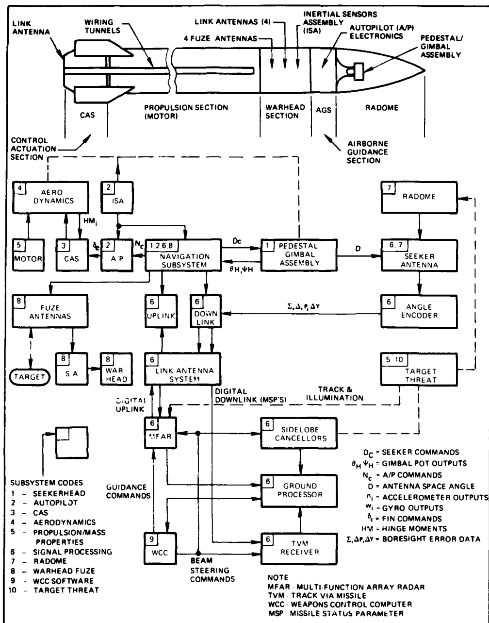
Figure 2. Guidance Simulation Models and Relation to System Hardware.
