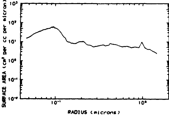
Fig. 13 Particle number concentration per \text{cm}^3 per micron (upper plot), particle mass concentration in grams per \text{cm}^3 per micron (centre plot) and particle surface area in \text{cm}^2 per \text{cm}^3 per micron (lower plot) as a function of particle radius in microns. Measurement period : April 19, 1988; 1330 - 1600 local time.
