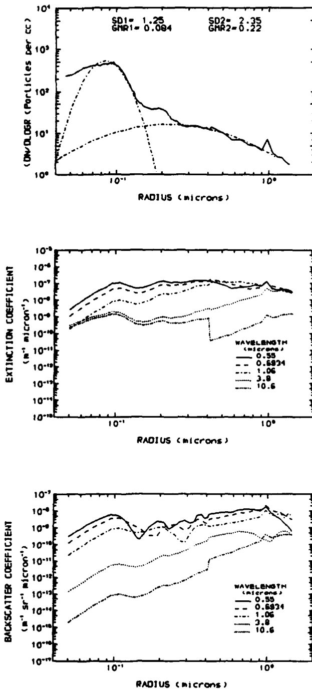
Fig. 14 Particle size distribution (upper curve) plotted in the form dn/dlogr versus particle radius r for the data of April 19, 1988; 1330 - 1600 local time. Two modes with log-normal parameter values for geometric mean radius (GMR) r_g and geometric standard deviation (SD) \sigma_g are fitted to the data.
