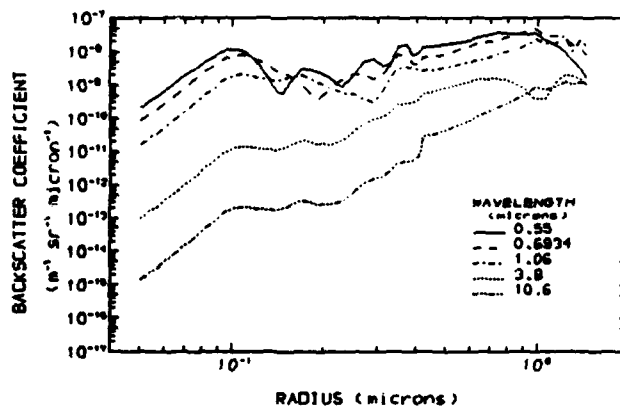
Fig. 18 As per Fig. 14 except for the measurement period : April 21, 1988; 0150 - 1245 local time.
