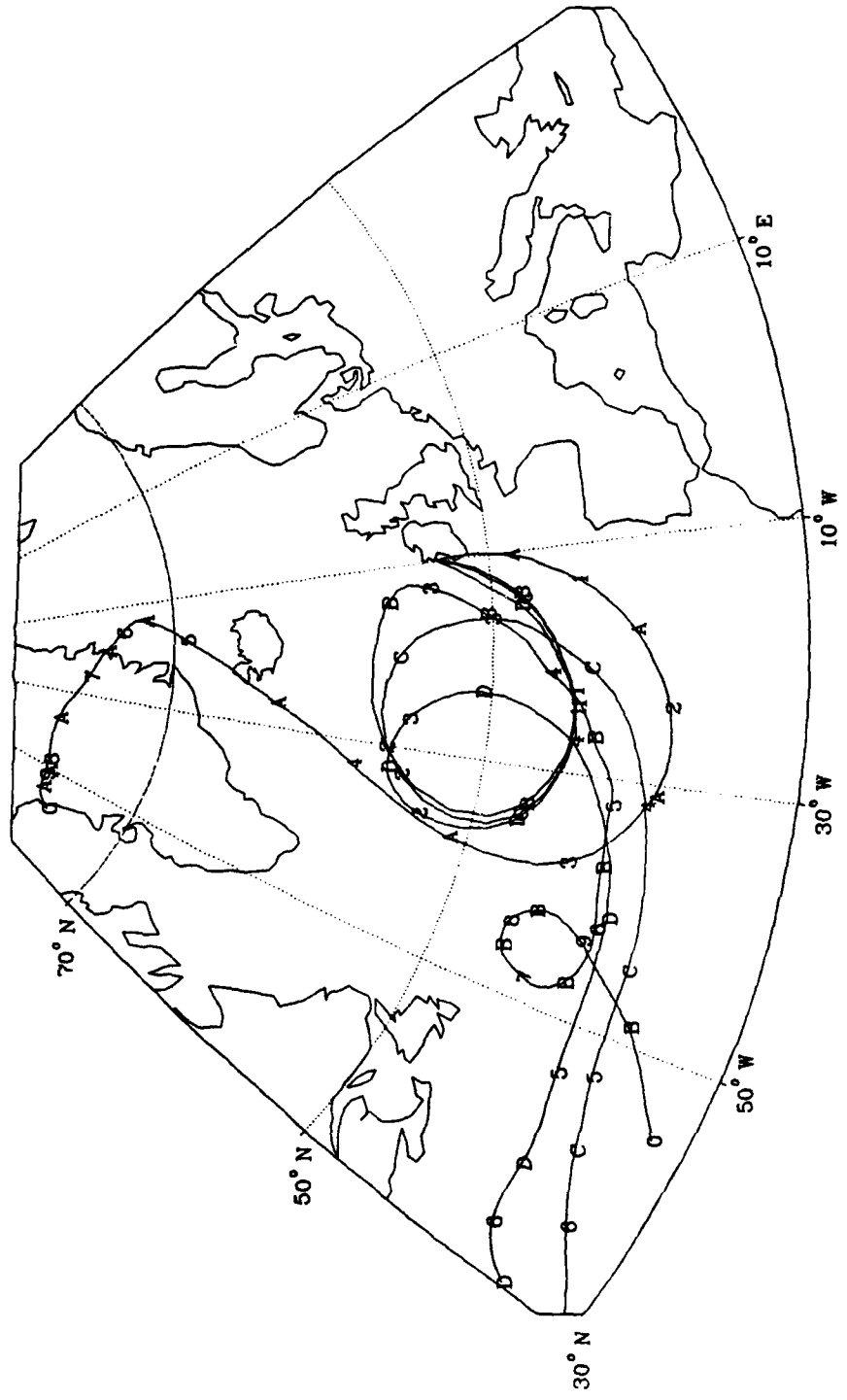
Fig. 7 As per Fig. 5 except for 20 April 1988
