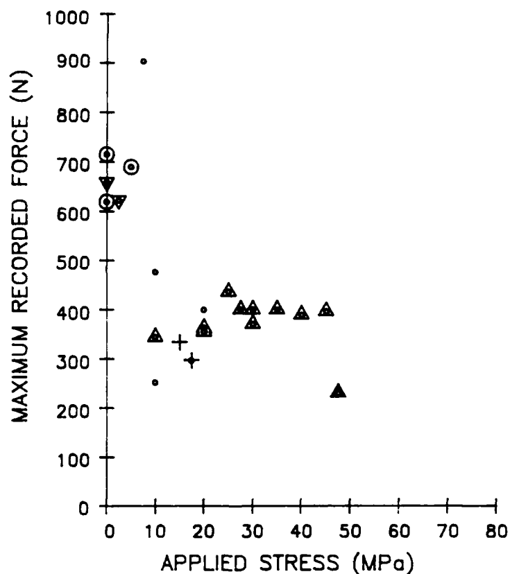
FIGURE 46. Variation of maximum recorded force with applied stress and impact energy for the Carbon / LAS glass-ceramic composite materials.
