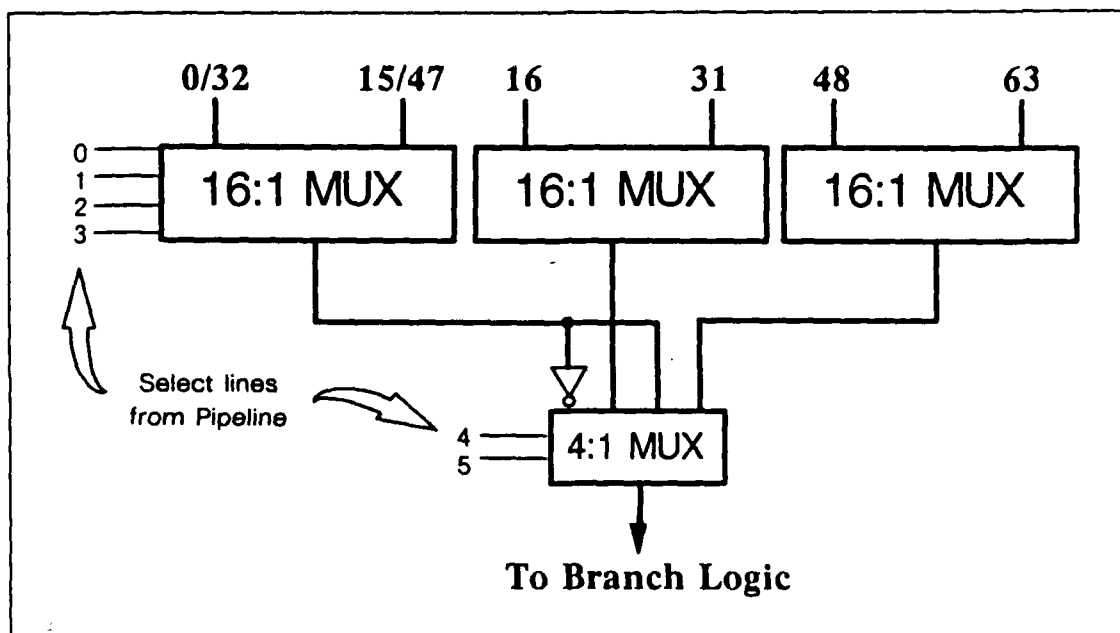
Figure 4.20. Condition Multiplexer.
