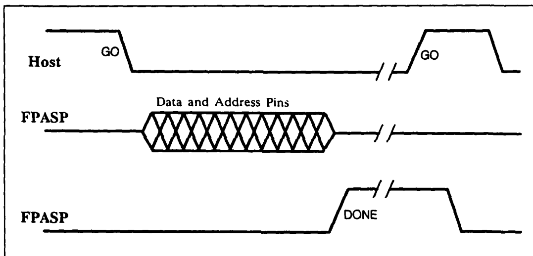
Figure 3.9. Host-FPASP Handshaking.
