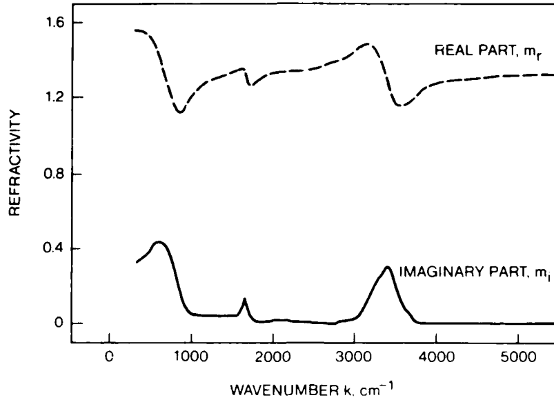
Figure 2. Real and imaginary parts m_r, m_i of refractivity as a function of wavenumber k .
