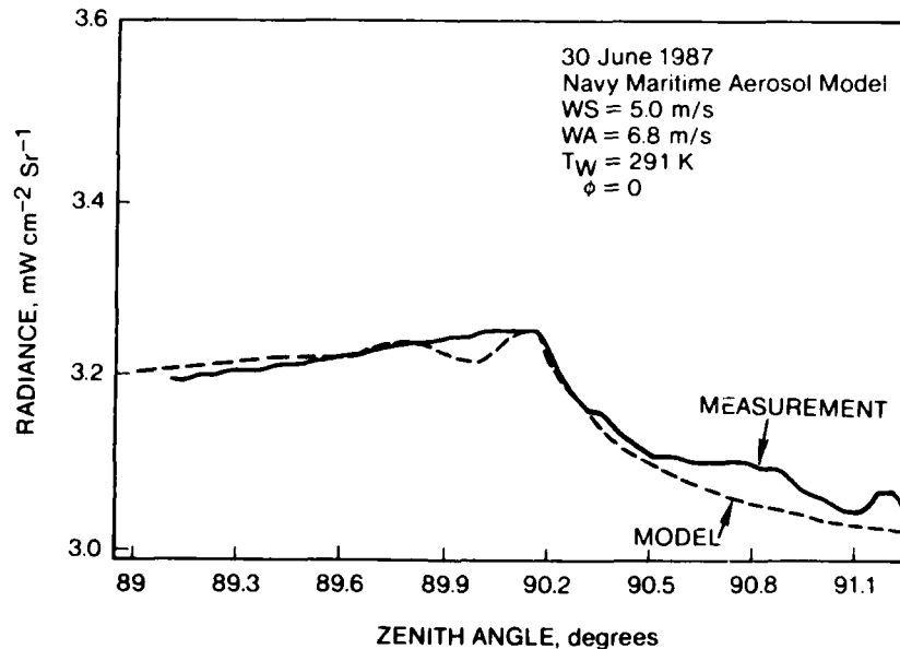
Figure 11. Comparison between measured and calculated radiances for 30 June 1987.
