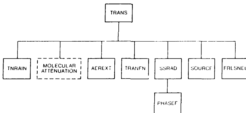
Figure 5. Subroutine FRESNEL is added to the subprogram TRANS.
