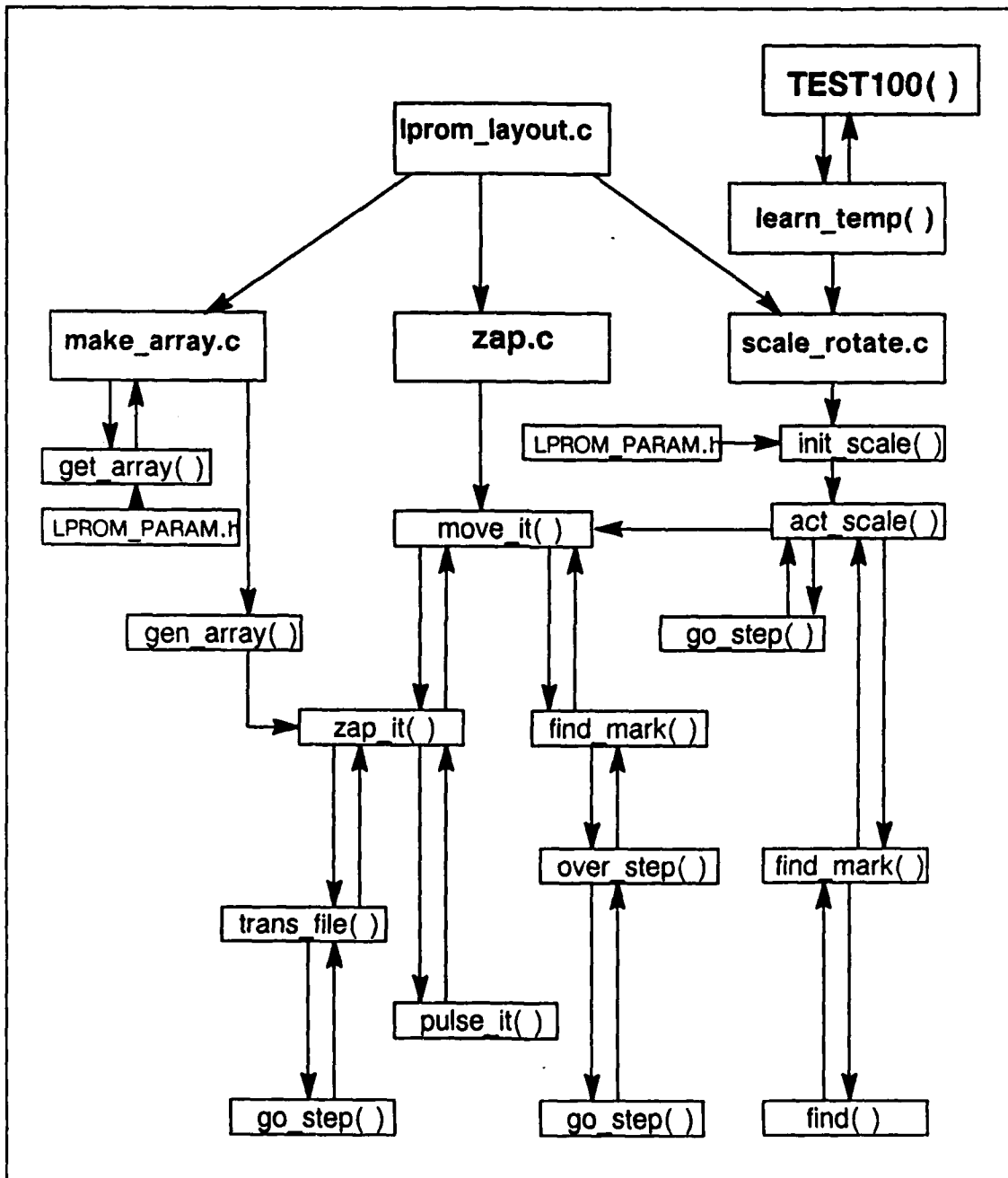
Figure 4.7. Software Subroutines.
