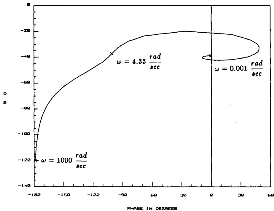
Figure 4.3. Continuous Time Nichols Plot - \beta vs \beta_{cmd}
