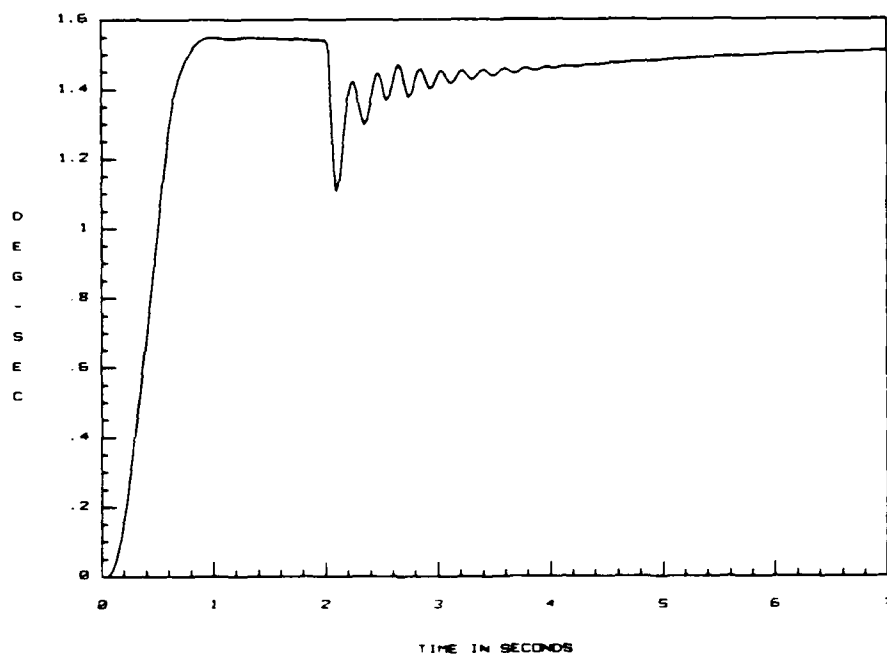
Figure 6.6. r - 45° Banked Turn
