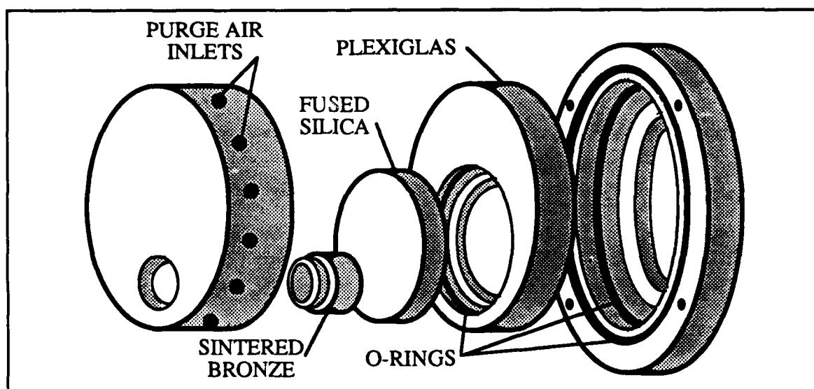
Figure 3.3. Window/Purge Assembly
