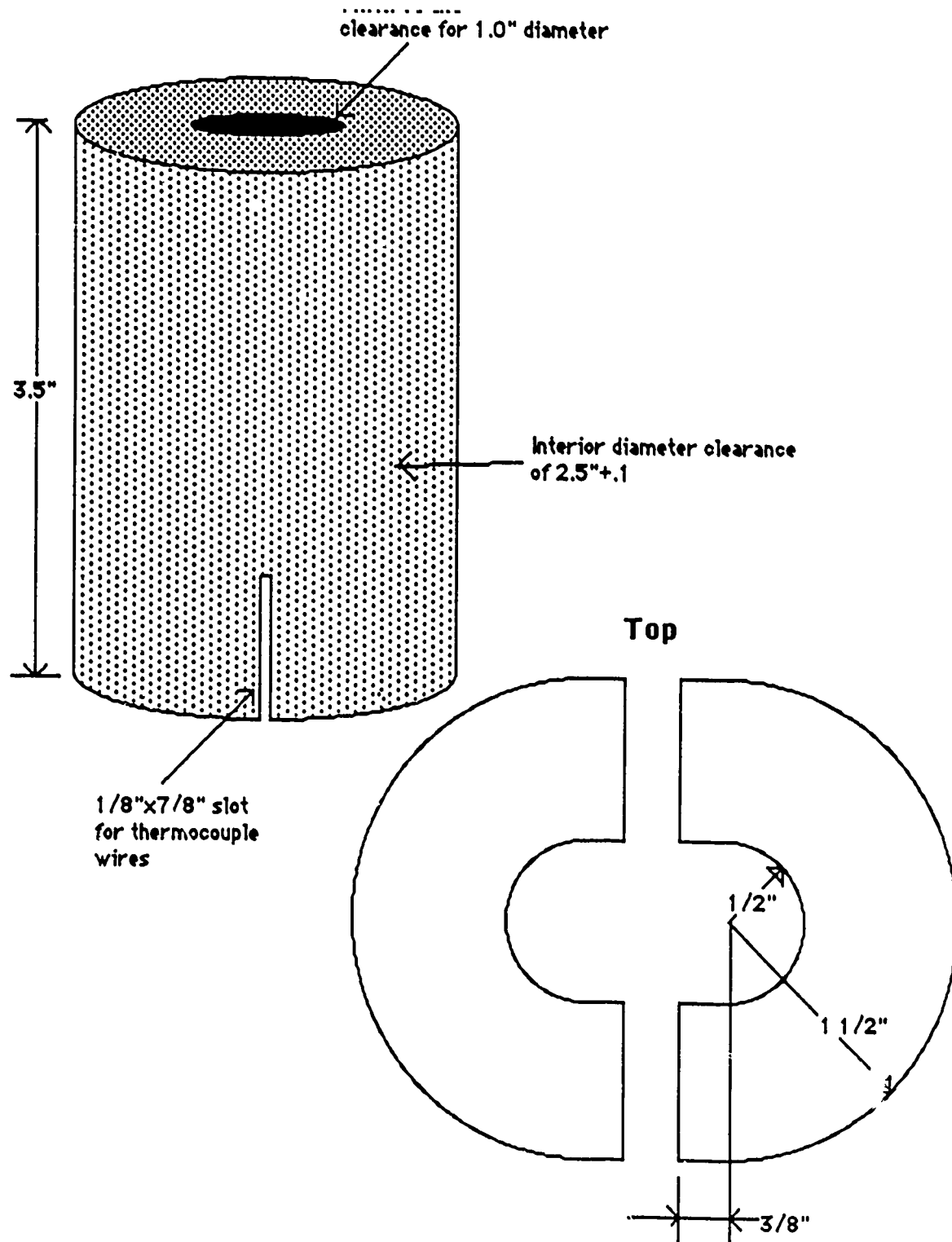
Figure 63. Susceptor
