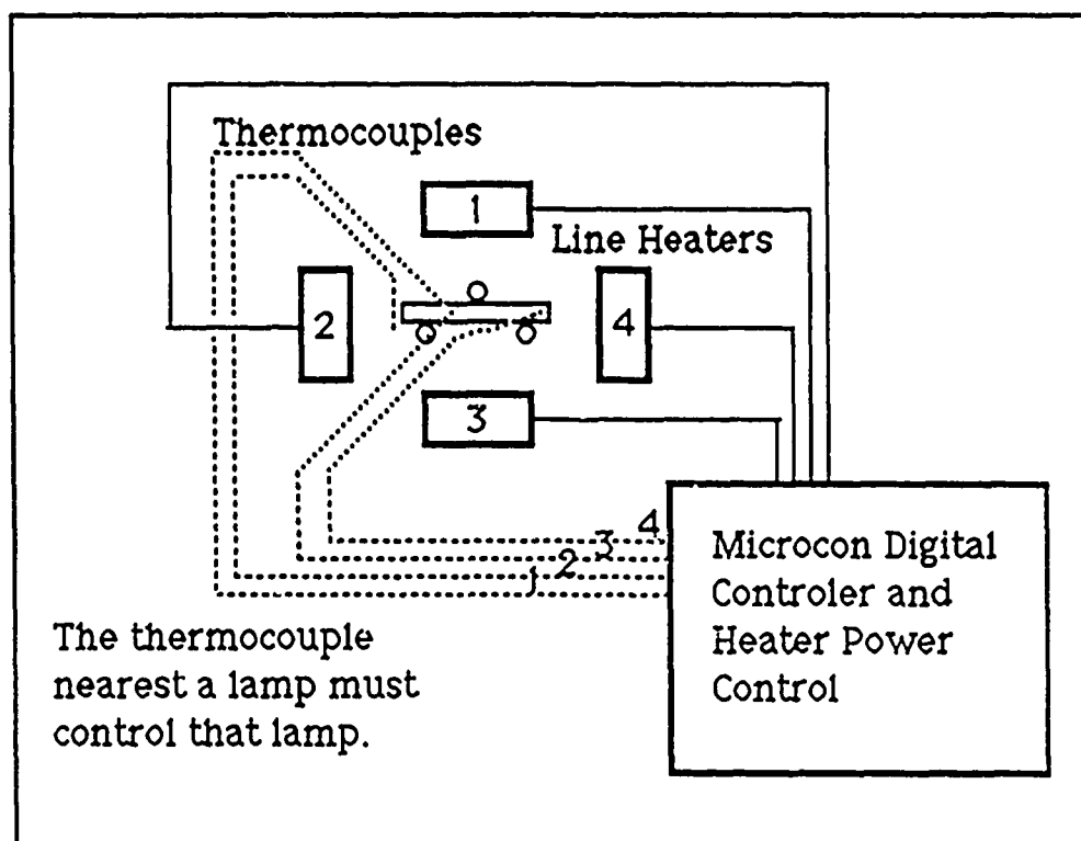
Figure 6. Microcon/Thermocouple Layout
