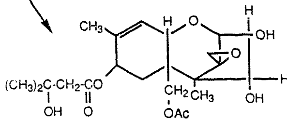
3' HYDROXY HT-2
