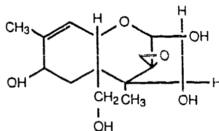
T-2 TETRAOL
