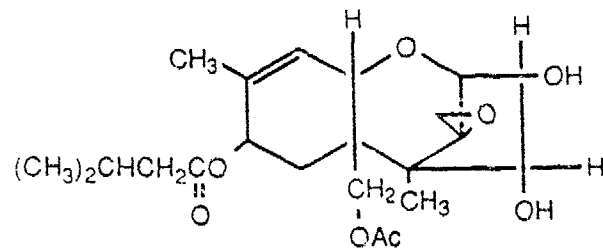
HT-2
