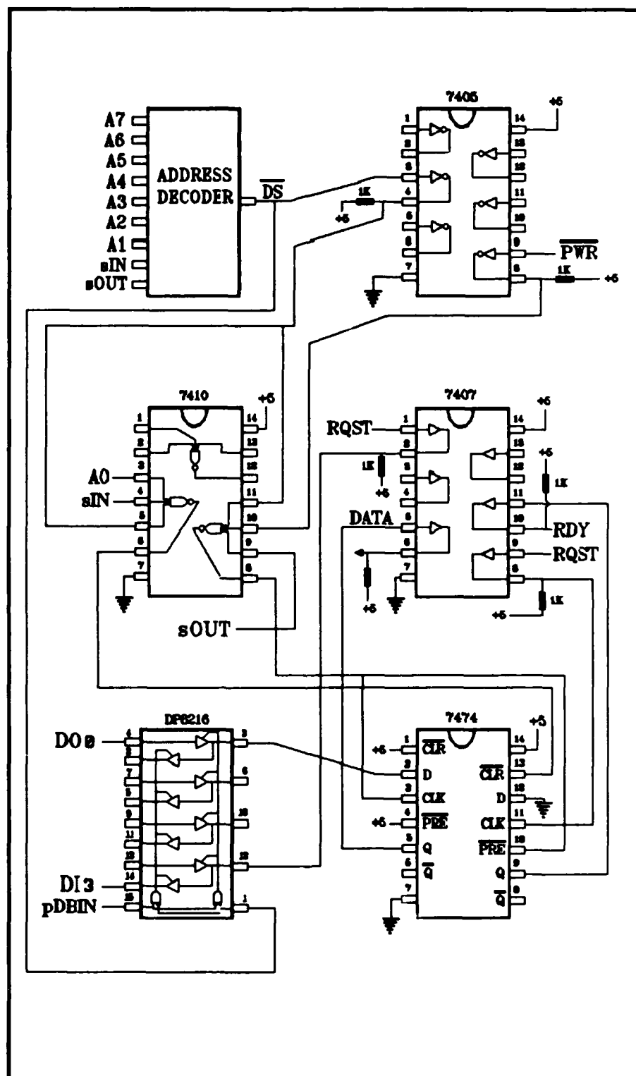
Figure 6 - Output Port
