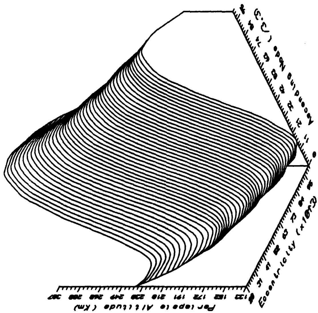
Fig E.3: Perigee Altitude ( i = 1.5 deg)
