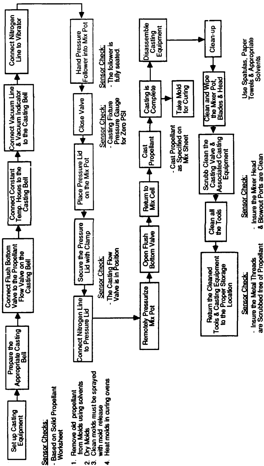
FIGURE 13 CASTING OPERATION
