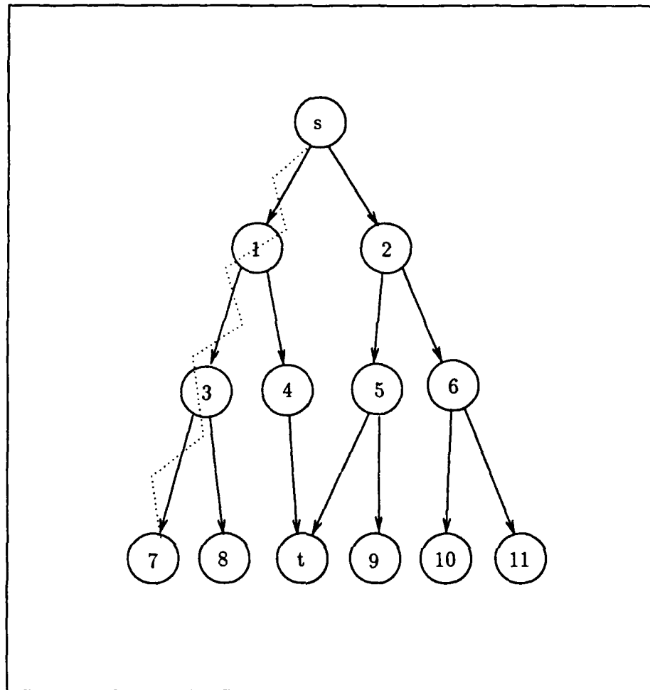
Figure 8. Depth-First Search
