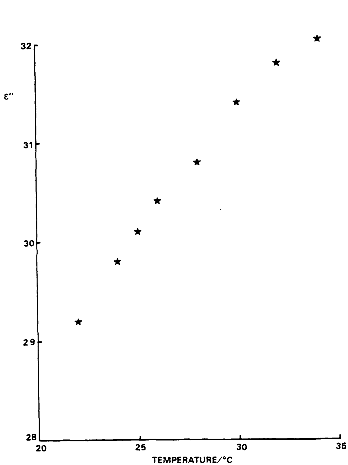
Figure 21. \epsilon'' against temperature for water at 35 GHz.
