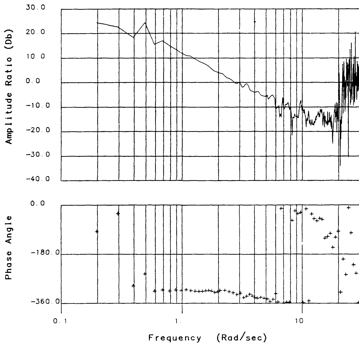
FIG. 8: BODE PLOT: PITCH FLIGHT DIRECTOR/DELTA e '40 KTS)
