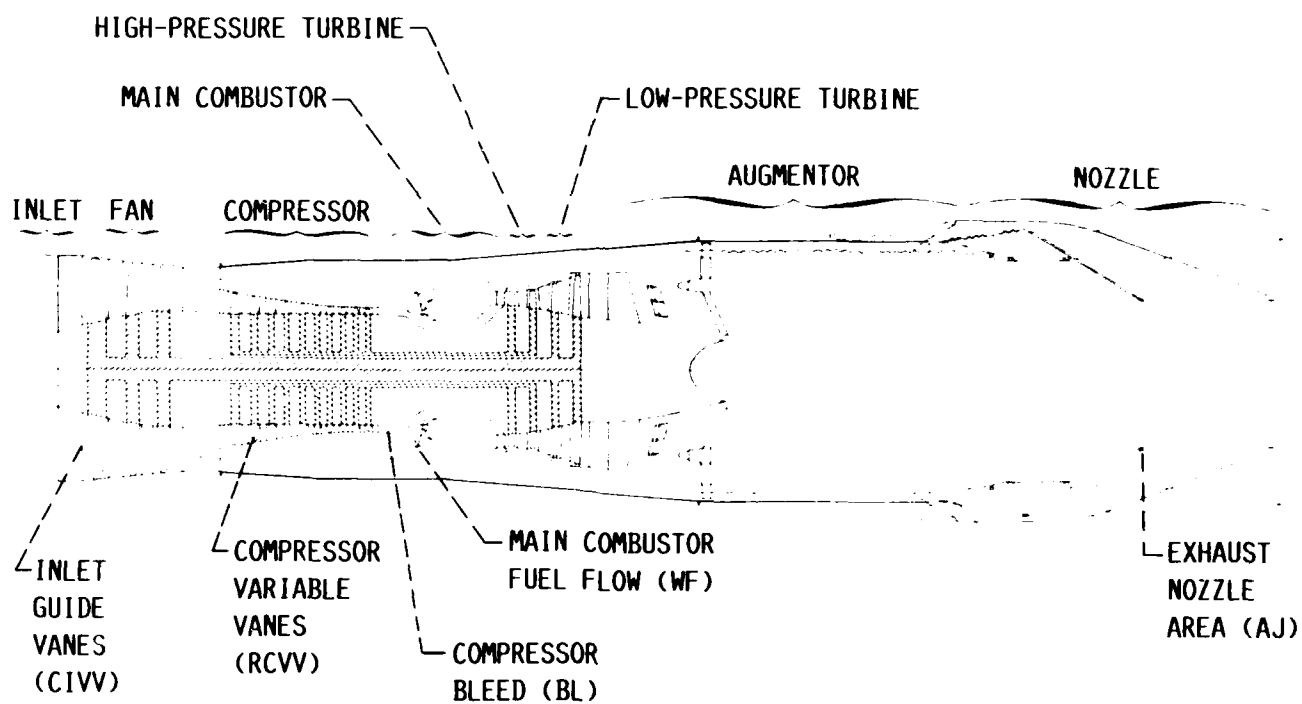
FIGURE 1. - F100 ENGINE INPUTS.
