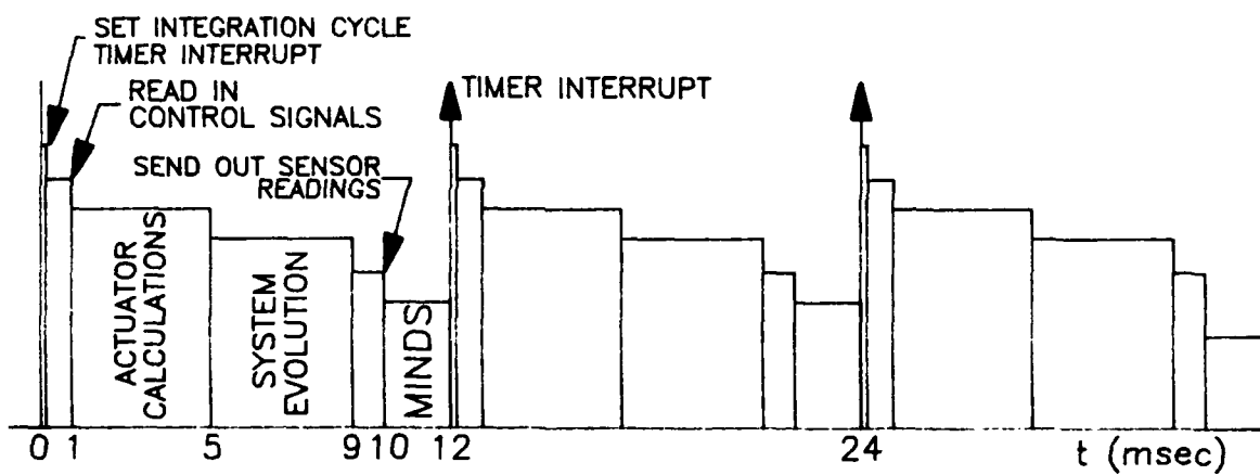
FIGURE 7. - TIMING DIAGRAMS.
