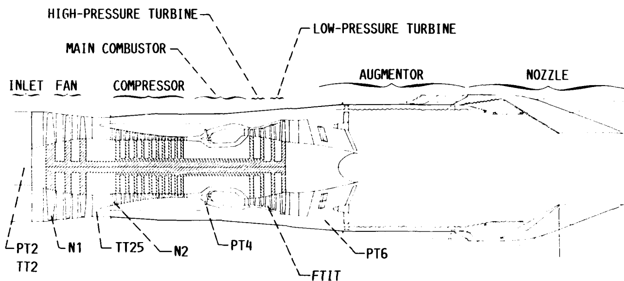
FIGURE 2. - F100 SENSE POINTS.
