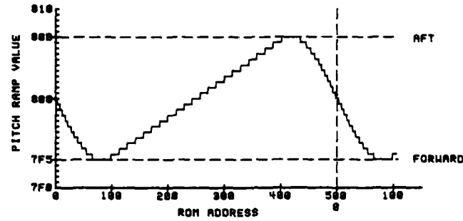
(a) SCAN-MIRROR PITCH WAVE
