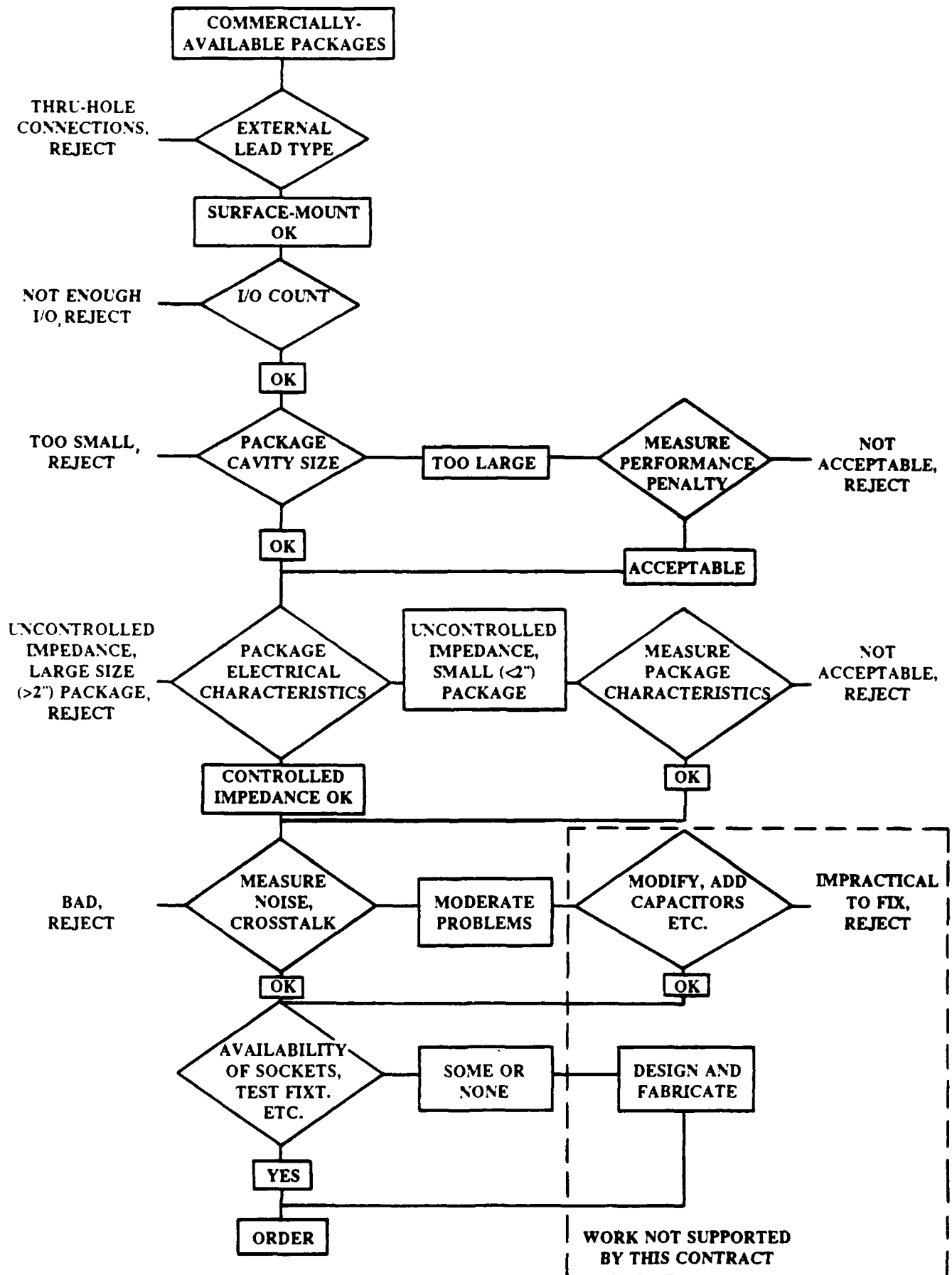
Figure A-13. High Speed Package Selection Process
