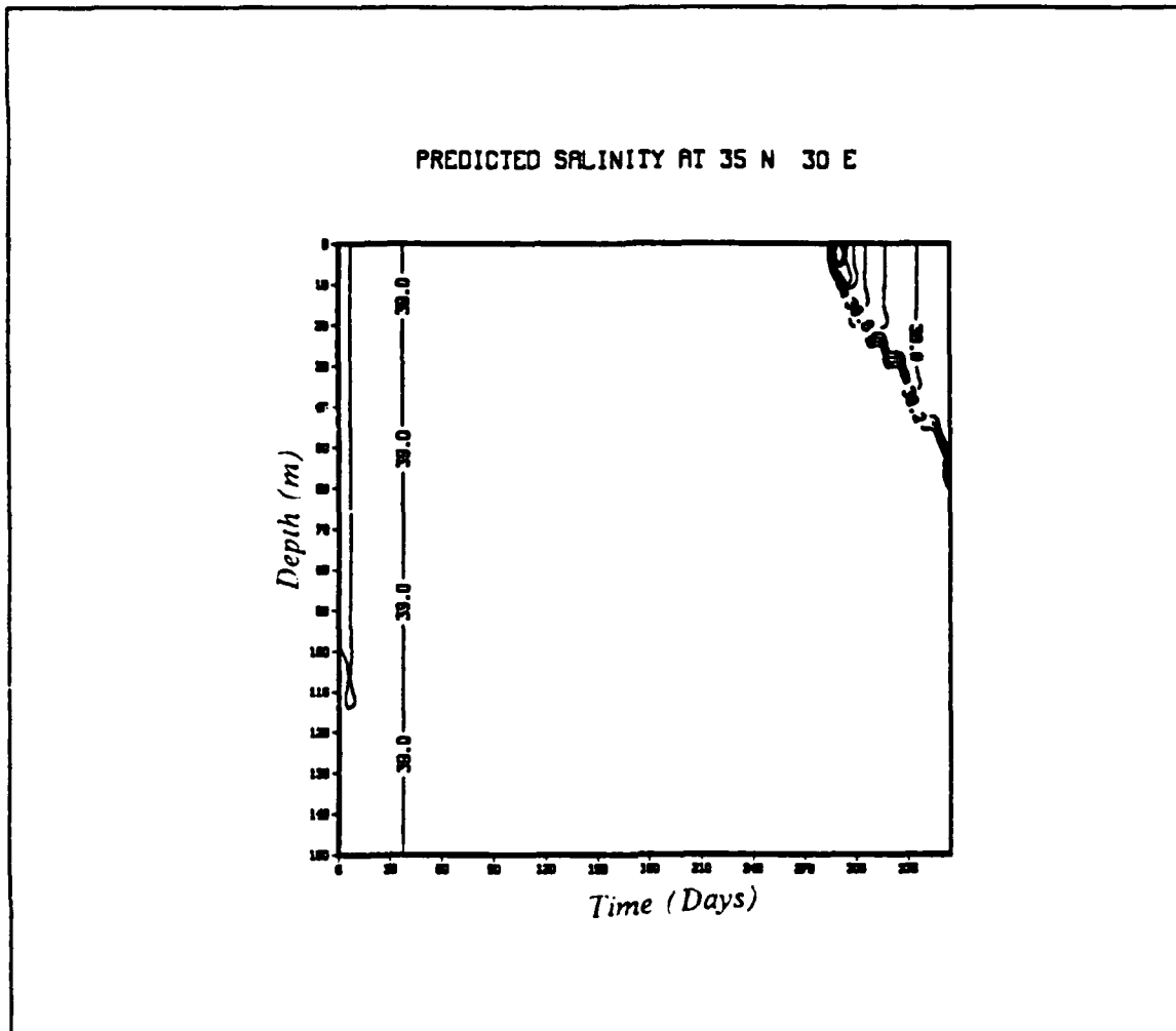
Fig. 19. The Predicted Salinity With Free Convection Only
