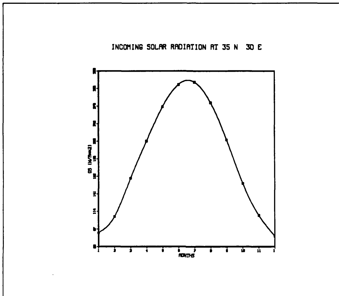
Fig. 32. The Incoming Solar Radiation At 35 ° N 30 ° E
