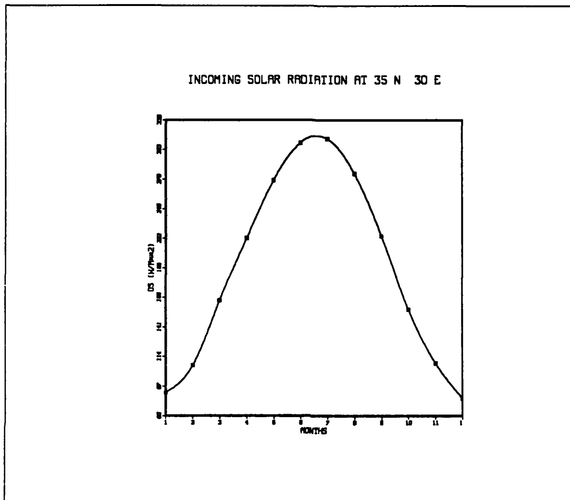
Fig. 5. The Incoming Solar Radiation At 35 ° N 30 ° E
