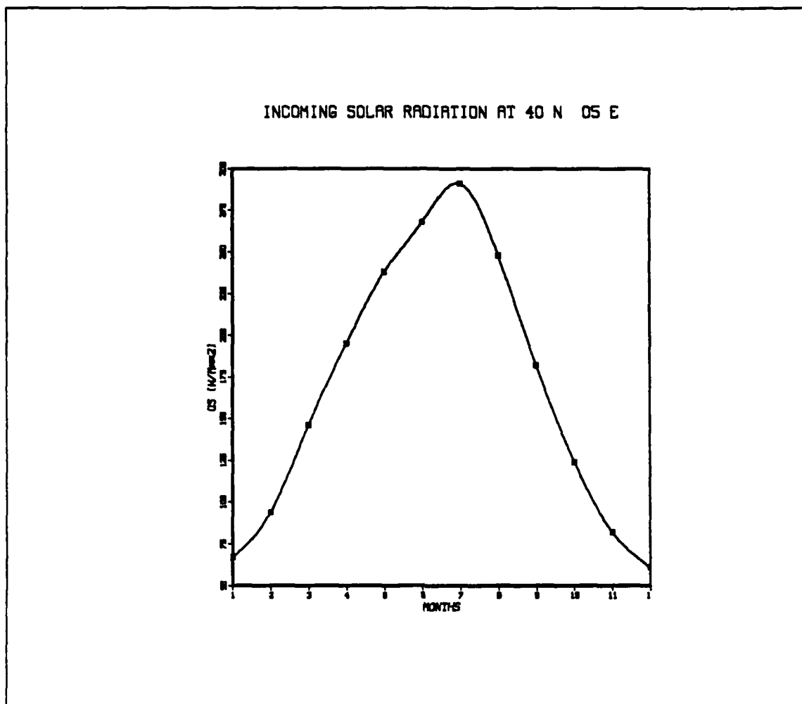
Fig. 3. The Incoming Solar Radiation At 40 ° N 05 ° E
