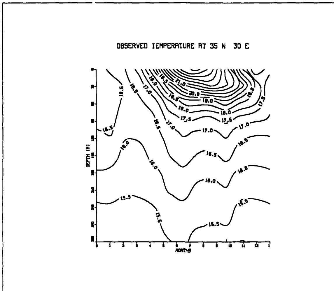
Fig. 11. The Observed Temperature At 35 ° N 30 ° E
