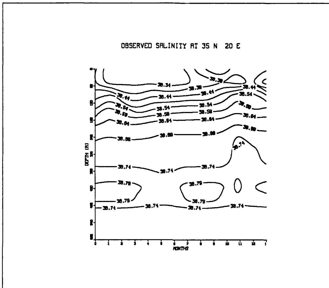
Fig. 16. The Observed Salinity At 35 ° N 20 ° E
