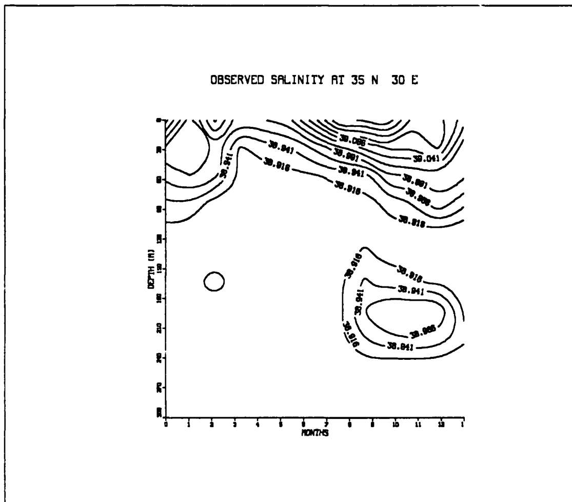
Fig. 14. The Observed Salinity At 35 ° N 30 ° E
