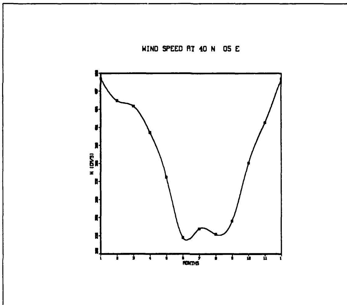
Fig. 8. The Wind Velocity At 40 ° N 05 ° E
