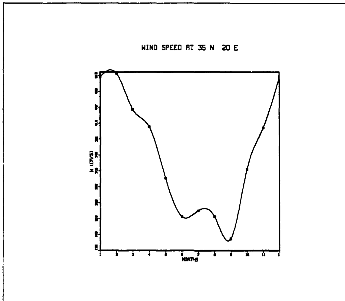
Fig. 9. The Wind Velocity At 35 ° N 20 ° E
