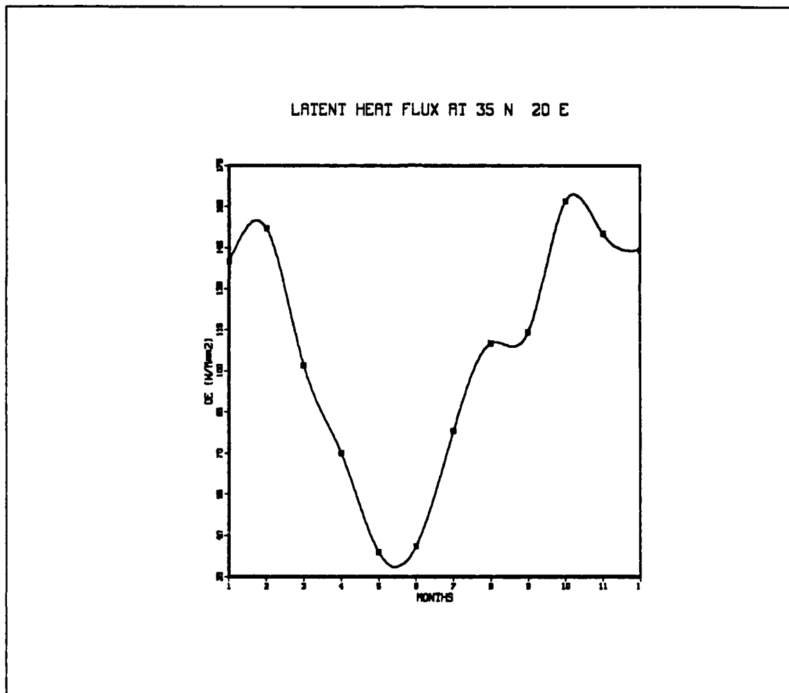
Fig. 2. The Latent Heat Flux At 35 ° N 20 ° E
