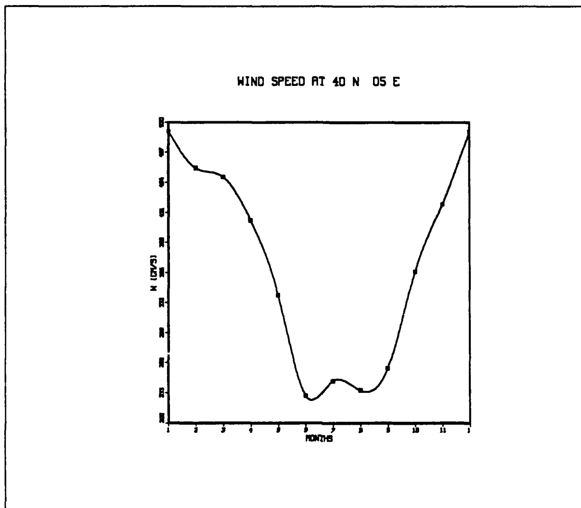
Fig. 34. The Wind Speed At 40 ° N 05 ° E
