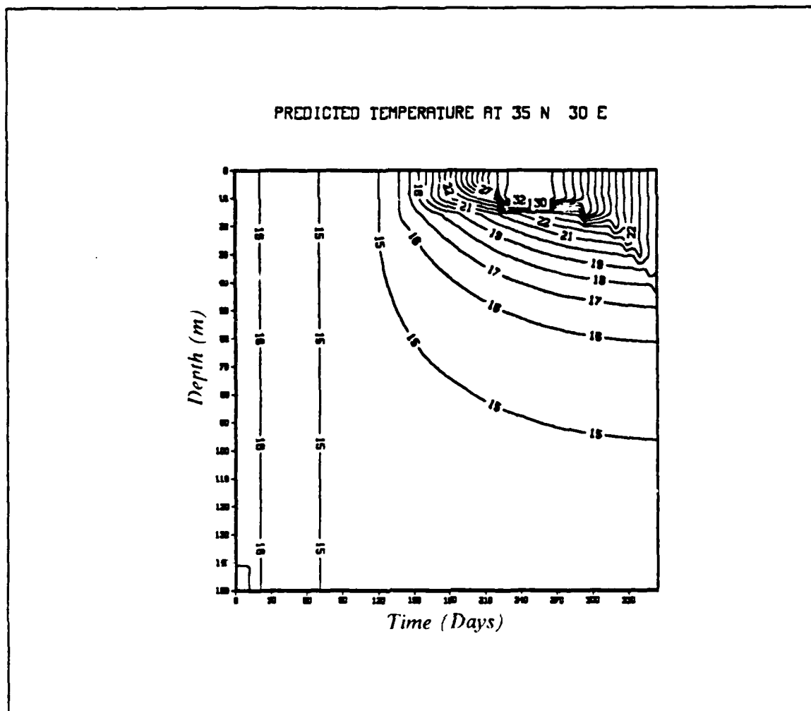
Fig. 25. The Predicted Temperature With Wind And Heat Fluxes Only
