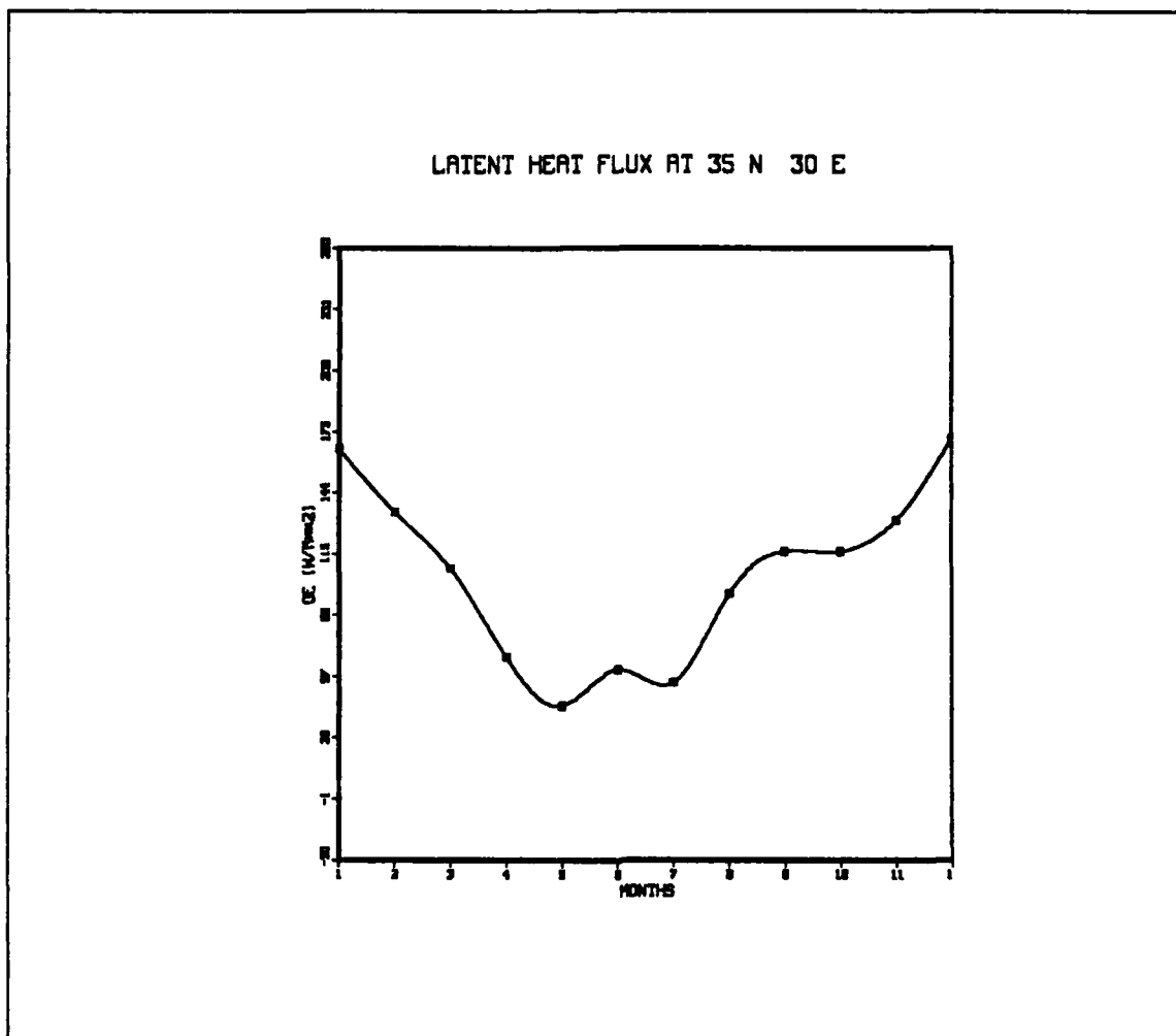
Fig. 33. The Latent Heat Flux At 35 ° N 30 ° E
