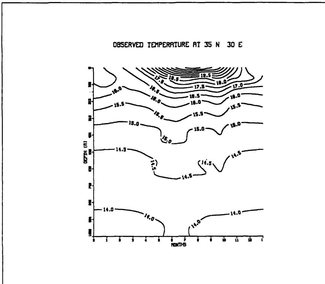
Fig. 12. The Observed Temperature At 35 ° N 30 ° E
