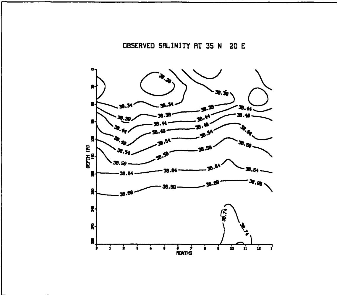
Fig. 15. The Observed Salinity At 35 ° N 20 ° E
