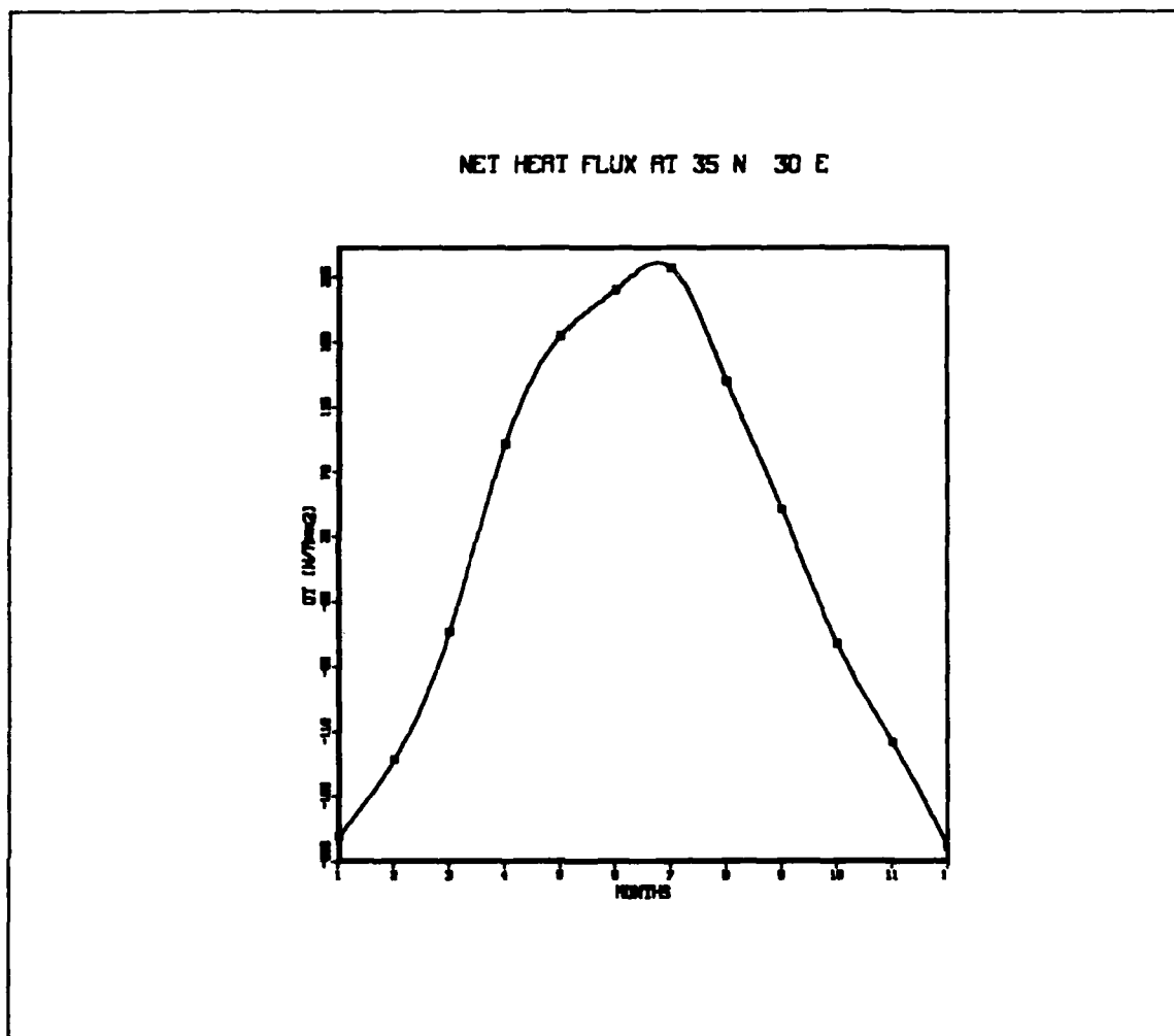
Fig. 7. The Net Heat Flux At 35 ° N 30 ° E
