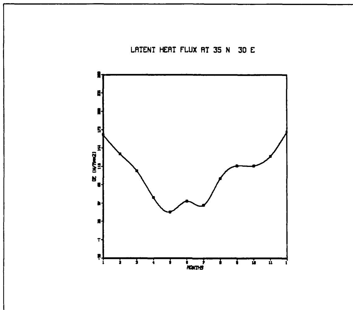
Fig. 6. The Latent Heat Flux At 35 ° N 30 ° E
