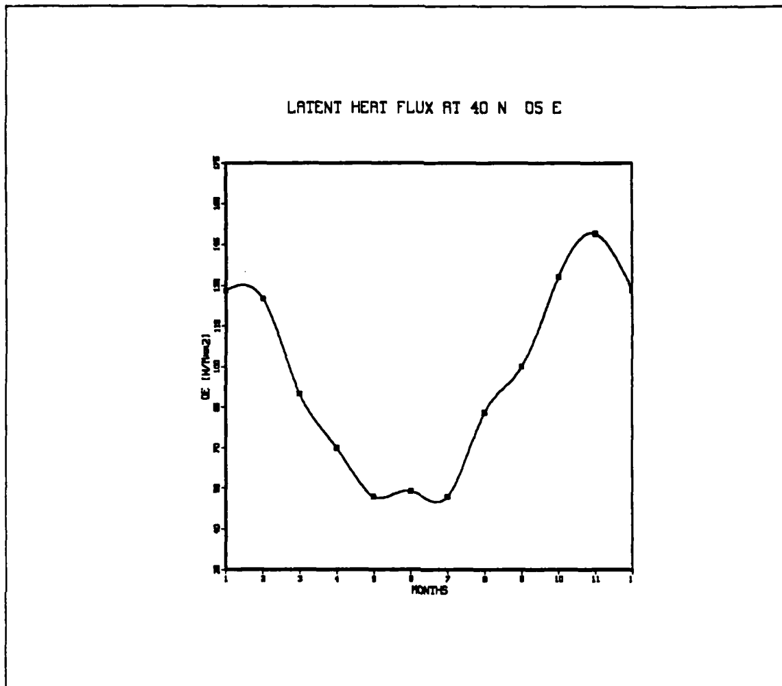
Fig. 1. The Latent Heat Flux At 40 ° N 05 ° E
