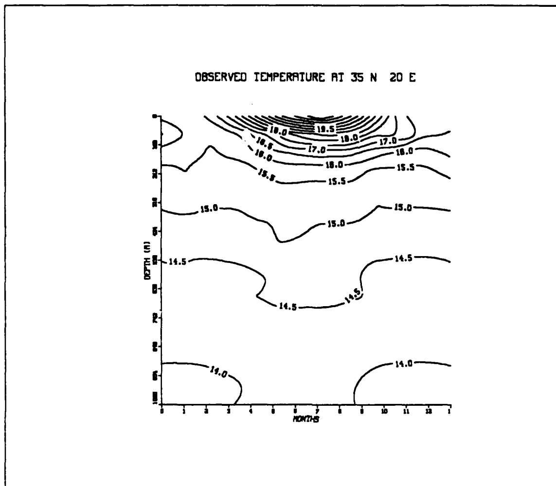
Fig. 13. The Observed Temperature At 35 ° N 20 ° E
