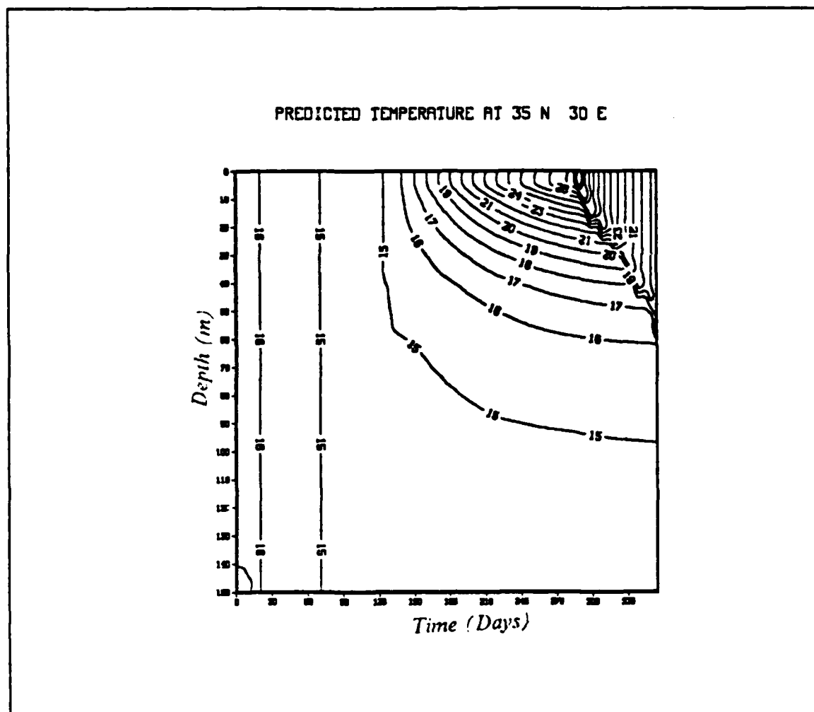
Fig. 20. The Predicted Temperature With Free Convection Only
