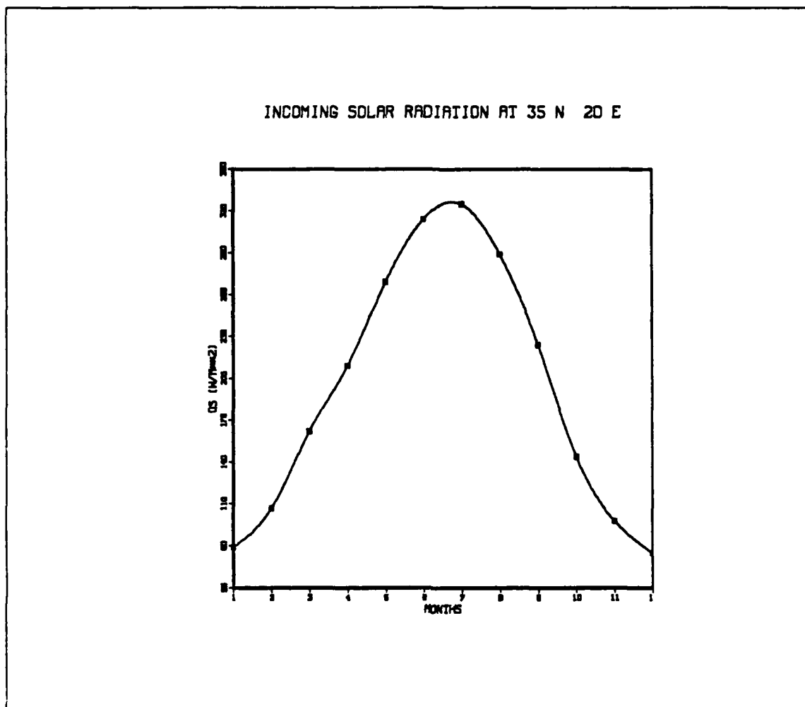
Fig. 4. The Incoming Solar Radiation At 35 ° N 20 ° E
