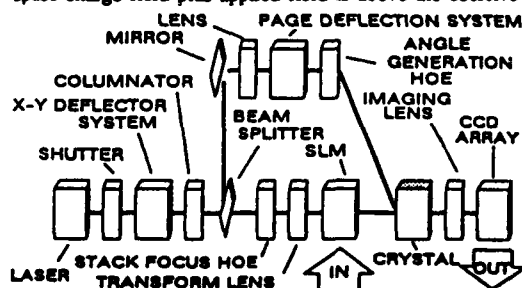
Fig. 1: Optical configuration
