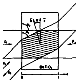
Fig. 1: Principle geometry of four-wave mixing
