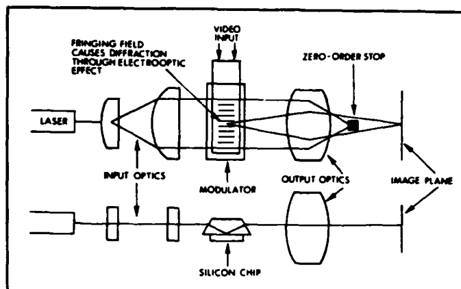
Fig. 8. Readout configuration for the linear array total internal reflection spatial light modulator (after Ref. 9). The top view shows the electrode structure at the interface between the silicon chip (with associated drive circuitry) and the proximity-coupled electrooptic crystal. The total internal reflection at the interface is shown in the side view (bottom half of the diagram).
