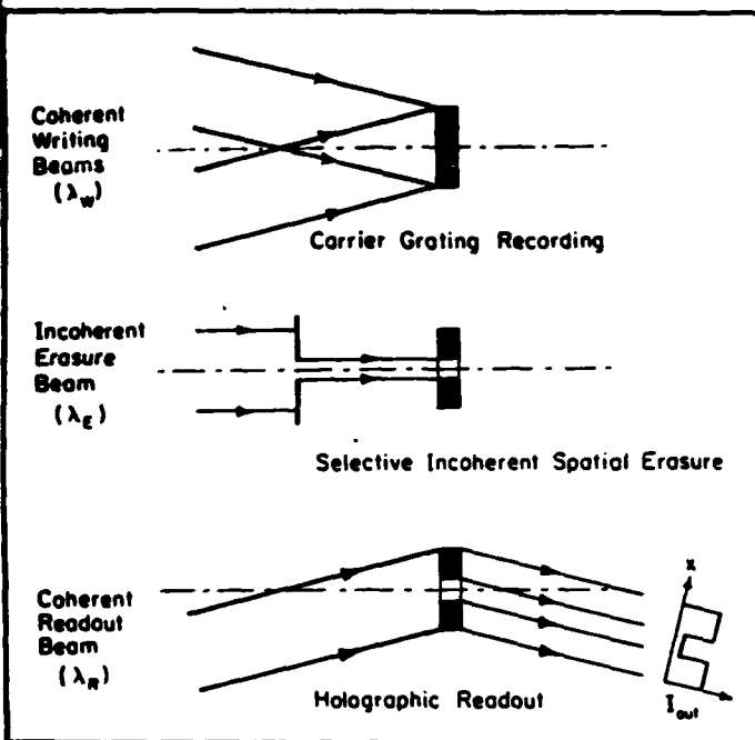
Fig. 14. Schematic diagram of the selective grating erasure process in the photorefractive incoherent-to-coherent optical converter (PICOC).
