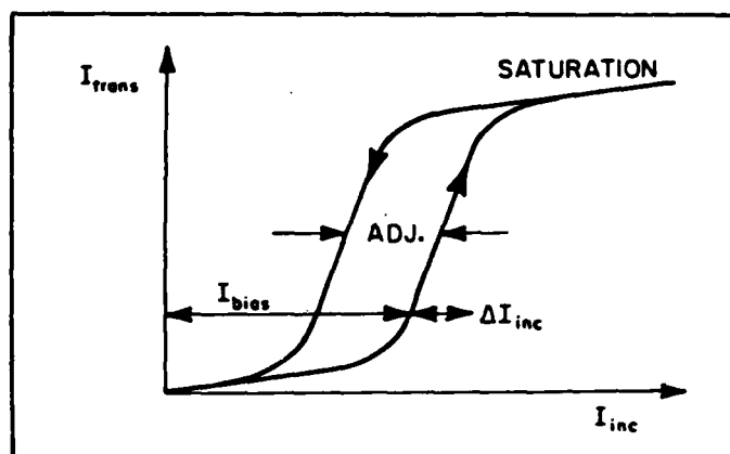
Fig. 19. Schematic illustration of the hysteresis and saturation effects characteristic of optical bistability.
