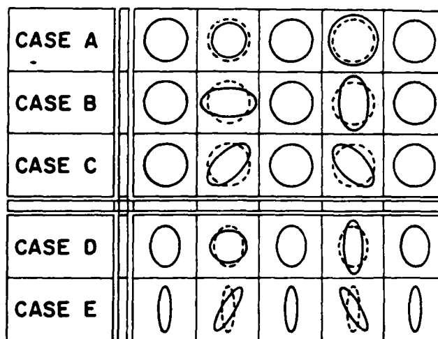
Fig. 6. Categories of birefringent phase gratings, in terms of the periodic spatial evolution of the index ellipsoid. The evolution is shown over one full period of the grating wavelength in the medium. Case A corresponds to an isotropic phase grating; cases B, C, and D correspond to different gratings with fixed principal axes and varying birefringence; case E corresponds to a grating with fixed birefringence and varying principal axes. Cases A, B, and C reside in an isotropic medium, while cases D and E reside in a medium with inherent optical anisotropy.
