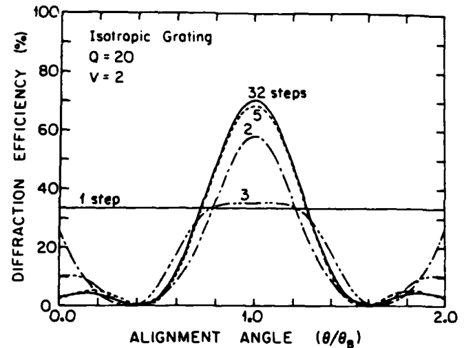
Fig. 13. Angular alignment sensitivity of a typical isotropic phase grating, showing the convergence of the optical beam propagation method to the desired solution for increasing numbers of computational steps.
