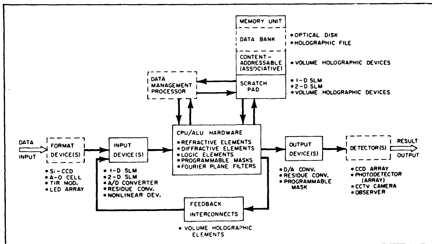
Fig. 1. Schematic diagram of the elements of a generalized optical processor or computer.
