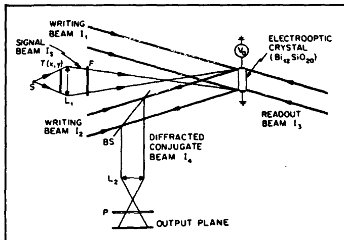
Fig. 16. Experimental arrangement for the demonstration of the simultaneous erasure/writing mode of the photorefractive incoherent-to-coherent optical converter (after Ref. 24). The transparency T(x,y) is imaged by lens L_1 and incoherent source S through spectral filter F onto the surface of the photorefractive device. A retroreflected readout beam derived from the incident writing beam I_1 generates a coherent replica of the transparency in the output plane through lens L_2 and polarizer P .
