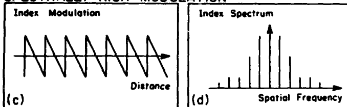
Fig. 7. Schematic diagram of spectrally pure and spectrally rich index perturbation profiles, and their concomitant spatial frequency spectra. Most phase grating analyses typically assume a sinusoidal perturbation. This leads to a simplified coupling of the diffraction orders in which only nearest neighboring orders interact. A more general index perturbation profile has a more intricate spatial frequency spectrum, with a consequently more intricate interaction of non-neighboring diffraction orders. This greater coupling complexity induces significantly greater computation times for numerical integration algorithms such as the Runge-Kutta.
