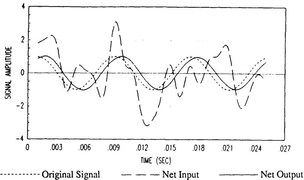
Figure 27. Test 2 - Network Behavior with 124 Hz Experimental Input Signal.
