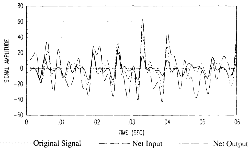
Figure 76. Test 11 - Network Behavior with 1 kHz Speech and High Noise.
