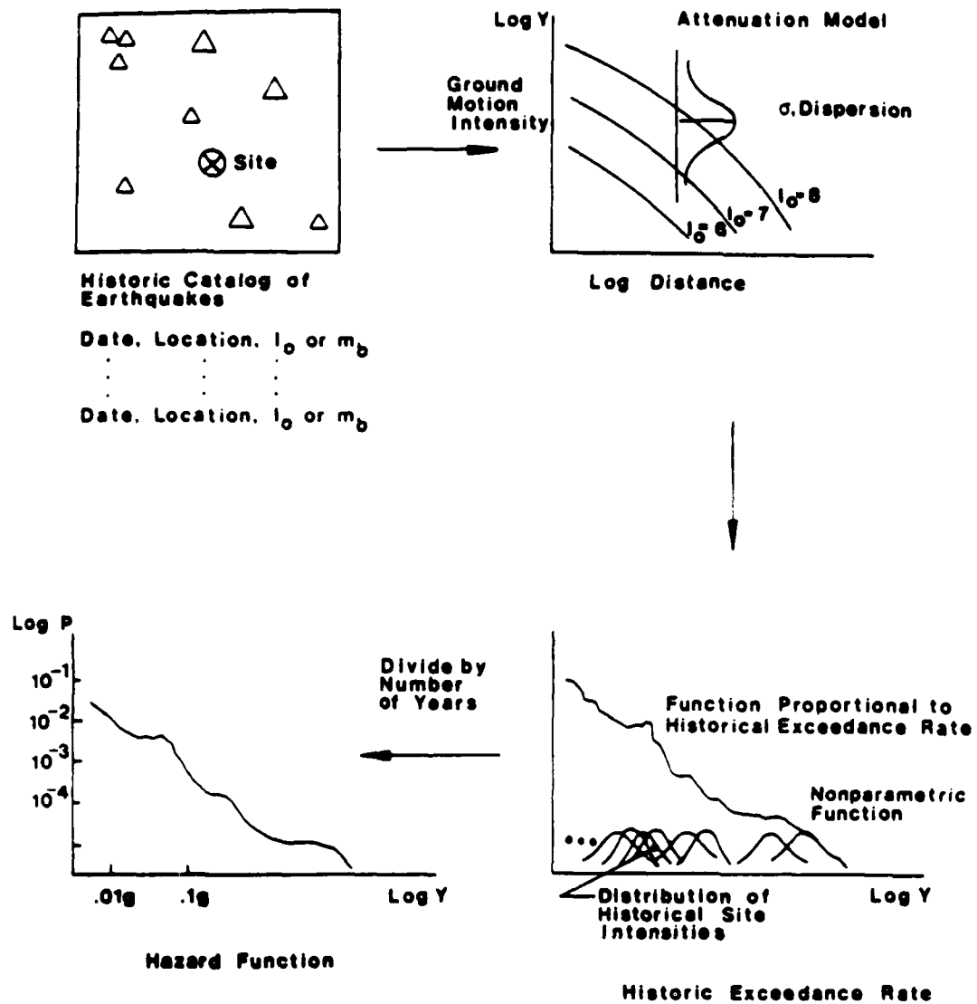
FIGURE 2.6 Steps involved in the (nonparametric) historic method. (Veneziano et al., 1984). Reprinted by permission from the Electric Power Research Institute.
