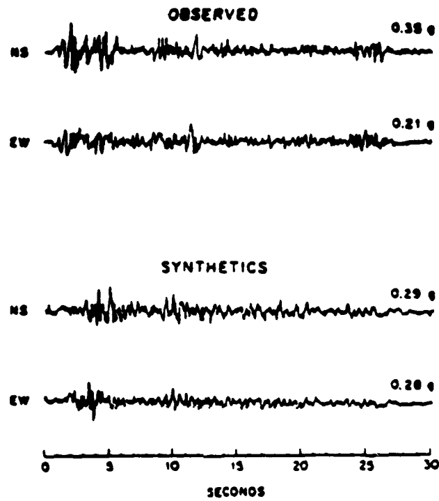
FIGURE 6.5 1940 Imperial Valley earthquake. Observed and simulated acceleration records at El Centro station (Munguia and Brune, 1984).
