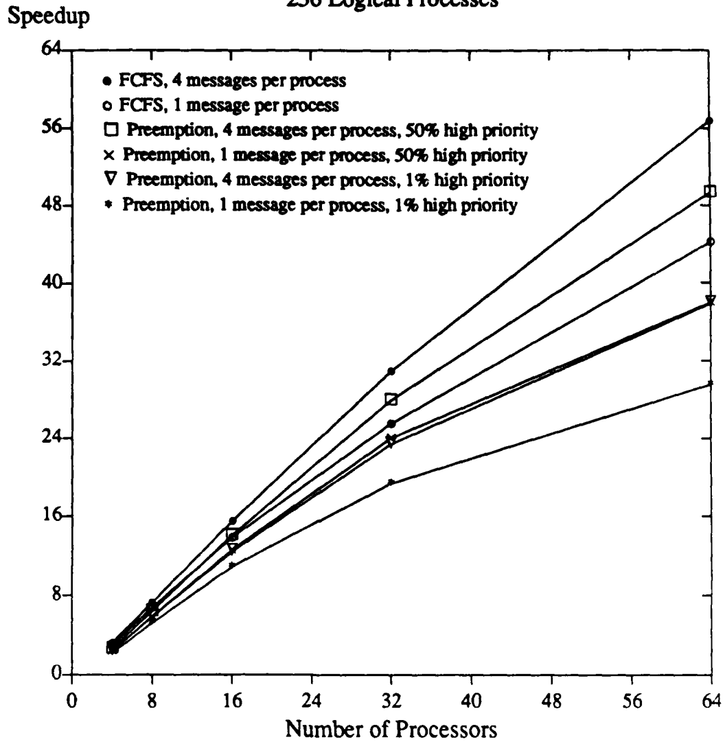
Figure 8. Speedup of 256 process hypercube simulator.
