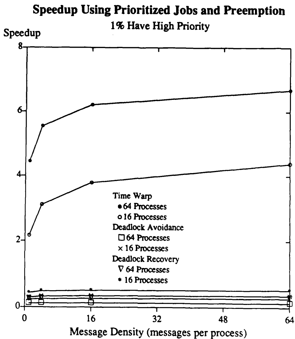
Figure 5. (b) One percent of all jobs have high priority.
