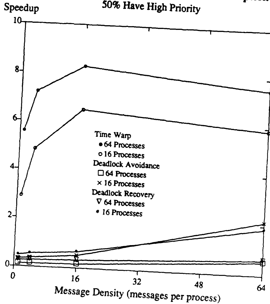
Figure 5. Speedup curve for queuing network simulator with prioritized jobs and preemption. (a) Half of all jobs have high priority.
