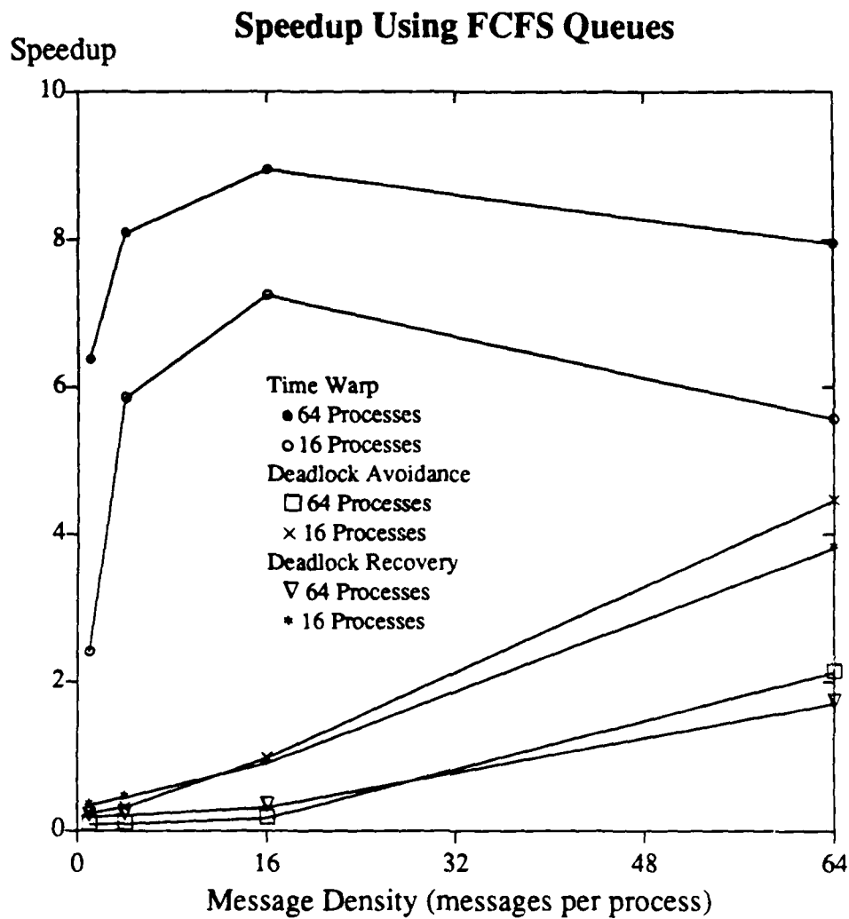
Figure 2. Speedup of the queuing network simulator using first-come-first-serve queues. Time Warp performance degrades for large message densities because the time required for event list insertions dominates (the conservative algorithms use FIFO queues so they do not suffer from this problem).
