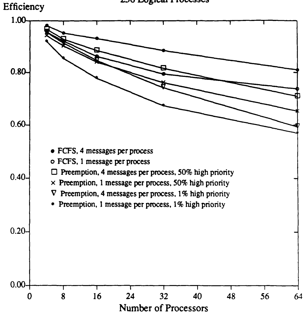
Figure 9. Efficiency of Time Warp simulations for 256 process hypercube.
