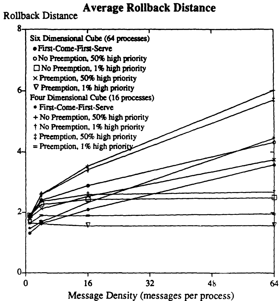
Figure 7. Average rollback distance for queuing network simulations (number of processed events rolled back per rollback).
