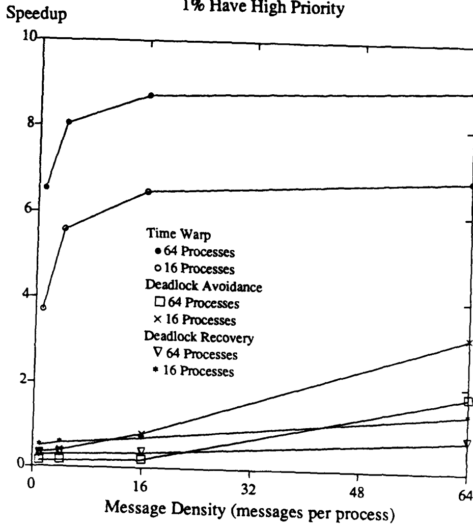
Figure 4. (b) One percent of all jobs have high priority.
