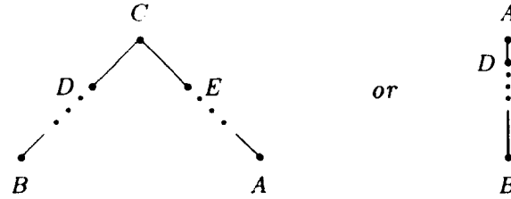
Figure 3.6: Lock propagation
