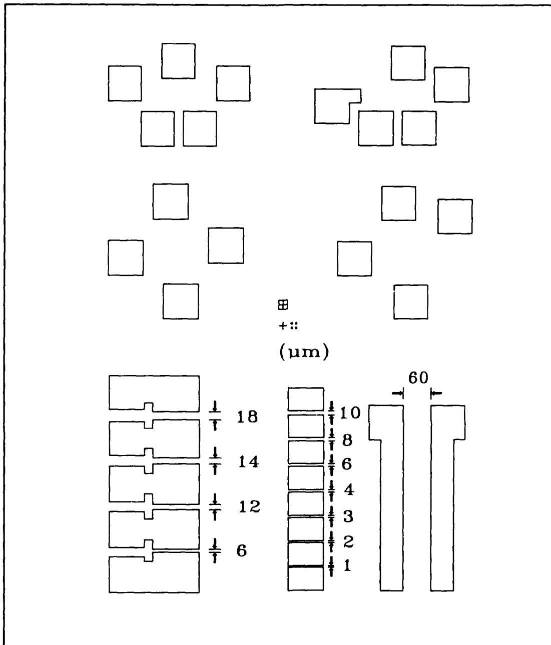
Figure 22. Source and Drain Contact Mask Pattern
