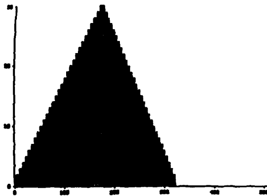
Figure 3: (Factorial 30): Invocation Tree Profile- Parallel
