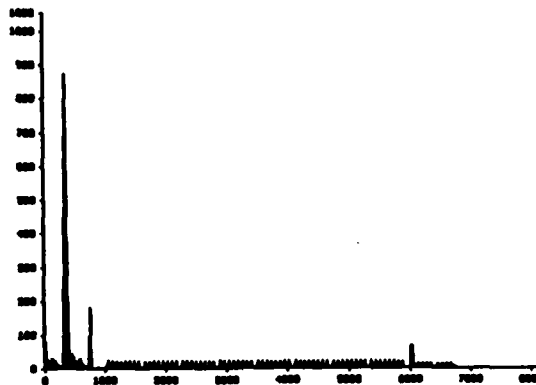
Figure 23: DNA Sequence Matching: alu operations profile- futures
