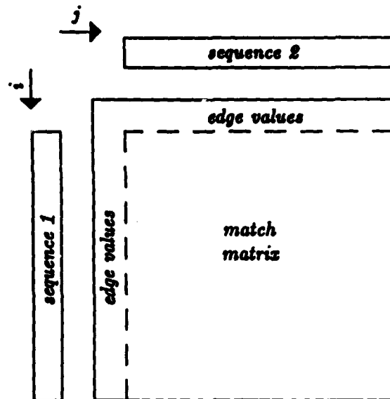
Figure 12: Alignment of sequences with match matrix
