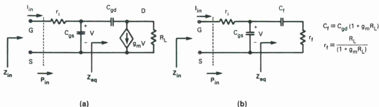
Figure 3-4. Device input model extended to include feedback capacitance: (a) original and (b) equivalent models.
