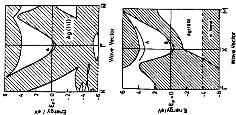
Fig. 1: Surface band structures of Ag(111) and Ag(100). A, B: surface states.
