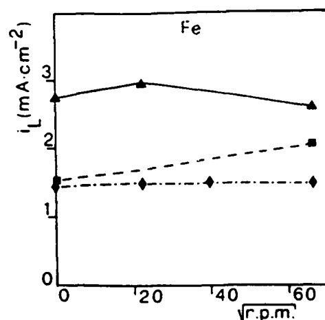
Fig. 2 - i_L in 0.1 N solutions of weak acids: \blacktriangle HF; \blacksquare HCOOH \blacklozenge CH 3 COOH
