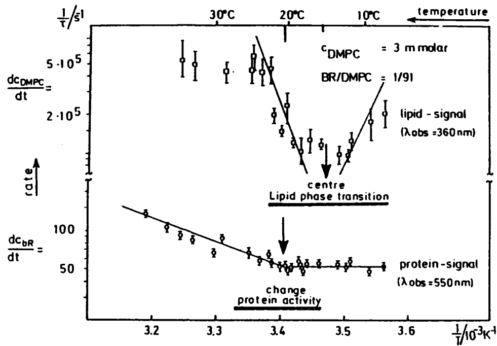
Fig. 2: Arrhenius dependence of the lipid relaxation \tau_{DMPC} and the bR relaxation \tau_{bR}
