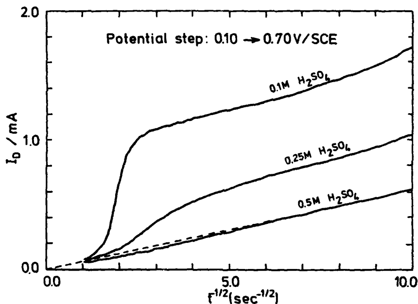
Figure 3: Cottrell-type representation of chronoamperometric current ( I_D ) transients observed with electrolytes of indicated \text{H}_2\text{SO}_4 concentration and 1 mM \text{Fe}^{2+} . Electrode area 0.27 \text{ cm}^2 .
