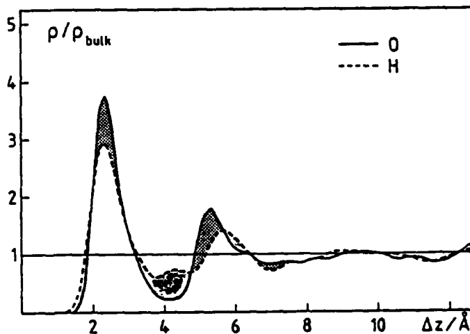
Figure 2: Normalized oxygen and hydrogen density profiles \rho^{(1)}(z)/\rho_{\text{bulk}} for a simulation of 305 water molecules between two (100) faces of a face centered cubic platinum crystal.
