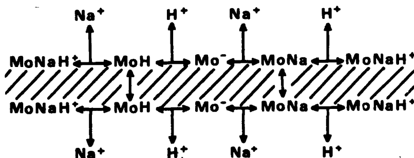
Scheme I. The reaction steps involved in pulse protonation of a membrane impregnated with monensin.
