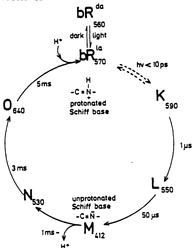
Fig. 1: Schematic Photocycle of Bacteriorhodopsin (bR) including averages of absorption maxima and lifetimes of intermediate states
