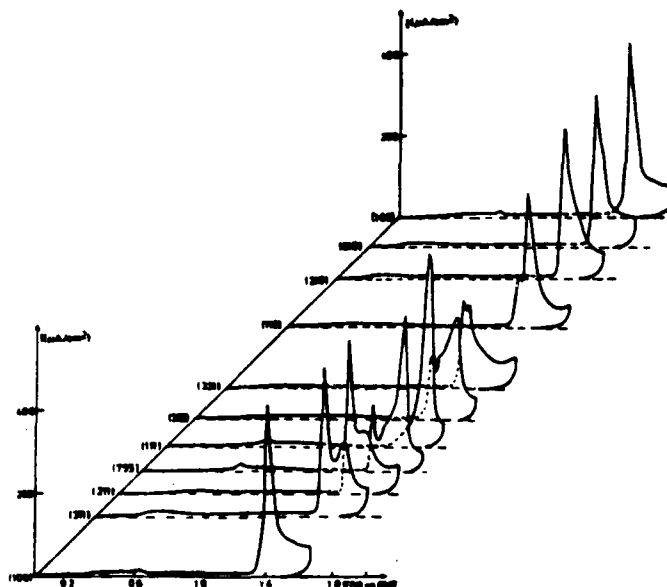
Fig. 1. Oxide formation on Au(hkl) in 0.05M H_2SO_4 ; sweep rate 50 \text{ mVs}^{-1} .
