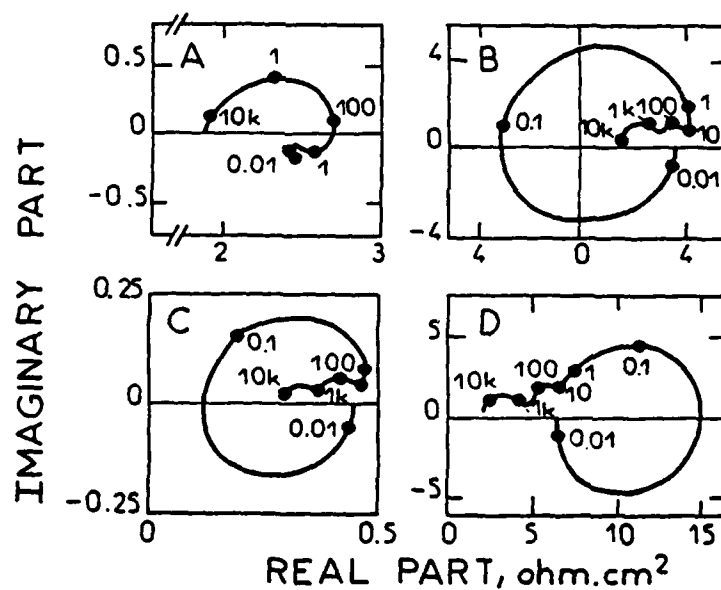
Figure 2 : Impedance diagram. A to D corresponds the point marked on Fig. 1 by the same letter.
