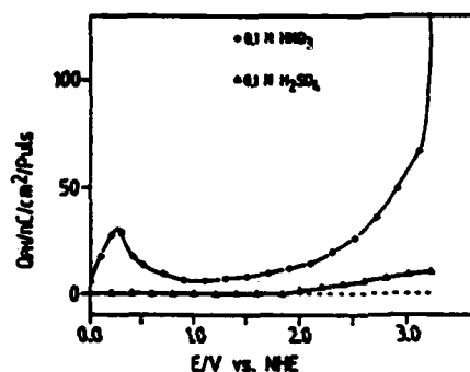
Fig. 1 Photocurrent-potential dependence of passivated Ti electrode (3.2 V \text{TiO}_2 layer); light intensity I = 0.33 \text{ mW/pulse} ; \lambda = 500 \text{ nm} , \phi = 0.1 \text{ N HNO}_3 , \Delta = 0.1 \text{ N H}_2\text{SO}_4 .
