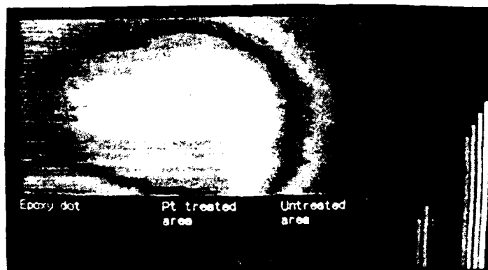
Fig. 3 A computer generated picture showing the effect of Pt treatment on the photocurrent. A drop of 20 mM \text{H}_2\text{PtCl}_4 was applied onto the electrode for 5 min, which was then rinsed with water. The photocurrent is much higher at the area which was covered with the Pt solution compared to the untreated area. The scanned area is 400 \mu\text{m} in Y-direction and 1000 \mu\text{m} in X-direction.
