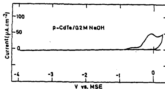
Fig. 2 Dark current versus potential characteristic of p-CdTe in basic electrolyte.
