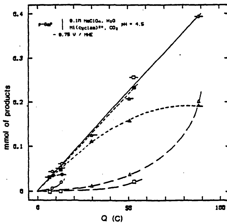
Figure 2 Plot of the quantities of CO and H 2 produced vs electric charge passed through the semiconductor electrode: CO + H 2 : —○— : —△— : —●— (———) CO : —□— : —▲— : —●— (---) H 2 : —□— : —△— : —●— (---) — quantities of Ni(cyclam) 2+ : —□— : 600 μmol; —△— : 70 μmol; —●— : 7 μmol
