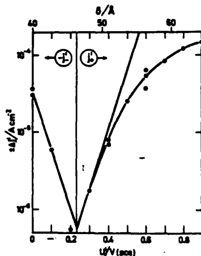
Fig. 1. Stationary Tafel data ( \text{pH} = 3.0 , j_f = 2 \mu\text{Acm}^{-2} , (\text{ox}) = (\text{red}) = 0.01 \text{ M} and quasi-steady passive film thickness at each potential as noted by top scale).
