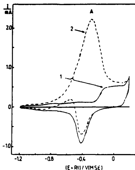
Figure 1 Voltammograms of Au-NaY zeolite electrode. 1) N_2 flow, 2) ethanol vapors, p_2 11.5 Torr. Surface area : geometrical 1.31 \text{ cm}^2 , "true" 6.47 \text{ cm}^2 . Sweep rate 50 \text{ mV s}^{-1} , 1M \text{ NaOH} , 25^\circ\text{C} .
