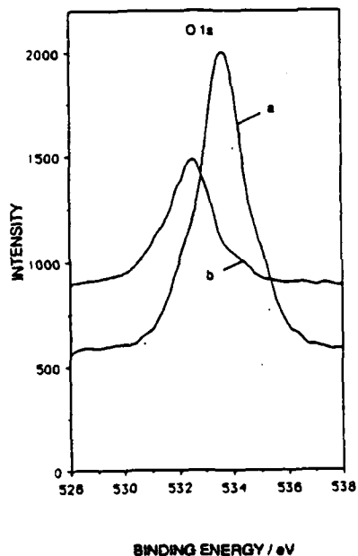
Fig. 3: XPS data for the O 1s line for a) a thick and b) a thin passivating layer on a-Si:H with Mg K \alpha radiation at normal emission. The thickness for a) is about 10 times higher than for b).
