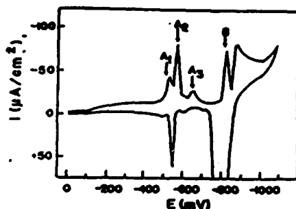
Figure 2. CV for thallium deposition on a Ag(111) electrode from 1.0 mM \text{Ti}_2\text{SO}_4 / 0.25 M \text{Na}_2\text{SO}_4 / pH = 3.0. 10 mV/s.
