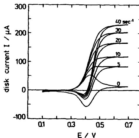
Figure 1: Pseudo-stationary \text{Fe}^{2+} oxidation at a rotated disk electrode coated with a 1.2 \mu\text{m} "Nafion" film. Electrolyte: 1 \text{ mM FeSO}_4 + 0.1 \text{ M H}_2\text{SO}_4 . Electrode area: 0.27 \text{ cm}^2 . The rotation rates are given in \text{sec}^{-1} . The electrode potential ( E ) is reported with respect to the SCE.
