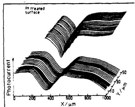
Fig. 2 Line images of the cathodic laser spot photocurrent in 0.1M \text{K}_2\text{SO}_4 at an InSe surface. The decrease in photocurrent is due to recombination at a step between adjacent layers. The upper curves show the effect of Pt treatment on the cathodic laser spot photocurrent.
