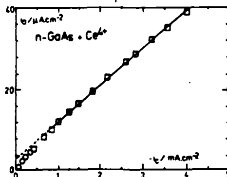
Fig.3. Plot of i_a as a function of i_c measured at an n-GaAs rotating disk electrode in 2 \text{ mol} \cdot \text{dm}^{-3} \text{ H}_2\text{SO}_4 + \text{Ce}(\text{SO}_4)_2 ; T = 298 \text{ K} . \text{Ce}^{4+} concentration: (O) 5 \times 10^{-3} \text{ mol} \cdot \text{dm}^{-3} , (□) 10^{-2} \text{ mol} \cdot \text{dm}^{-3} .
