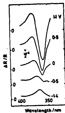
Fig.1 - Electroreflectance spectra of the electrolyte-SiO 2 /Si structure for different applied dc voltages.
