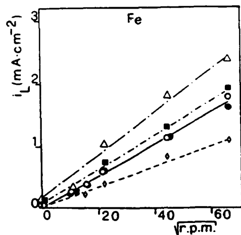
Fig. 1 - i_L for the h.e.r. on Armco iron in 0.001 N acid solutions as a function of the rotation speed (r.p.m.) \Delta HF; \blacksquare HCOOH; \bullet HClO 4 ; \circ HCl \diamond CH 3 COOH
