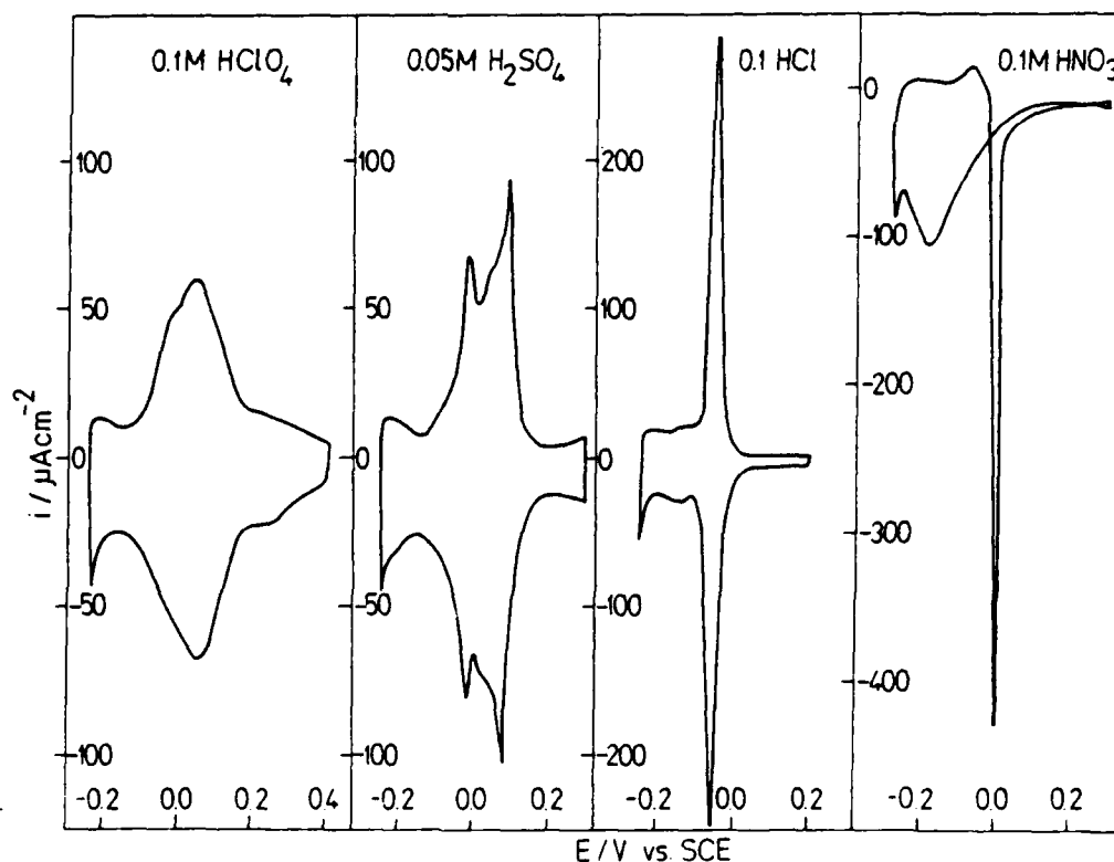
Fig. 1. Cyclic voltammetry for Pt(100) in four different electrolytes. Sweep rate 50 mV/s.
