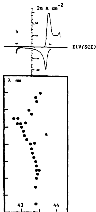
Fig.3 : a - SP dispersion curve of thin Hg film (0.5 \mu\text{m} ) b - i(E) curve of this film in \text{HClO}_4 0.1M
