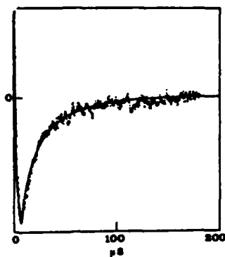
Fig. 2. Transient current measured during pulse protonation of a black lipid membrane made of phosphatidyl cholin (PC) and phosphatidyl serin (PS) at 6-4 molar ratio. The continuous line is reconstruction of the current curve by numerical solution of differential equation.
