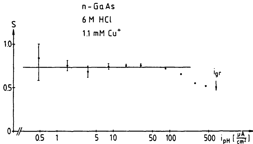
Fig. 2: Stabilisation of n-GaAs against photocorrosion at different light intensities in the same solution as in fig. 1.
