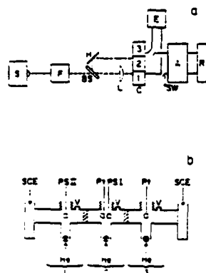
Fig. 1. Experimental apparatus for photogalvanic measurements: S = source; F = water filter; BS = beam splitter; L = lens; C = cell; A = current amplifier; R = recorder; E = electrometer. (b) Details of three-compartment photoelectrochemical cell.
