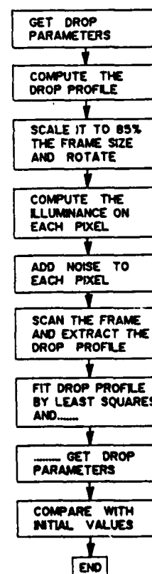
Fig. 2. Flow chart of the simulation program.
