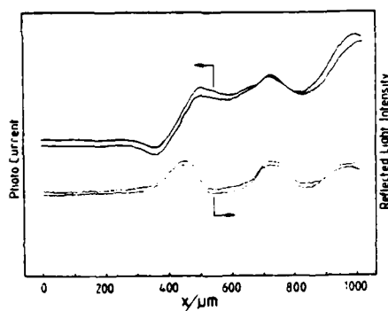
Fig. 3 A computer generated picture showing the effect of Pt treatment on the photocurrent. A drop of 20 mM \text{H}_2\text{PtCl}_4 was applied onto the electrode for 5 min, which was then rinsed with water. The photocurrent is much higher at the area which was covered with the Pt solution compared to the untreated area. The scanned area is 400 \mu\text{m} in Y-direction and 1000 \mu\text{m} in X-direction.
