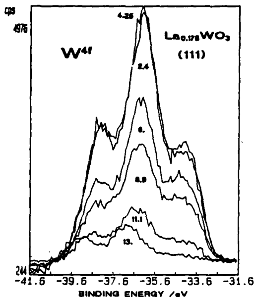
Fig. 2 W^{4f} spectra of emersed surfaces at different pH values of the electrolyte.
