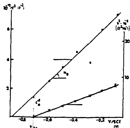
Fig. 3. Variations of (●) 1/C ( C is the high frequency value of the capacity) and (X) b^2 as a function of the steady potential V . No tartare added.
