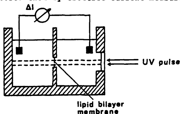
Fig. 1. Schematic presentation of the observation cell.
