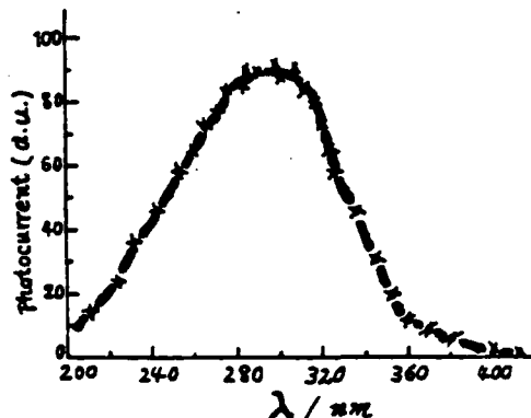
Fig. 3, The photoresponse vs. wave length for a r.f. sputtered TiO_2 (rutile) anode in 1M NaOH electrolyte.
