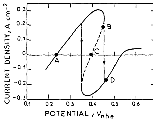
Figure 1 : Polarisation curve. Co in 11M- HNO_3 . Broken line, that obtained with a negative resistance.
