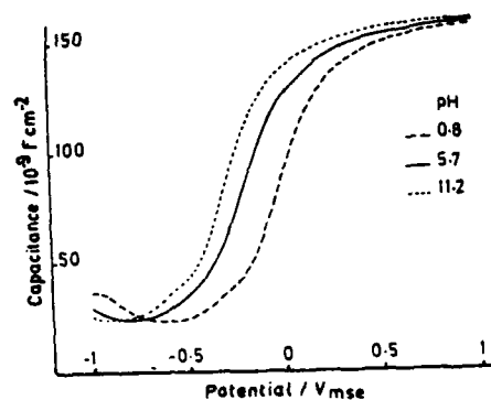
Fig.2 - Influence of the pH on the capacity-potential characteristics of the electrolyte - SiO 2 /Si junction.
