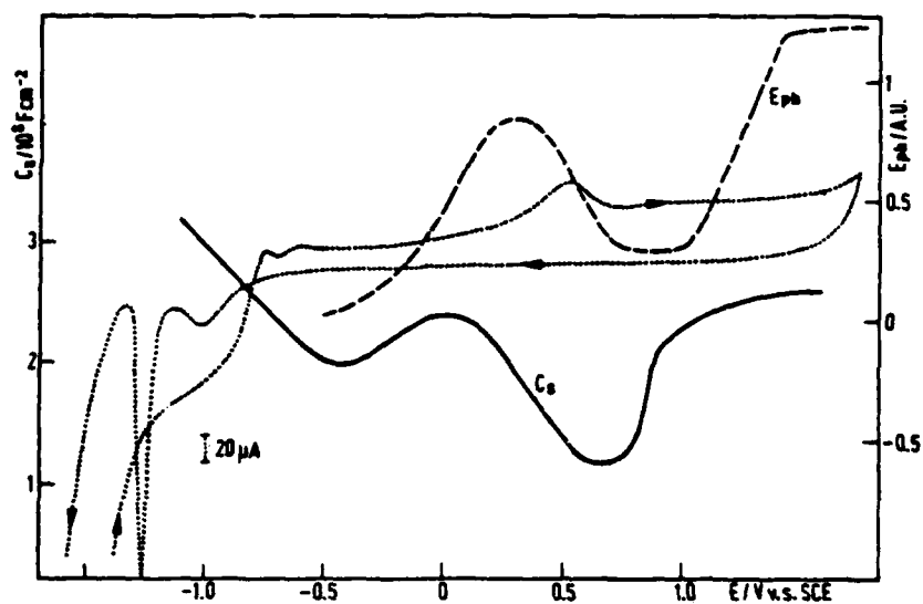
Fig.1. Capacitance, photopotential curves and cyclic voltammogram obtained at 10 mV/s, on freshly polished tin electrode in 0.05M borate buffer solutions, pH=8.2.
