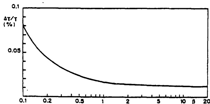
Fig. 3. 'Single shot' accuracy vs \beta value (camera resolution 512 \times 512 pixel, N/S ratio = 0.01).
