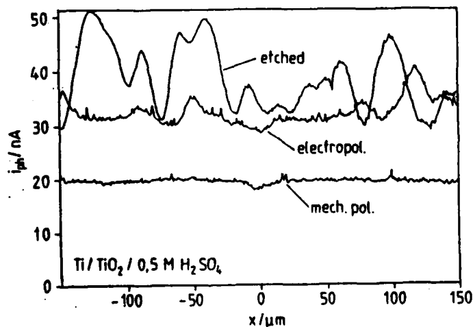
Fig. 1: Local photocurrent measurements of Ti-electrodes after different pretreatment (mechanical-, electropolishing and etching) and following passivation \epsilon_{ox} = 5 \text{ V} ; \epsilon = 1.5 \text{ V} ; P = 10 \text{ μW}
