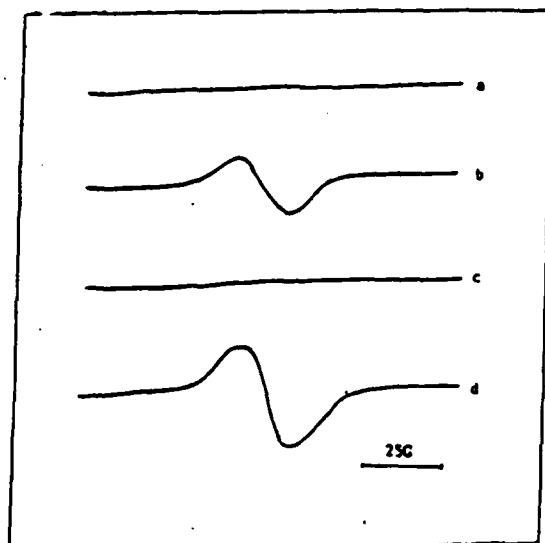
Fig.2 ESR signals of 1 \cdot 10^{-3}M MB during potential scan a: start, b: scan from 0.2 to -0.13V , c: at -0.4V , d: reverse scan from -0.4 to -0.13V .
