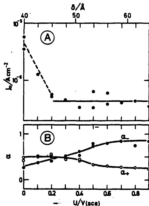
Fig. 3. Exchange current (A) and symmetry factors (B) from initial Tafel data for various U' or \delta ( \text{pH} = 3.0 , j_f = 2 \mu\text{Acm}^{-2} , (\text{ox}) = (\text{red}) = 0.01 \text{ M} ).
