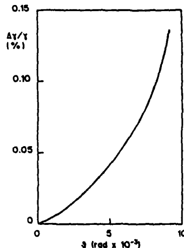
Fig. 4. Systematic error in \gamma due to misalignment of the camera vertical axis.
