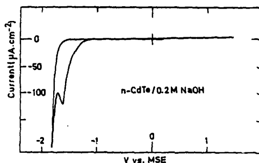
Fig. 1 Dark current versus potential characteristic of n-CdTe in basic electrolyte
