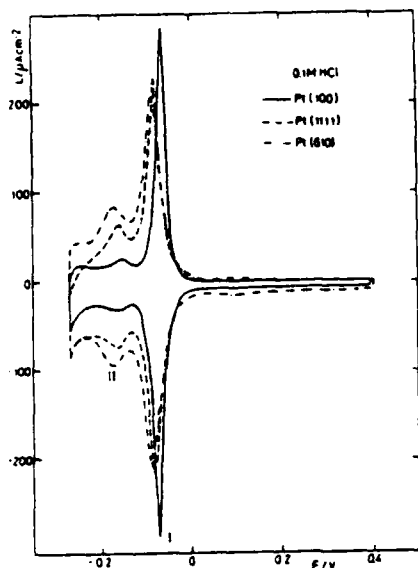
Fig. 2. Comparison of the voltammetry curves for Pt(100), Pt(11, 1, 1) and Pt(610) in 0,1M HCl. Sweep rate 50 mV/s.
