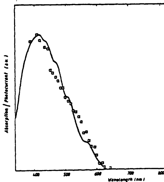
FIG. 4. Absorption spectrum (full line) and photocurrent action spectrum (squares) of 6T in 0.02 M \text{EuCl}_3 water solution at 0.4 V vs. sce.
