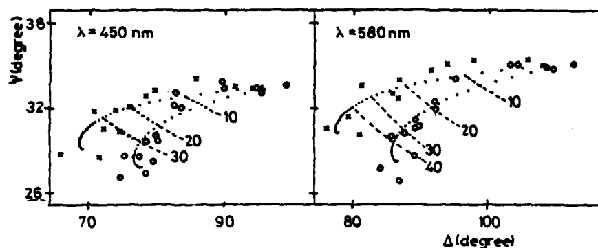
Fig. 2.- Ellipsometric data ( \Delta - \psi plots) at two wavelengths corresponding to the electroreduced platinum overlayers under different conditions, (x) v = 2 \text{ mV s}^{-1} , (o) v = 100 \text{ mV s}^{-1} . The numbers indicate the film thickness in nm.
