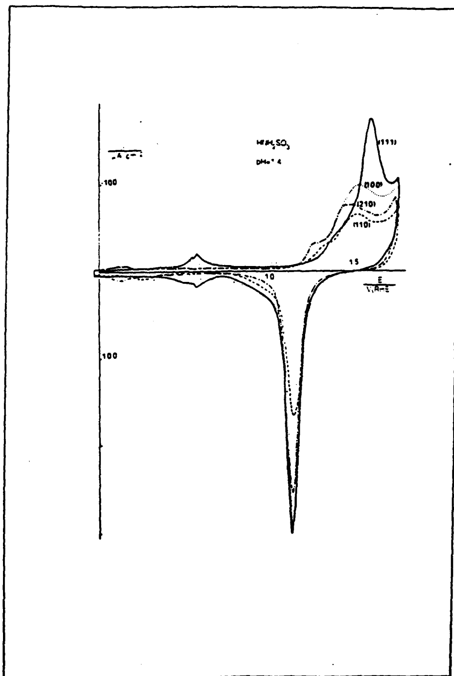
Figure 2- Cyclic voltammetry i-E profiles for Au single crystal face electrodes in sulphamic acid solutions recorded at 50 \text{ mVs}^{-1} and 25^\circ\text{C}
