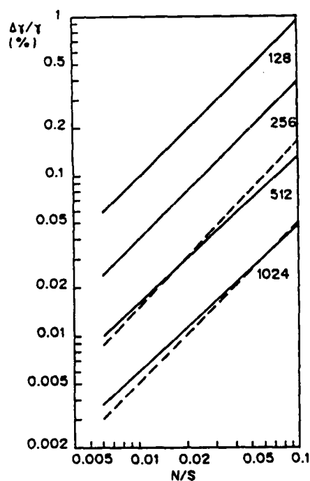
Fig. 1. 'Single shot' accuracy in interfacial tension vs noise to signal ratio for a camera resolution from 128 \times 128 to 1024 \times 1024 pixel and a shape factor \beta = 5 .
