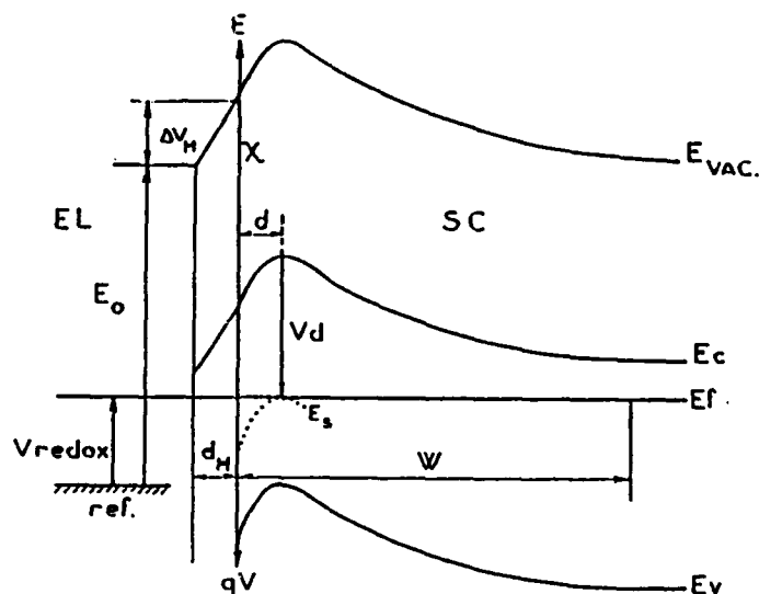
Fig. 1 : Energy diagram of a semiconductor/electrolyte junction in the case of a spatial distribution of interface states.
