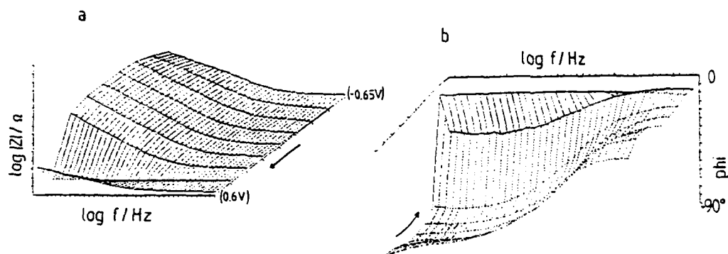
Figure 2. (a) Bode plot and (b) phase surface of the system n\text{-FeS}_2/0.5\text{M H}_2\text{SO}_4 + 0.1\text{M Br}^- under illumination using RG-645 cut-off filter. Geometric electrode area is 0.029\text{ cm}^2 . The polarization (vs \text{HgSO}_4 ) of the curves is related to the drawn lines (1-9) as follows: (1) -0.65 ; (2) -0.5 ; (3) -0.35 ; (4) -0.2 ; (5) -0.05 ; (6) 0.1 ; (7) 0.2 ; (8) 0.4 ; (9) 0.6\text{V} . Arrows indicate the anodic direction.
