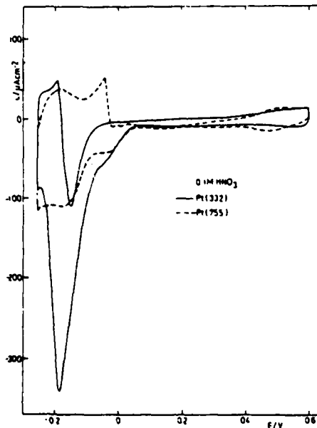
Fig. 4. Cyclic voltammograms for Pt(755) and Pt(332) in 0,1M HNO 3 . Sweep rate 50 mV/s.
