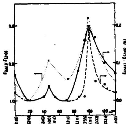
Fig. 2. Correlation between \delta(hkl)/\delta(210) and E(hkl) - E(210) and E_{av} - E(210) in the dependence of crystallographic orientation.
