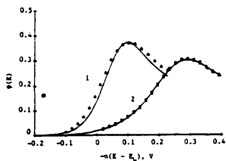
Fig. 1. Variation of current function, \psi(E) with potential for OPG (A) and uncycled HOPG (X) in O_2 -saturated CH_3CN (0.1 M TEAP). Scan rate: 500 \text{ mV s}^{-1} . Solid lines are theoretical curves for ideal quasi-reversible behavior.
