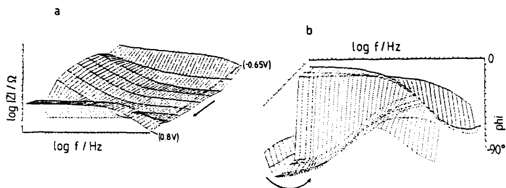
Figure 1. (a) Bode plot and (b) phase angle surface of the system n\text{-FeS}_2/0.5\text{M H}_2\text{SO}_4 + 0.1\text{M Br}^- in darkness. Geometric electrode area is 0.029\text{ cm}^2 . The polarization (vs \text{HgSO}_4 ) of the curves is related to the drawn lines (1-10) as follows: (1) -0.65 ; (2) -0.5 ; (3) -0.35 ; (4) -0.2 ; (5) -0.05 ; (6) 0.1 ; (7) 0.2 ; (8) 0.4 ; (9) 0.6 ; (10) 0.8\text{V} . Arrows indicate the anodic direction.
