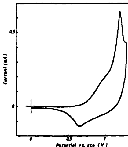
FIG. 1. Cyclic voltammogram of \alpha -sexithienyl (6T) evaporated on \text{SnO}_2 glass, in 0.1 M \text{LiClO}_4 acetonitrile solution. Scan speed : 10 mV/s.
