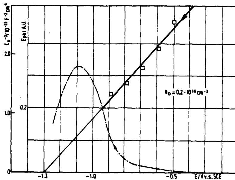
Fig.2. Photopotential-potential plot and the Mott-Schottky plot at 1000 Hz for an oxide covered tin electrode (n-type) in 0.05M borate buffer solutions, pH=8.2.
