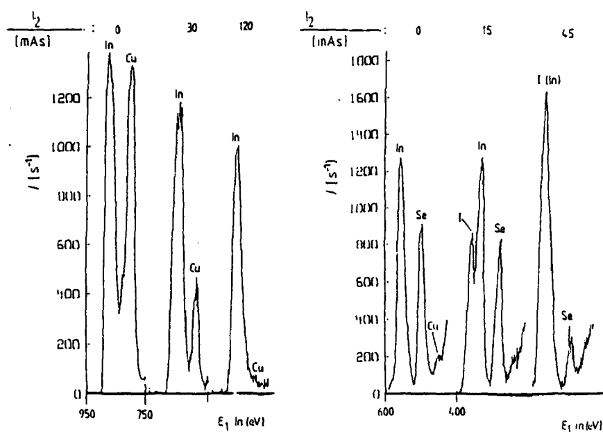
Fig 1. LEISS data (He and Ne) of CuInSe 2 /I 2 interfaces
