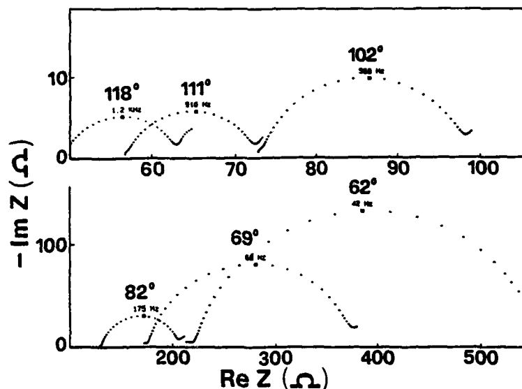
Fig.1 . Complex impedance plots for the cell \text{Pb}/(\text{PEO})_{40}.\text{Pb}(\text{ClO}_4)_2/\text{Pb} at the indicated temperatures.
