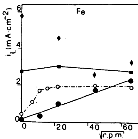
Fig. 3 - i_L for the h.e.r. in various solutions of HF, on Armco iron: \blacklozenge 1N; \blacksquare 0.1 N; \circ 0.01 N \bullet 0.001 N
