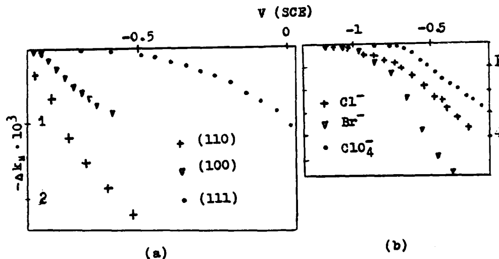
Fig.1 Potential dependence of the position of SP resonance [3-5] : (a) effect of surface orientation (Ag(hkl))-0.5 M NaClO 4 ; (b) effect of adsorption of anions (Ag polycrystalline). \Delta k_u in units \omega/c .
