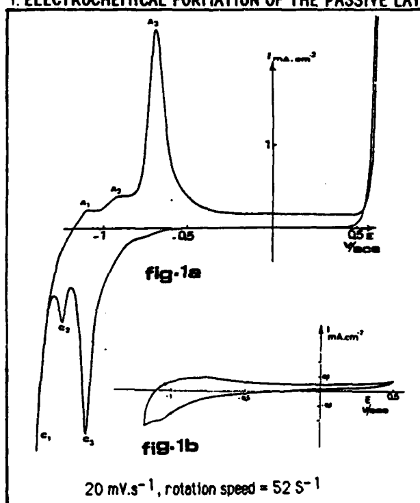
Fig. 1a shows the well-known voltammogram concerning the electrochemical behavior of Fe 2N in alkaline solution (rotating disc electrode). The protocole to form the oxide layer studied in this paper consists in multi cyclic polarisation in a domain of potential cathodically limited at -1.15\text{V/SCE} and anodically limited at 0\text{V} . The cathodic limit has been chosen between C_2 and C_3 to prevent the destruction of the inner layer of \text{Fe}^{2+} oxide.
