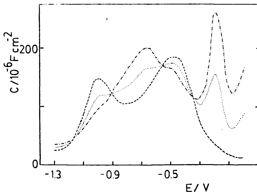
Fig. 1.- C vs. E response for thin silver film electrodes in 0.04 N KCl for different number of potential cycles the anodic limit was changed from -0.3 V to 0.0 V at the 4th cycle. (---) 1st cycle, (...) 6th cycle, (-.-) 12th cycle.
