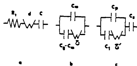
Fig. 1. Equivalent circuits for the impedance in the high frequency range.
