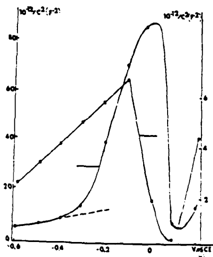
Fig. 4. Variations of 1/C as a function of V (●) with and (■) without tartare addition.
