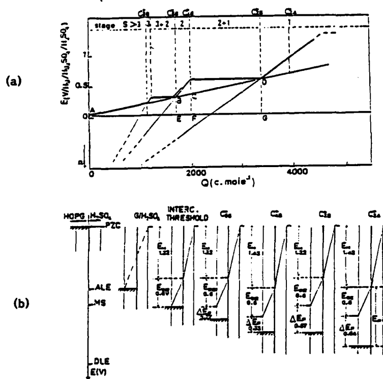
Fig.1(a) Potential charge E(Q) curve for slow intercalation of H_2SO_4 13 M into HOPG : Potential plateaus correspond to two-phases domains, while slopes correspond to pure stage domains except for the mixtures of high-stage compounds.
