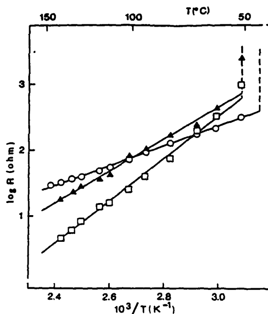
Fig. 2. Bulk resistance R_b (○), charge transfer resistance R_{ct} (□) and diffusion impedance Z_d (△) as a function of 10^3/T .
