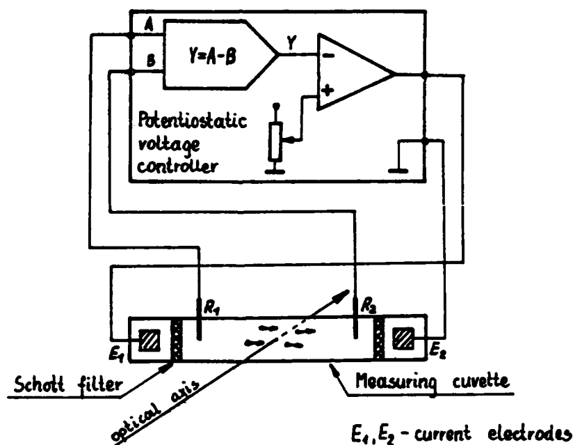
Fig. 1. The block diagram of microelectrophoretic setup.
