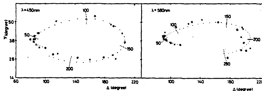
Fig. 1.- Ellipsometric data ( \Delta - \psi plots) at two different wavelengths corresponding to hydrous platinum oxide layers obtained through RSWPS at 3.12 \text{ kHz} . The numbers indicate the film thickness in nm.
