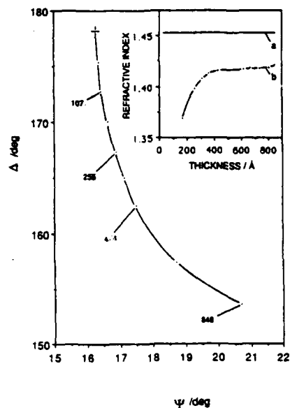
Fig. 2: Ellipsometric Profile during formation of an electrochemical oxide on p-Si <111> N_A = 1.5 \cdot 10^{16} \text{ cm}^{-3} in Phthalate buffer at \phi = 60^\circ , \lambda = 632.8 \text{ nm} . Numbers at the graph denote thickness in Å. Insert: Comparison of the calculated refractive index vs. thickness for the b) electrochemical oxide and a) thermal oxide.
