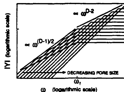
Fig.4. Typical behavior for the Faradaic impedance of a fractal electrode in the presence of diffusion: the characteristic frequency \omega_f is of the order of 1/D(cr)^2 with c = (z^2 e^2 / kT) c_{red} c_{ox} / (c_{red} + c_{ox}) .
