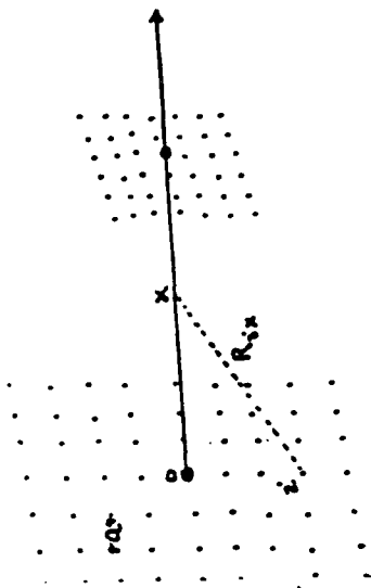
FIGURE 2a. Grids of charge locations utilized in computations of electric potential profiles presented in figures 2 and 3. No charge is present at origin, in order to avoid singularity.
