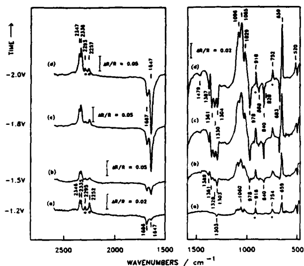
Figure 1: Steady-state FTIR reflectance spectra for \text{CO}_2 reduction in \text{CO}_2 saturated \text{CH}_3\text{CN}/0.1 \text{ M TBAF} as a function of electrode (Pt) potential. The reference spectrum for (a)-(d) was obtained at 0.4 V. Stars indicate the positions of strong \text{CH}_3\text{CN} bands.
