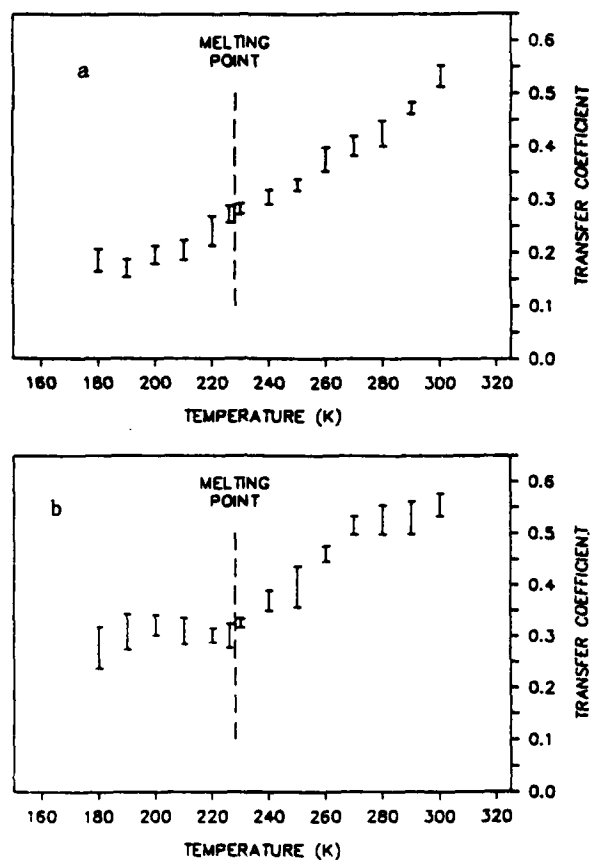
fig. 1: transfer coefficient for the proton discharge as a function of temperature a: gold electrodes b: silver electrodes
