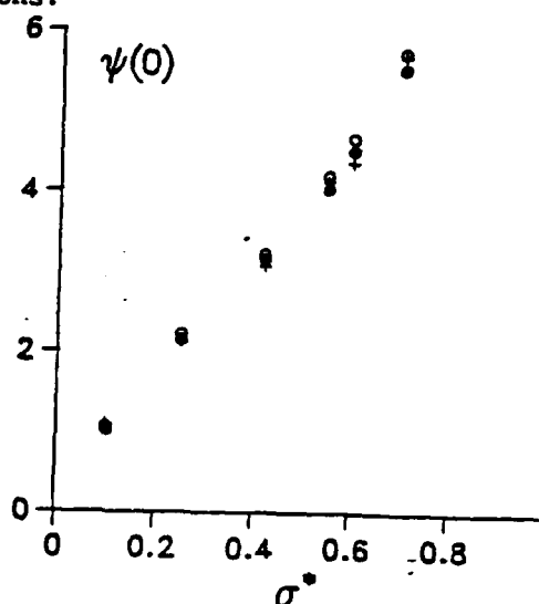
Figure 2: \Psi(0) as function of \sigma^* . Filled circles:MSA, open circles:HNC, crosses: data of reference 6.
