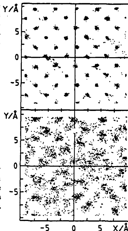
Figure 3: Density distribution in the xy-plane for the first (top) and second (bottom) layer of oxygen atoms (see text for exact definition). A dot is made every 0.15 ps at the (x,y)-position of oxygen atoms which are located in the corresponding layer at that time.
