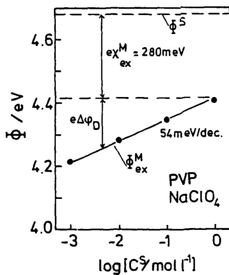
Fig. 1 The work function of the electrolyte, \phi_S , at E=0.0 \text{ V/SCE} , and of the coated electrodes emersed at the same E , \phi_{ex}^M
