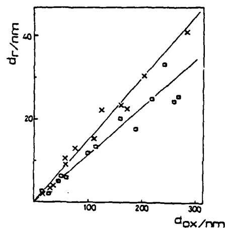
Fig. 4.- d_r vs. d_{ox} plot. (x) v = 2 \text{ mV s}^{-1} ; ( \square ) v = 100 \text{ mV s}^{-1} .
