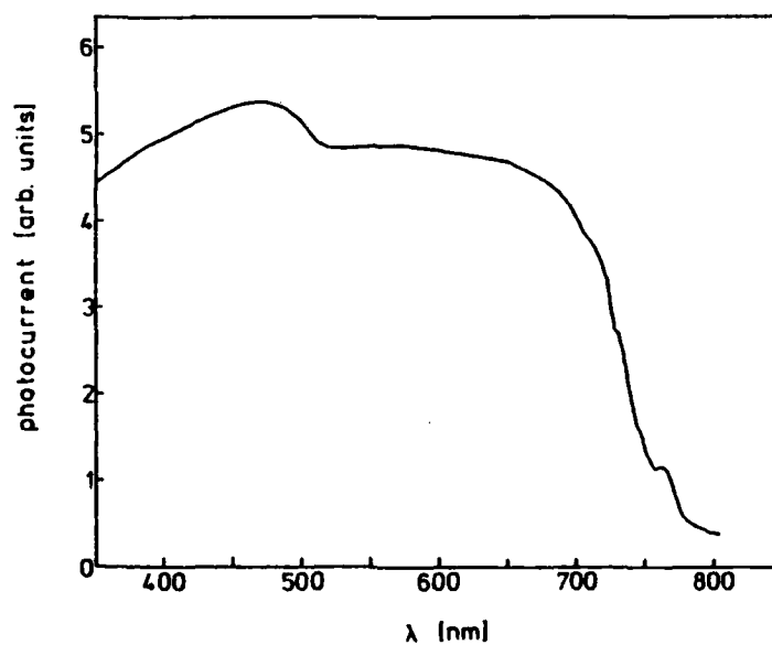
Fig. 2: Excitation spectrum of the hole photocurrent originating in the functionalized Langmuir Blodgett film (uncorrected).
