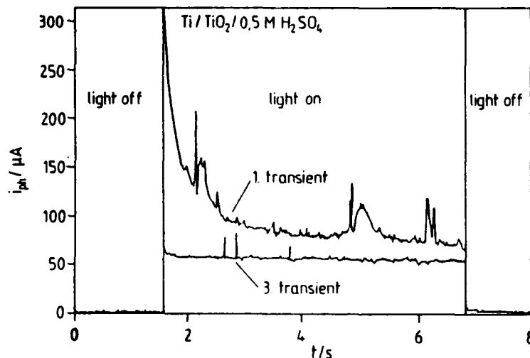
Fig. 2: Photocurrent transients for a 1st and 3rd run, \epsilon_{ox}=5\text{ V} , \epsilon=1.6\text{ V} , power density PD=40\text{ kW/cm}^2 .
