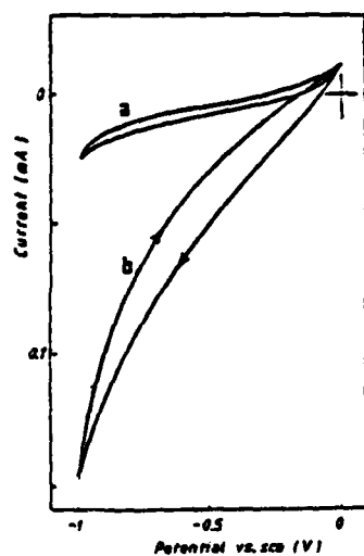
FIG. 3. Current-voltage plot of 6T in 0.02 M \text{EuCl}_3 water solution in the dark (a) and under white light illumination (b)
