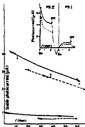
Steady photocurrent versus time for PS II (O) and PS I (X) covered electrodes. (—) Both electrodes illuminated; (---) only one electrode illuminated. Compartment (1) contains pH 7 buffer phosphate solution; compartment (2) contains 1.0 \times 10^{-3} M 1:1 [Fe(CN)_6]^{3-}/[Fe(CN)_6]^{4-} in pH 7 phosphate buffer solution; compartment (3) contains 1.2 \times 10^{-3} M NADP^+ in pH 7 phosphate buffer solution. The on and off arrows indicate the turning on and off of illumination of the second photochemical system. Inset: Photocurrent-time behavior for PS II and PS I-covered electrodes with both electrodes (—) or only one (---) illuminated electrode. Arrows indicate the turning on and off of the light.
