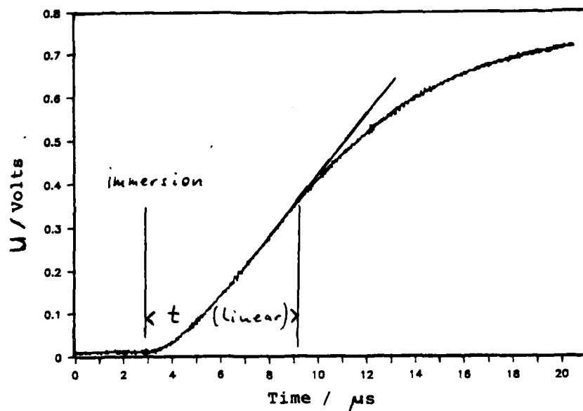
Figure 1 Potential vs. time immersion transient for Au into 0.01 M \text{HClO}_4 (potential w.r.t. internal Pd reference at 0.615 V against \text{Hg/Hg}_2\text{SO}_4 ).
