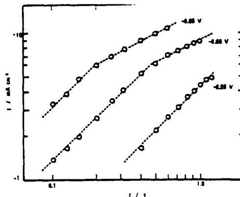
Fig. 3 \log j - \log t plot for the growth of Al-nuclei. Slopes are 1 and 0.5.
