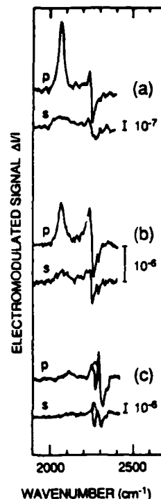
Fig.2. \nu SiH spectrum for s and p polarizations. (a) 10h-aged interface; (b) 78h-aged; (c) anodically oxidized. Notice the different behaviors of the two \nu SiH peaks upon changing the polarization. The 2270 cm -1 peak is superimposed with a sharp \nu CN line. The dotted line in (c) is an attempt to remove the \nu CN contribution. Electromodulated charges (a) 0.95, (b) 1.8, (c) 18 \times 10^{-7} C/cm 2 .
