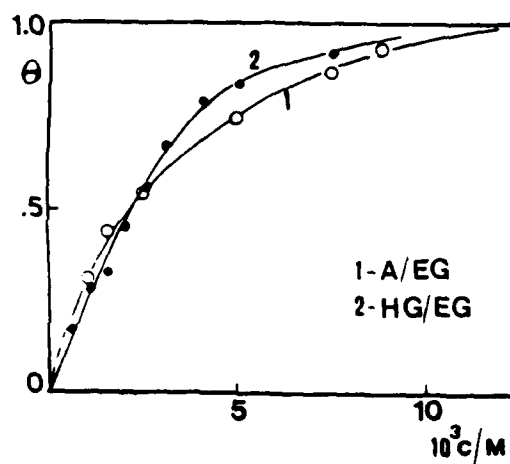
Fig.3-Adsorption isotherm of LN at the A/EG (O) and HG/EG (●) interface from 0.5M NaClO 4 solutions.
