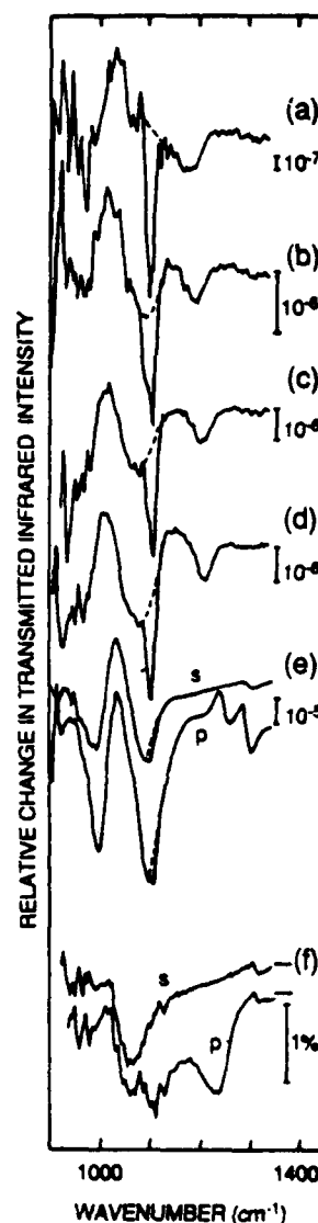
Fig.4. \nu SiO spectrum for acetonitrile + TBAP electrolyte. (a) 8h-aged interface; (b) 26h-aged; (c) 80h-aged; (d) 144h-aged; (e) anodically oxidized (+5 V, \sim 100 \mu\text{A}/\text{cm}^2 , 5 min.); (f) classical transmission spectrum of the oxidized surface (same as (e)) normalized to the initial surface. Electromodulated charges (a) 1.2, (b) 1.9, (c) 2.2, (d) 2.2, (e) 18 \times 10^{-7} \text{C}/\text{cm}^2 . The dashed lines have been drawn to remove the \nu ClO peak due to the perchlorate ion.
