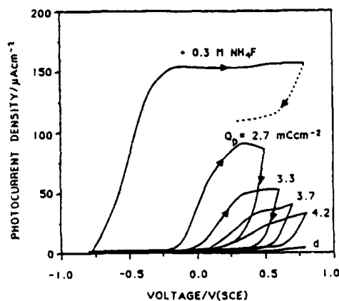
Fig. 1: Cyclic voltammogram of an untreated intrinsic a-Si:H layer deposited on stainless steel under white illumination (20 mWcm -2 ). Lower curves: in phthalate buffer pH 4.5, the integrated charge Q_p is given for successive cycles. Upper curve: after addition of 0.3M NH 4 F. Scan velocity : 20 mVs -1 .
