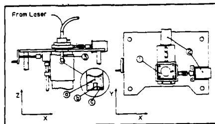
Fig. 1 The experimental equipment used for the LSS experiment. (1) x-y coordinate table. (2) Step motors. (3) Laser spot probe with (a) single mode optical fibre, (b) Selfoc microlens and (c) assembly of optical fibres.
