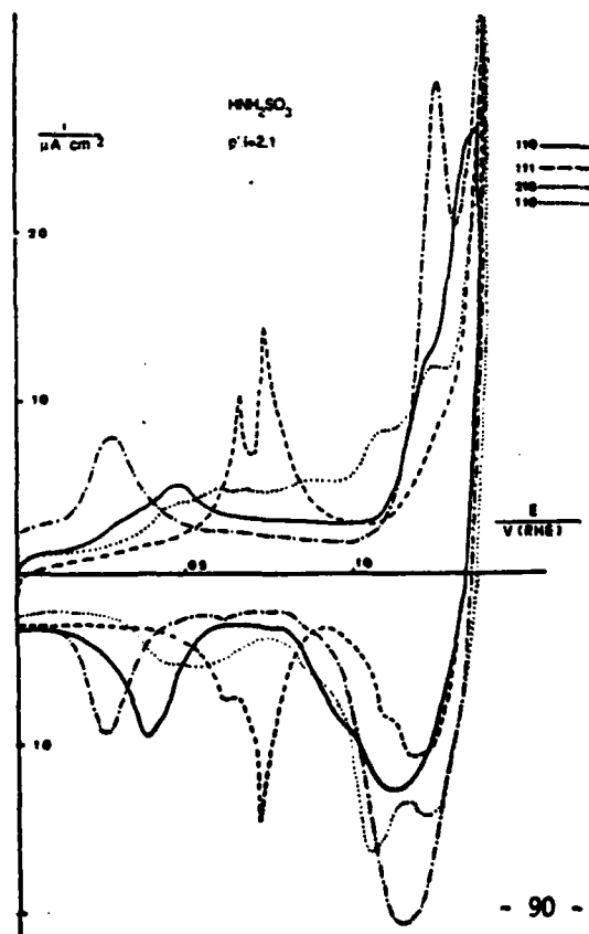
Figure 3-i-E profiles for the early oxidation of gold face electrodes in sulphamic acid solutions
