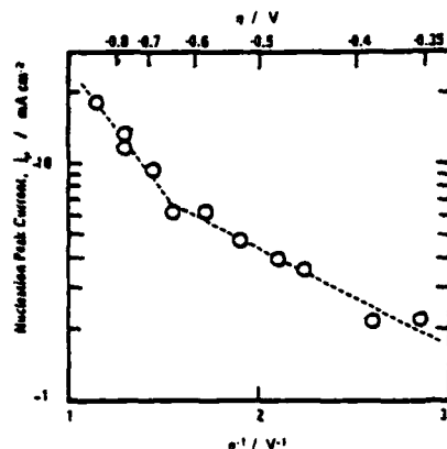
Fig. 2 Nucleation peak current vs. \eta^{-1} . Potential dependence of 2D-nucleation.
