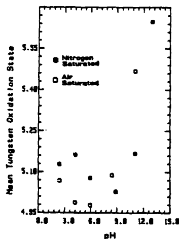
Fig. 3 Mean tungsten oxidation state n_{ox} dependent on the solution acidity.
