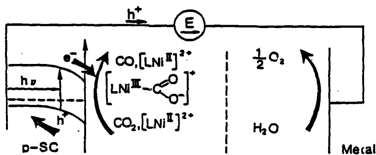
Figure 1 Principle of the photoelectrochemical cells (A) and (B).
