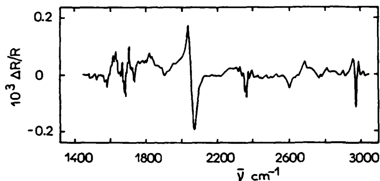
Fig.2 : EMIRS spectrum of the species resulting from the chemisorption of 10^{-3} M C_2H_5OH in 0.5 M HClO_4 at a Pt polycrystalline electrode (modulation amplitude 400 mV, mean potential 0.2 V/RHE, f = 13.6 Hz, room temperature, 35 averaged scans).
