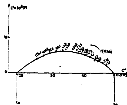
Fig. 2. Cole-Cole plot for the high frequency range; V = -0.4 V SCE; C(X^-) = 0 .
