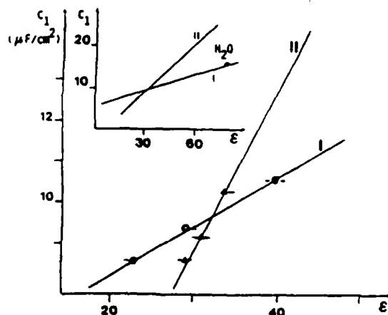
Fig.3-Dependence of C 1 on solvent bulk permittivity, ε.
