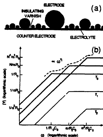
Fig. 1. Illustration of the use of the Bode plot for finding a CPA exponent. Case of the "parallel spherical pore" electrode (shown in (a)) with N=2 and \alpha=1.6 .
