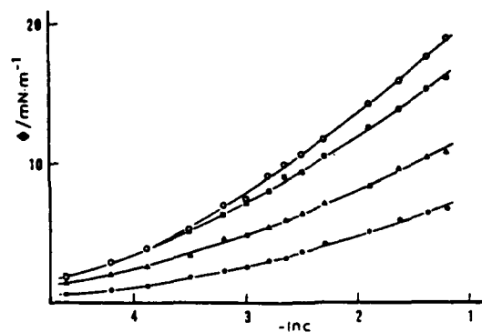
Fig. 2 Surface pressure against \ln c for TPO adsorption at the following surface charge densities (○) -7.5; (◻) -6; (Δ) -4; (●) -2 \mu\text{C}\cdot\text{cm}^{-2} .
