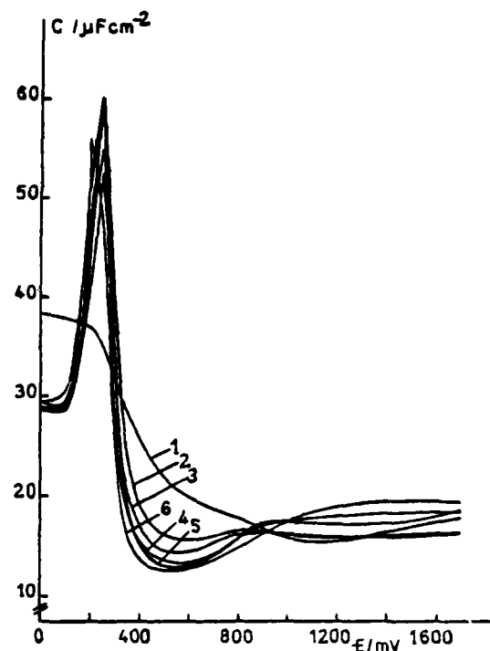
Fig.1. Double layer capacity curves for aqueous 0.1M Na 2 SO 4 containing \beta -CD at the following concentrations: (1) 0, (2) 0.02, (3) 0.05 (4) 0.314, (5) 0.785, (6) 3.14 mmol·l -1
