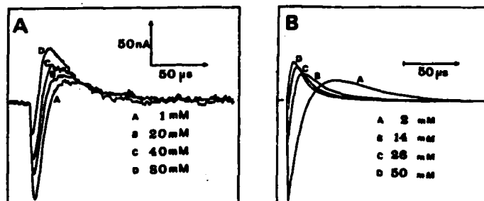
Fig. 3. A - current transient recorded after proton pulsing of a PC+PS black lipid membrane in presence of monensin and increasing K^+ concentrations. B - Simulation of the current transient by numerical solution of differential equation pertinent to the system described in scheme I.
