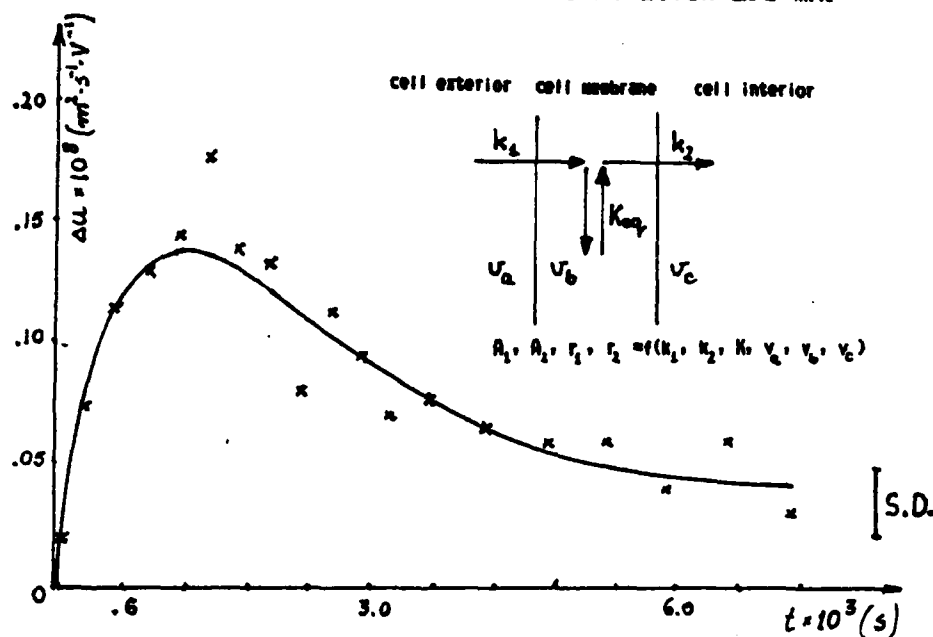
Fig.2. Changes in the electrophoretic mobility of human red blood cells influenced by \text{Pi}^- anions; solid line represents the calculated curve. S.D. - standard deviation.
