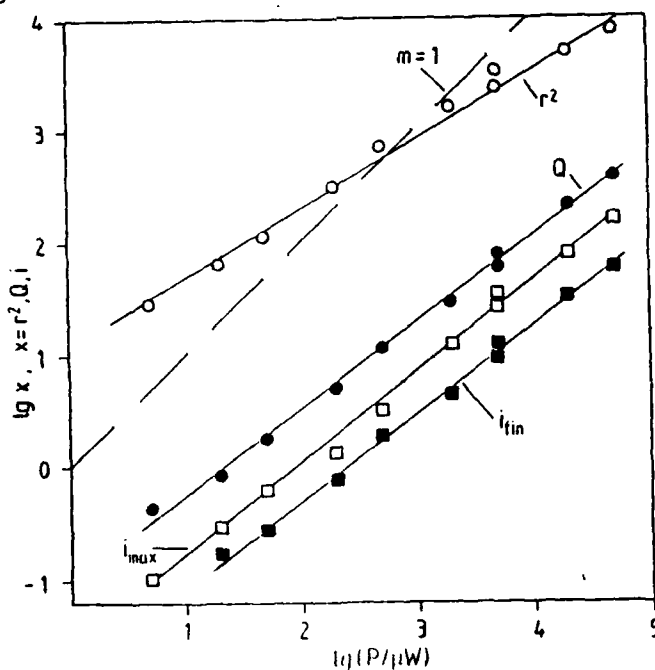
Fig. 3: Intensity P ( \mu W ) dependence of i_{max} , i_{min} ( \mu A ); charge Q ( \mu C ); A \sim r^2 ( \mu m^2 ) in a double logarithmic scale
