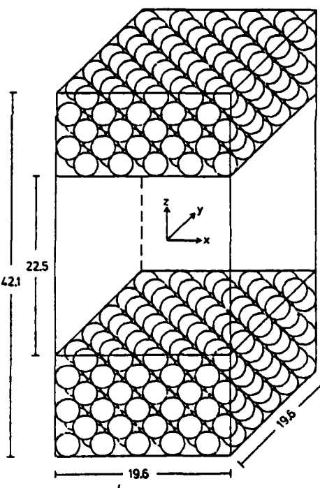
Figure 1: Sketch of the basic tetragonal simulation cell. The water molecules are located in the center of the box and the platinum atoms are represented by the circles. All distances are in Å.
