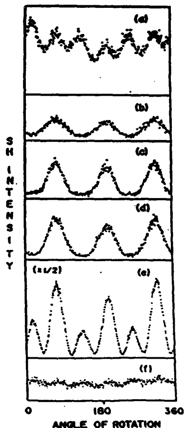
Figure 3. Dependence on Tl coverage of the p-polarized SH intensity as a function of angle of rotation for the solution in figure 2 at: (a) 0.00V (b) -0.52V (c) -0.57V (d) -0.67V (e) -0.85V (f) -0.90V.
