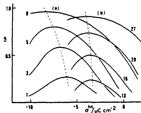
Fig.1 Plots of \theta vs \sigma^M calculated at various \ln(\beta c) values indicated by the lines for (a) r=3 , \alpha_A=7 \cdot 10^{-29} \text{ m}^3 and (b) r=7 , \alpha_A=1.2 \cdot 10^{-28} \text{ m}^3 . Other molecular parameters: P_A=1.4 \cdot 10^{-29} \text{ Cm} , P_S=6 \cdot 10^{-30} \text{ Cm} , \alpha_+ = \alpha_- = 1 \cdot 10^{-28} \text{ m}^3 , \alpha_+ = \alpha_- / 2 , d=5.2 \cdot 10^{-10} \text{ m} , z_e=10.6 , n_+ = r , n_- = n_+ / 2 , \Delta U=0 , \beta'=100 , A^{AS}=0 . The meaning of symbols is given in ref.2.
