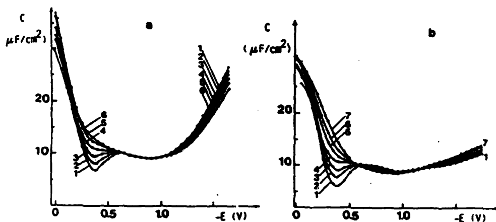
Fig.1. Differential capacity curves of a Hg electrode in contact with KF solutions in 1,4-BD (a) and \text{LiClO}_4 solutions in 1,4-BD (b) at different concentrations: (1) 0.005; (2) 0.01; (3) 0.02; (4) 0.05; (5) 0.1; (6) 0.2; (7) 0.5.
