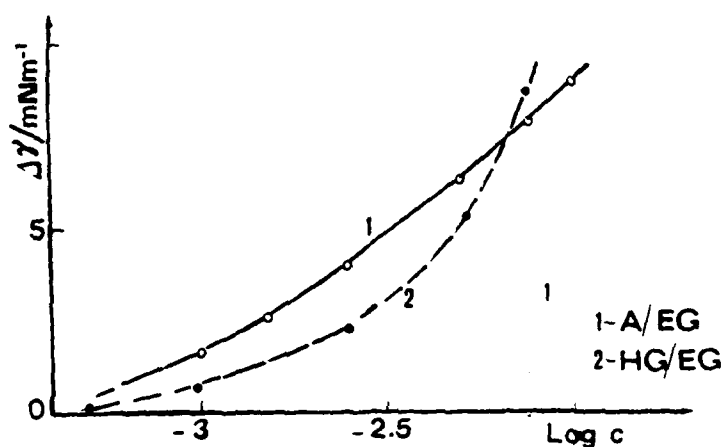
Fig.2-Surface pressure curves of LN at the A/EG (1) and at the HG/EG interface (2).
