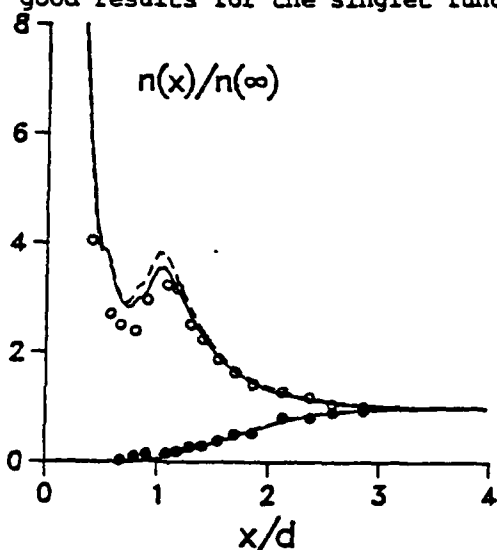
Figure 1: n(x) for \sigma^*=0.7 . Solid line:MSA, dashed line:HNC, points: data of reference 6
