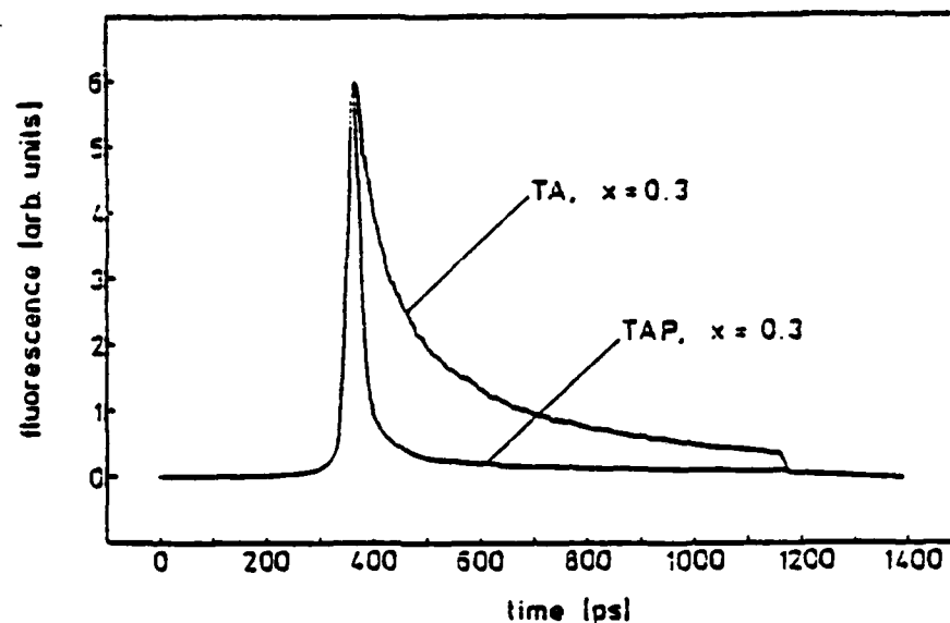
Fig. 1: Charge transfer fluorescence decay in the LB film in the presence (TAP) (lower curve) and in the absence (TA) (upper curve) of the third chromophore (normalized). x is the molar ratio of photoactive to inert supporting molecules.
