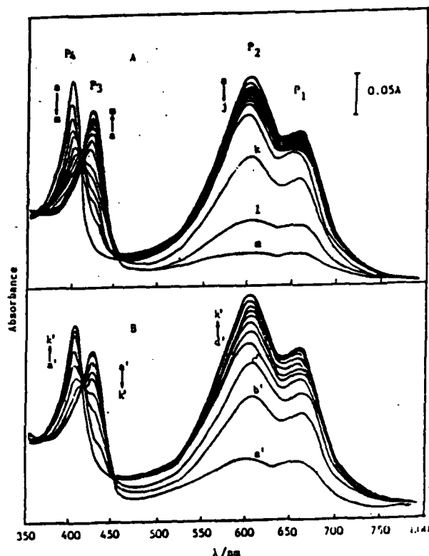
Fig.1 Spectra of Hb at Pt electrode in 1.10^{-4} M MB
