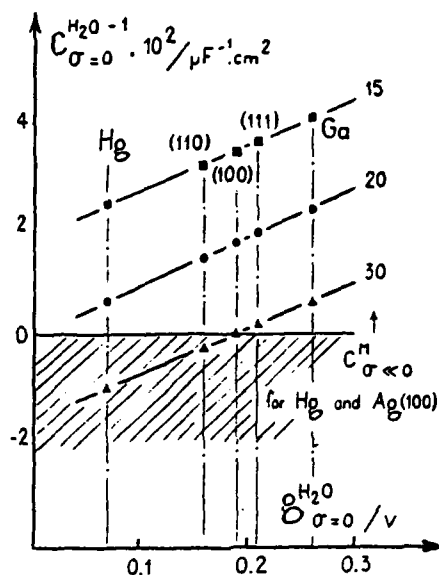
Fig. 1. (C_{\sigma=0}^{H_2O})^{-1} as a function of g_{\sigma=0}^{H_2O} for different C_{\sigma \ll 0}^M .
