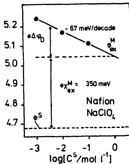
Fig. 1 The work function of the electrolyte, \phi_S , at E=0.0 \text{ V/SCE} , and of the coated electrodes emersed at the same E , \phi_{ex}^M
