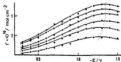
Fig. 3 Surface excess of TPO vs potential with respect to a 0.1M LiCl/H 2 O calomel electrode at the following concentrations of TPO: 0.2; 0.1; 0.05; 0.03; 0.02; 0.01 \text{mol}\cdot\text{dm}^{-3} .
