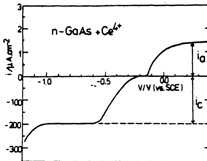
Fig.1. Current-potential curve measured at an n-GaAs rotating disk electrode in aqueous 2 \text{ mol.dm}^{-3} \text{ H}_2\text{SO}_4 + 10^{-2} \text{ mol.dm}^{-3} \text{ Ce}(\text{SO}_4)_2 ; rotation rate 17 \text{ s}^{-1} ; T = 298 \text{ K} .
