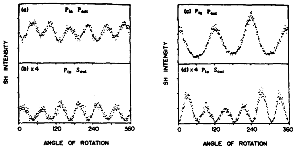
Figure 1. SH intensity as a function of angle of rotation for (a) Ag(111) electrode immersed in 0.1M \text{NaClO}_4 at -0.19\text{V} vs \text{Ag}/\text{AgCl} ; p-polarized SH light; (b) Same as (a) with s-polarized SH light. (c) Cu(111) in 0.1M \text{Na}_2\text{SO}_4 at -0.3\text{V} ; p-polarized SH light; (d) same as (c) with s-polarized SH light.
