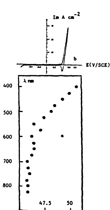
Fig.2 : a - SP dispersion curve of thick Hg film (1-5 \mu\text{m} ) b - i(E) curve of this film in \text{HClO}_4 0.1M.
