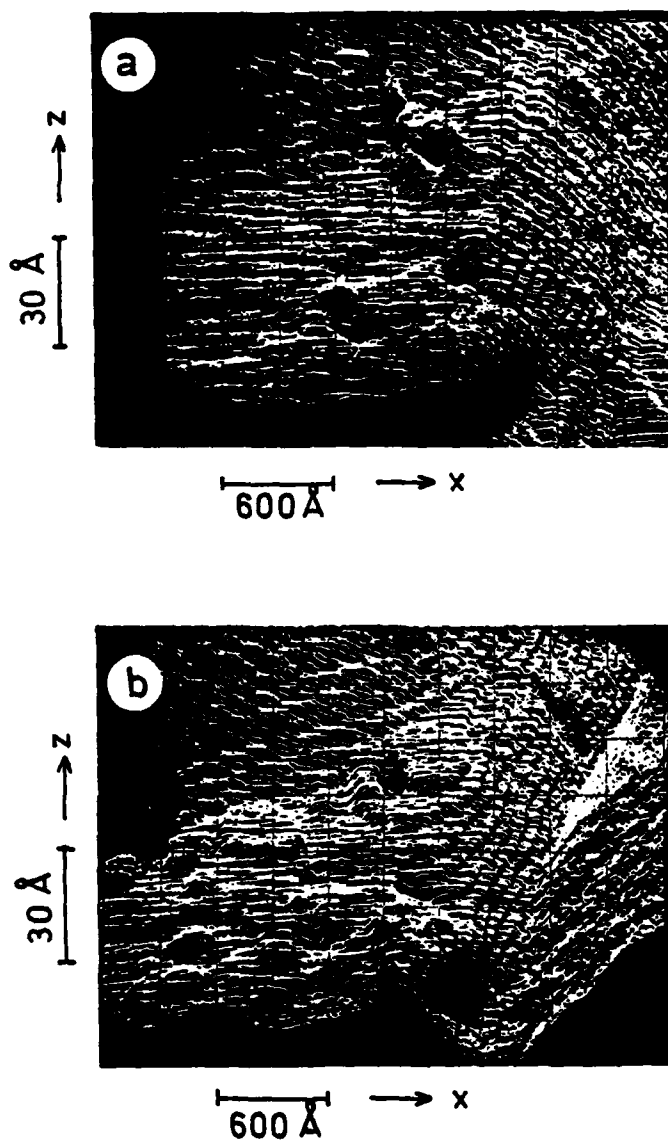
Fig. 2: (a) STM image ( 2700 \text{ \AA} \times 2700 \text{ \AA} ) of a clean, freshly flame-treated Au(111) surface at rest potential in 0.05 \text{ M H}_2\text{SO}_4 . (b) STM image of the above region, again at rest potential in the same solution, having cycled the electrode once to 1.5 \text{ V(Pd-H)} and back, at 10 \text{ mV s}^{-1} .
