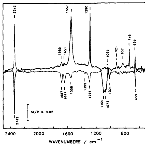
Figure 2: In situ FTIR reflectance spectra for the oxidation of TBAOX (0.01 M) in \text{CH}_3\text{CN}/0.1 \text{ M TBAF} at Pt/0.1 V (thick curve). The reference spectrum was obtained at -1.5 V. Re-reduction of the TBAOX oxidation product ( \text{CO}_2 at Pt/-1.8 V (thin curve). The reference spectrum was collected at 0.1 V. Stars indicate the positions of strong \text{CH}_3 bands.
