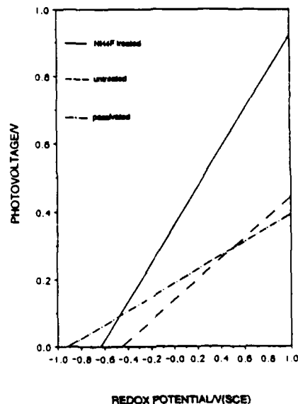
Fig. 4: Dependence of photopotential for a-Si:H/redox electrolyte junctions on redox potential for differently prepared surfaces. Redox couples: Ce 3+/4+ , Fe 2+/3+ , Fe(CN) 3-/4- , I 1/3- , V 2+/3+ . Where photovoltages were not constant, initial values are plotted in the figure.
