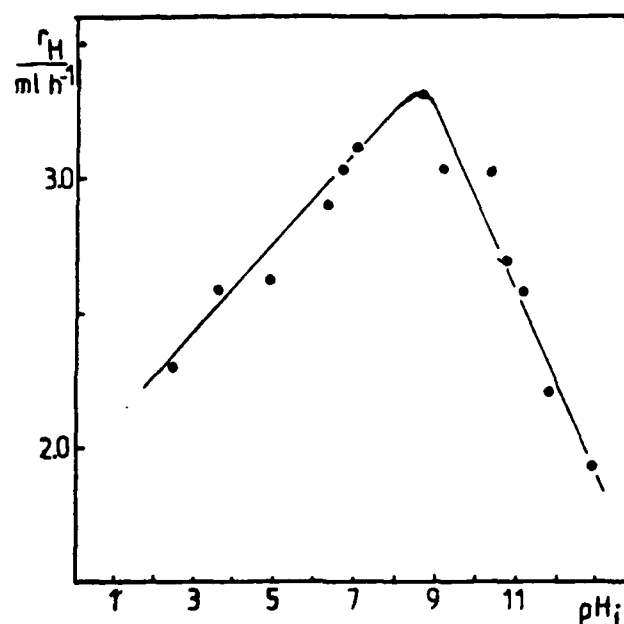
Figure r_H vs. pH_i for Pt/TiO 2 suspensions in 0.1 M sorbitol solution at 25°C.
