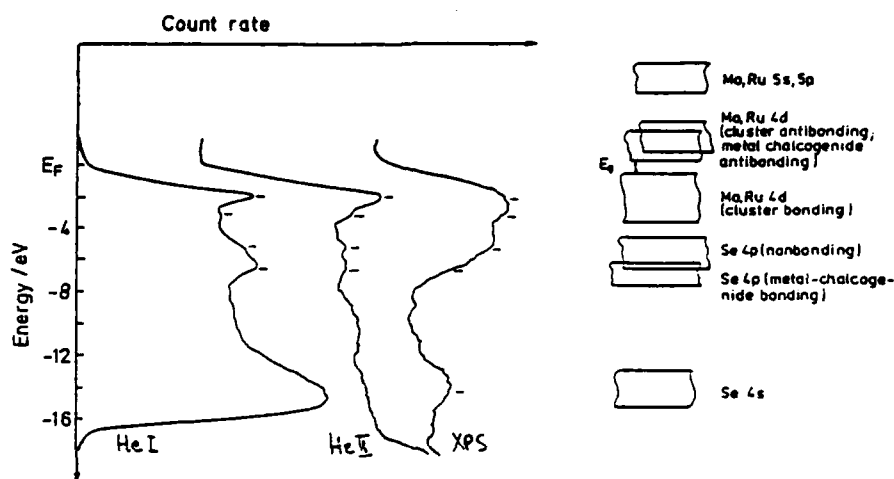
Fig. 2 Valence spectra of \text{Ru}_2\text{Mo}_4\text{Se}_8 and schematic density of state distribution
