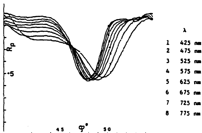
Fig.1 : R_p as a function of the angle of incidence \phi for various \lambda : Hg film (1.5 \mu\text{m} ) / water.
