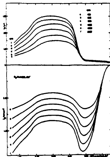
Fig.4. Rotating Au(100) -disk - Pt(poly) ring measurements of \text{O}_2 reduction in 0.1M NaOH. Sweep rate 50 \text{ mV s}^{-1} .
