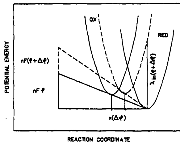
fig. 2: effect of electric field on the potential energy curve of the oxidized state
