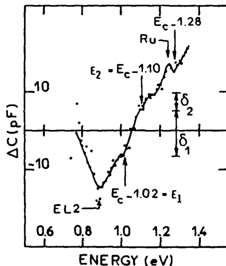
Figure 1 : PC spectrum corresponding to the junction n-GaAs/1M KOH modified by Ru electrodeposition. Surface preparation : etching.
