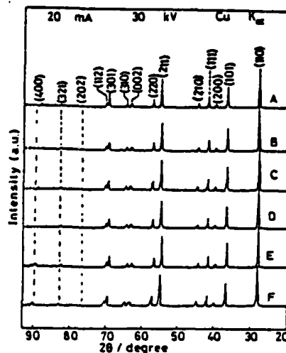
Fig. 1. X-ray diffractograms of the sintered \text{TiO}_2 specimens. The powders were heated prior to compressing, in an electrical furnace under static air for 9hr at 1000 °C. The compressed pellets labeled as A-F, all were sintered at temperatures between 800 to 1500 °C, for different time intervals ranged between 2 to 20 hr at each experimental temperature; where all other conditions were the same as for heating the original powders.
