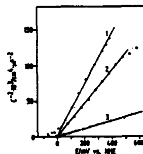
Fig. 2 Mott-Schottky behavior of anodic oxide films on Ti: 1. formed and measured in \text{H}_2\text{SO}_4 , 2. formed in \text{H}_2\text{SO}_4 and measured in \text{HNO}_3 , 3. formed and measured in \text{HNO}_3 .
