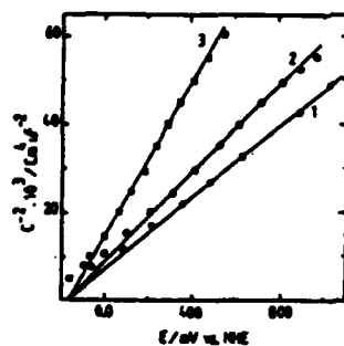
Fig. 3 Mott-Schottky plots of passivated titanium: 1. formed and measured in \text{H}_2\text{SO}_4 , 2. formed in \text{H}_2\text{SO}_4 and measured in \text{HNO}_3 , 3. formed and measured in nitric acid.
