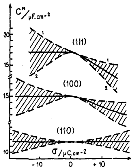
Fig. 3. Proposed electrode charge dependences of C^M for the (111), (100) and (110) faces of silver.
