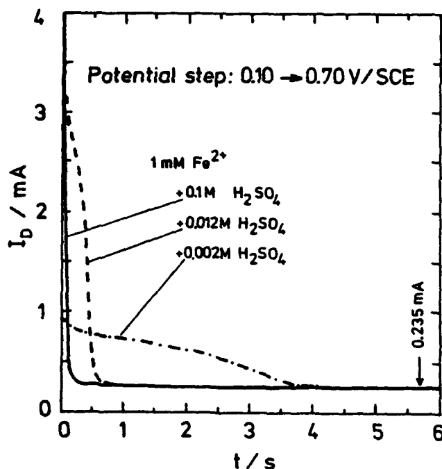
Figure 2: Current ( I_D ) transients observed with the rotated "Nafion"-coated platinum electrode in electrolytes of 1 mM \text{Fe}^{2+} in various concentrations of \text{H}_2\text{SO}_4 . Electrode area 0.27 \text{ cm}^2 .
