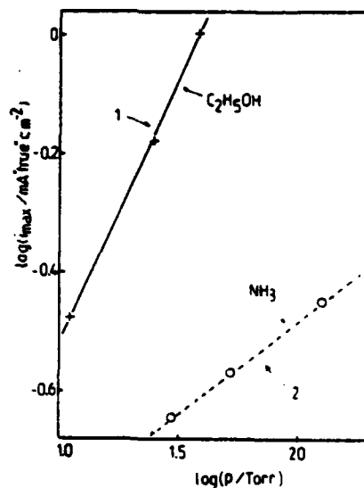
Figure 2 Dependence of i_{\text{max}} on the partial pressure p : 1) ethanol vapors from 11.5 to 37.5 Torr (r.f. 5.72); 2) ammonia vapors from 30 to 126 Torr (r.f. 4.50). Sweep rate 50 \text{ mV s}^{-1} , 1M \text{ NaOH} , 25^\circ\text{C} .
