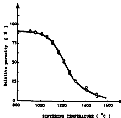
Fig. 2. Relationship between sintering temperature and the porosity variation of the \text{TiO}_2 specimens.
