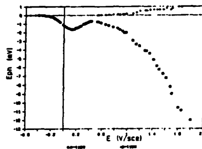
Fig. 2 - Photopotentials recorded during galvanostatic oxidation (200 nA/cm²) of tinplate in boric buffer.
