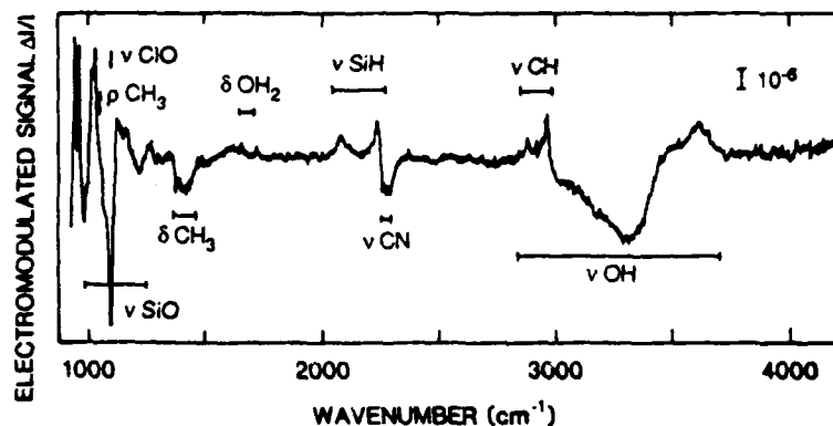
Fig.1. Typical electromodulated spectrum of a n-Si/acetoneitrile + 0.1M tetrabutylammonium perchlorate interface. Electromodulation potentials V_1 = -0.3\text{V} , V_2 = +0.3\text{V} . Reference is \text{Ag}/\text{Ag}^+ . Modulated charge 5 \times 10^{-7} \text{ C/cm}^2 . Here the infrared beam is unpolarized.
