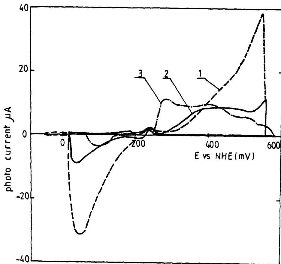
Fig.1. Photocurrent voltage curves. Curve for pure silver (1), Ag-0,44% Tl (2) and Ag-0,5% Pb (3). Wave length of incident photons is 400 nm and chopper frequency 2,1 cycle/s. Sweep rate 10 mV/s. Solution 1MKOH.
