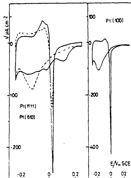
Fig. 3. Cyclic voltammograms for Pt(100), Pt(11,1,1) and Pt(610) in 0,1M HNO 3 . Sweep rate 50 mV/s.
