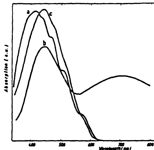
FIG. 2. Absorption spectra of 6T on \text{SnO}_2 glass. a : as deposited. b : after electrochemical oxidation. c : after electrochemical reduction.
