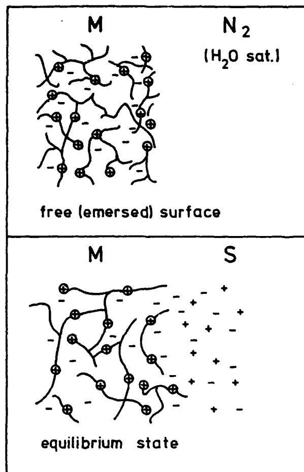
Fig. 2 The surface dipole layer generated upon emersion of a anion-exchange membrane.
