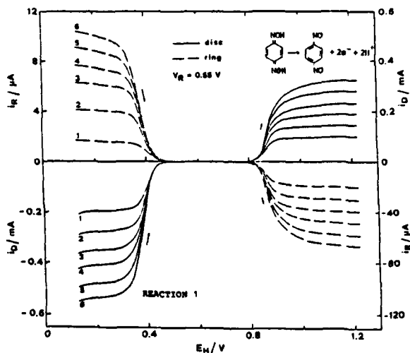
Fig. 1. Ring-disc measurements for p-benzoquinone dioxime ( 10^{-3} M) reduction and oxidation on Pt in 0.5 \text{ M HClO}_4 in the presence of 2.5 \times 10^{-4} \text{ M Bi(ClO}_4)_3 . |dE/dt| = 10 \text{ mV s}^{-1} . Rotation frequency f Hz: (1) 8.33; (2) 18.33; (3) 33.33; (4) 50; (5) 75; (6) 100.
