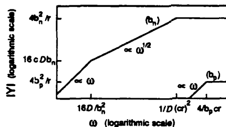
Fig.3. Faradaic impedance of a spherical pore of radius b in the presence of diffusion. Two different cases for b are shown ( b_n \gg Dcr \gg b_p ). Here c stands for (z^2 e^2 / kT) c_{red} c_{ox} / (c_{red} + c_{ox}) .
