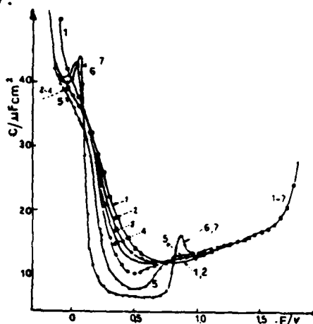
Fig.1-Differential capacity curves of a Hg electrode in 0.5M NaClO 4 in EG solutions at various LN concentrations: (1) 0; (2) 0.0005; (3) 0.0010; (4) 0.0025; (5) 0.0050; (6) 0.0075; (7) 0.010M.
