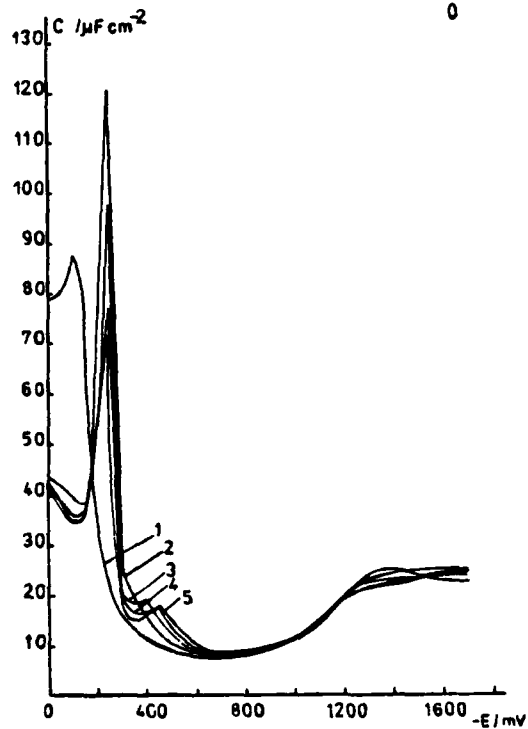
Fig.2. Double layer capacity curves for 0.1M phosphate buffer in H 2 O + 20% vol.EtOH containing \beta -CD at the following concentrations: (1) 0, (2) 3.14, (3) 6.28, (4) 9.41, (5) 12.5 mmol·l -1
