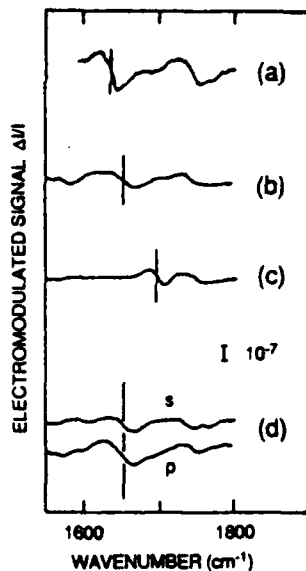
Fig.3. \delta OH 2 spectrum for different solvents ((a) nitromethane, (b) acetonitrile, (c) dimethylsulfoxide) and light polarizations ((d) in acetonitrile). Notice the shifting upon changing the solvent. The feature near 1740 cm -1 may be ascribed to a surface contaminant.
