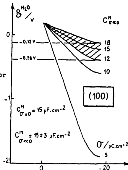
Fig. 2. g_{\sigma=0}^{H_2O} as a function of \sigma .
