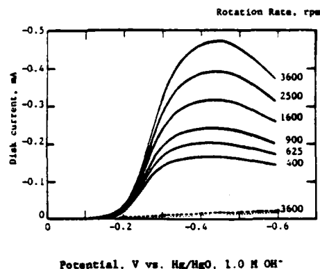
Fig. 2. Disk currents for O_2 reduction on HOPG with adsorbed 9, 10-phenanthrenequinone in O_2 -saturated 1.0 M NaOH at 22^\circ\text{C} . Scan rate: 20 \text{ mV s}^{-1} ; electrode area: 0.169 \text{ cm}^2 ; basal plane without quinone (---).
