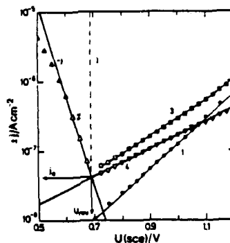
Fig.1. Initial polarization data for titanium electrode stabilized (20 h) at 0.9\text{ V(sce)} in 0.5\text{ M H}_2\text{SO}_4 . The curves 1,2 and 3 represent measurements in 0.5\text{ M H}_2\text{SO}_4 , in 0.5\text{ M H}_2\text{SO}_4 - 0.009\text{ M V(OH)}_4^+ and in 0.5\text{ M H}_2\text{SO}_4 + 0.1\text{ M VO}^{2+} + 0.009\text{ M V(OH)}_4^+ , respectively. Curve 4 is the difference between the curves 3 and 1. Open symbols apply to Wagner-Traud corrected data.
