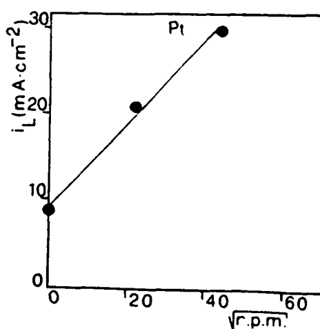
Fig. 4 - i_L for the h.e.r. in 0.1 N HF on bright platinum disk as a function of the rotation speed (r.p.m.)
