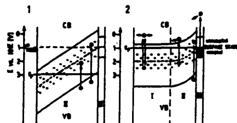
Fig. 4 Schematic model of the band structure of \text{TiO}_2 formed on Ti in 1 N \text{HNO}_3 solution. 1. Polarization potential E = 2.95 \text{ V} ; 2. Polarization potential E = 0.95 \text{ V} . E_p = Fermi level, --- = unoccupied impurities in the band gap, ... = occupied impurities in the band gap.
