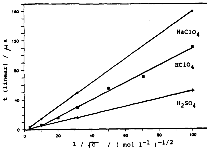
Figure 2 Time elapsed during the linear portion of the transients vs. 1/\sqrt{C} for immersion of Au into \text{HClO}_4 , \text{H}_2\text{SO}_4 and \text{NaClO}_4 solutions.
