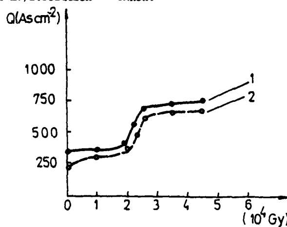
Fig.2. Charge and discharge capacity of pure silver electrode vs absorbed energy \gamma -ray. Solution 1MKOH.
