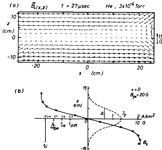
Fig. 2. (a) Magnetic field vector map ( B_x, B_z ) in the x - z plane ( y = 137 cm from cathode), showing the classical neutral sheet topology. The field configuration is quasi stationary, i.e. unchanged as long as external flux is supplied. ( B_{y0} \approx 20 G = const). (b) Magnetic field variation B_x(z) across the neutral sheet yields the current density profile J_y(z) = (\partial B_x / \partial z) / \mu_0 . The half width \Delta \approx 5 cm is smaller than characteristic ion scale lengths ( c/\omega_{pi} \approx 60 cm, r_{ci} \approx 12 cm), but larger than electron lengths ( c/\omega_{pe} \approx 0.7 cm, r_{ce} \approx 0.4 cm). The current is carried by electrons.
