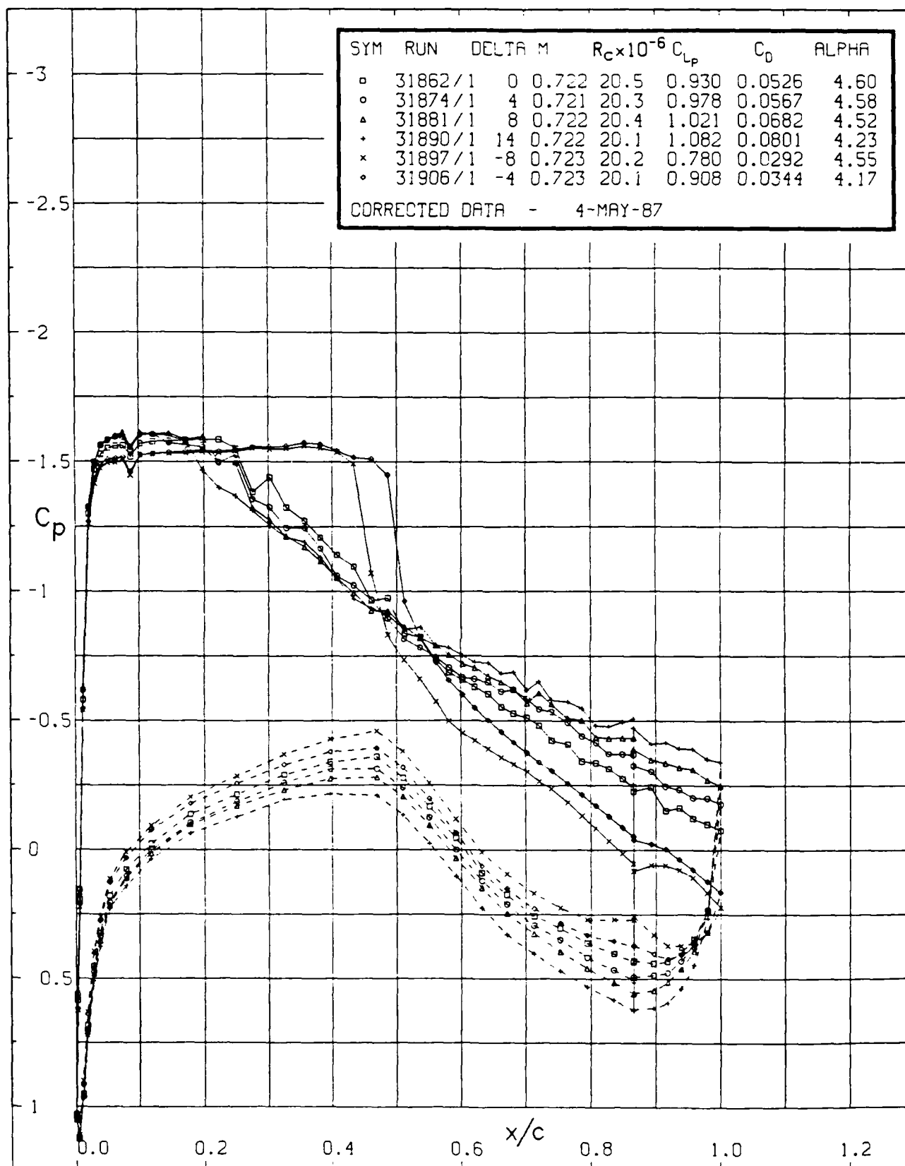
FIG. 19: SURFACE PRESSURE DISTRIBUTIONS AT M ABOUT 0.723 FOR VARIOUS FLAP ANGLES AT \alpha ABOUT 4.5^\circ
