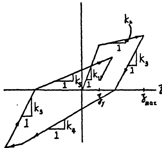
Fig. 8.1 The Q-hysteresis
