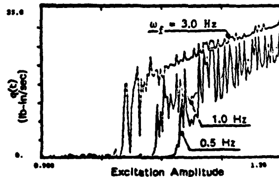
Fig.9.7 Structural Power vs Excitation Amplitude
