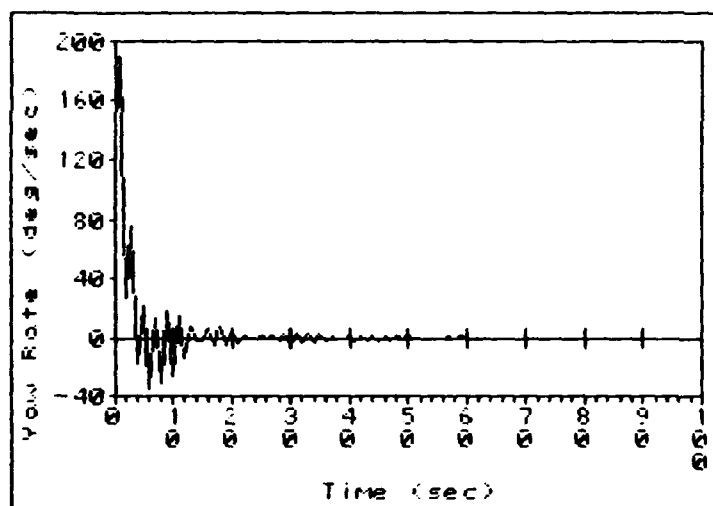
Figure 24. Yaw Attitude Response to Shuttle Docking Impulse
