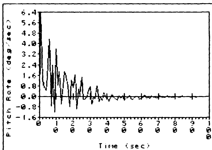
Figure 19. Pitch Attitude Response to Crew Disturbance Impulse
