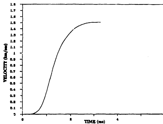
Figure 10. Conventional Firing: Simulation of In-Bore Velocity
