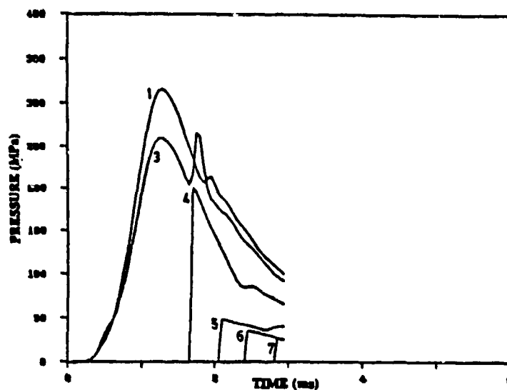
Figure 20. Late TC Ignition: Simulation of P. ID 44. Altered TC Burn Rate
