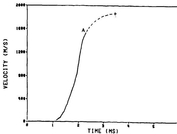
Figure 12. Late TC Ignition: Experimental V. ID 44
