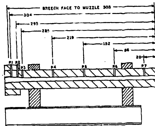
Figure 4. 14-mm Test Fixture: Units in CM
