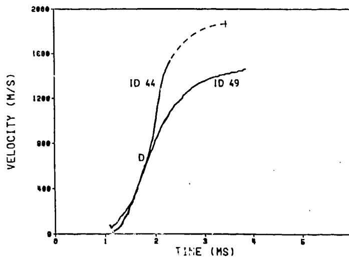
Figure 15. Experimental In-Bore Velocities: No TC Ignition (ID 49), Late TC Ignition (ID 44)
