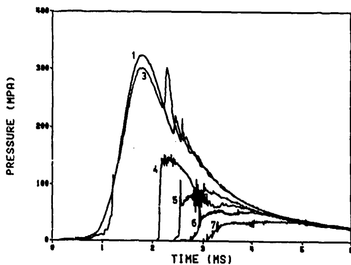
Figure 11. Late TC Ignition: Experimental P. ID 44
