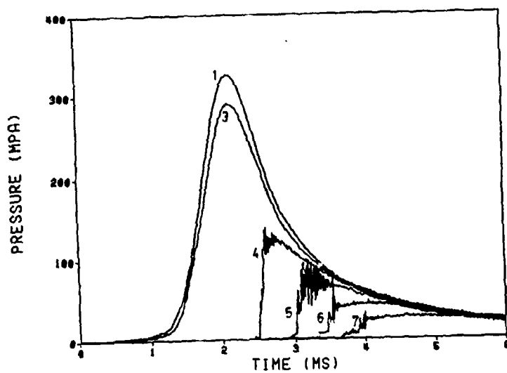
Figure 7. Conventional Firing: Experimental Pressures
