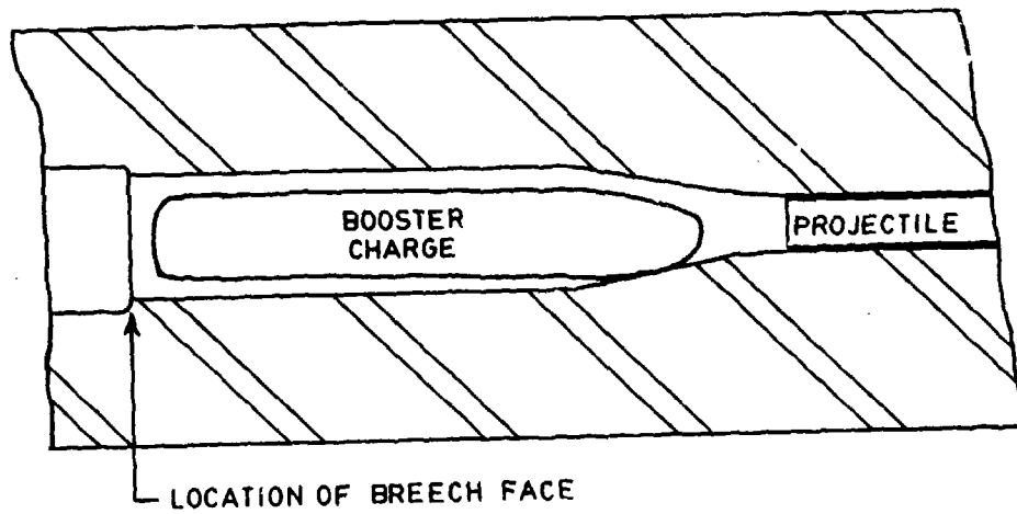
Figure 6. Booster Charge, Chamber and Projectile Schematic
