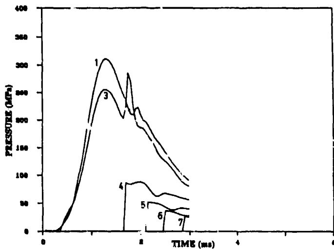
Figure 18. Late TC Ignition: Simulation of P, ID 44
