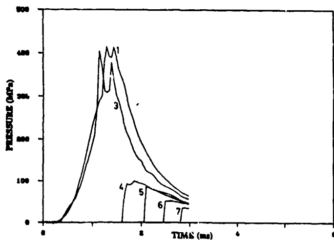
Figure 21. Early TC Ignition: Simulation of P. ID 51
