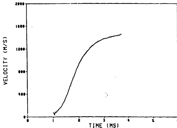
Figure 14. No TC Ignition: Experimental V. ID 49
