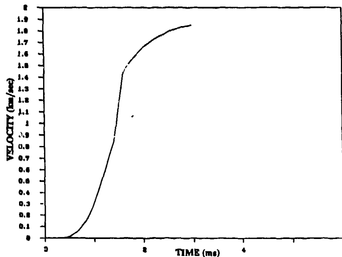
Figure 19. Late TC Ignition: Simulation of V, ID 44
