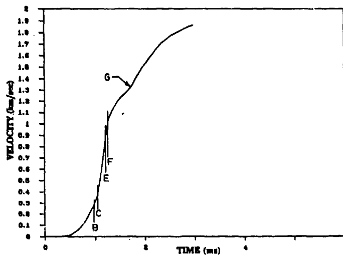
Figure 22. Early TC Ignition: Simulation of V. ID 51
