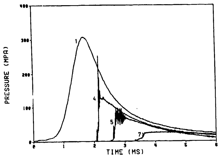
Figure 13. No TC Ignition: Experimental P. ID 49
