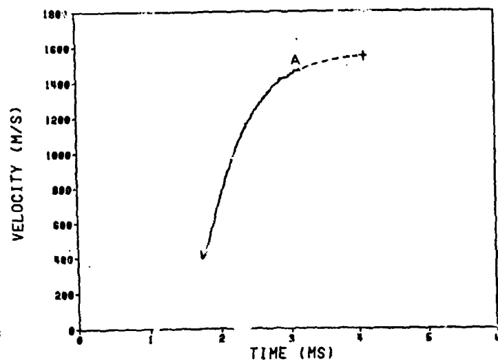
Figure 8. Conventional Firing: Experimental In-Bore Velocity
