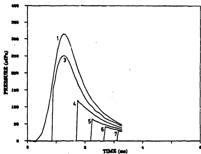
Figure 9. Conventional Firing: Simulation of Pressure
