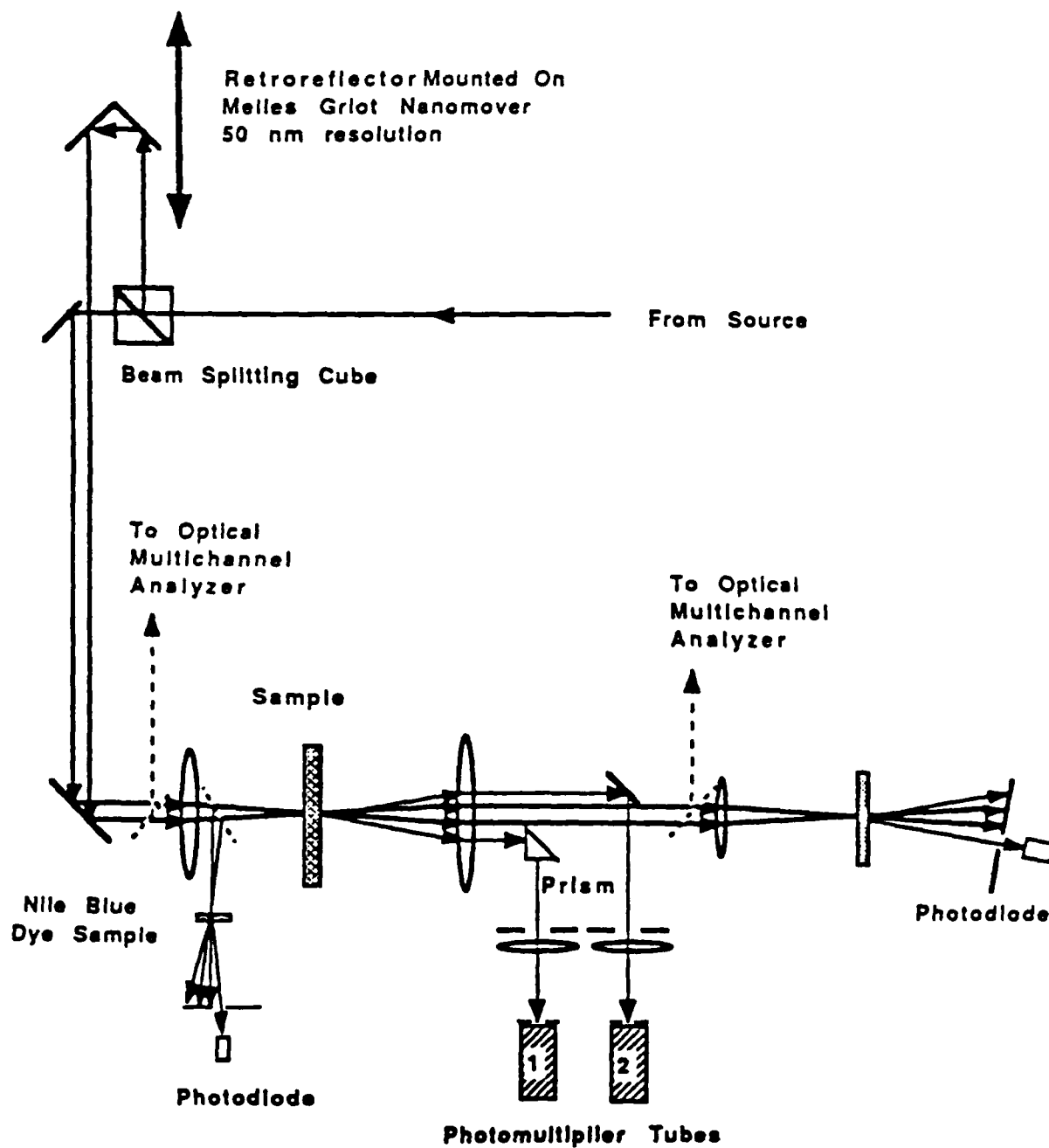
Figure 2. Experimental apparatus.
