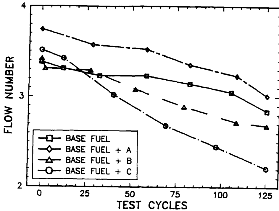
Figure 8. Degradation of flow capacity of primary fuel nozzles during 125-cycle test
