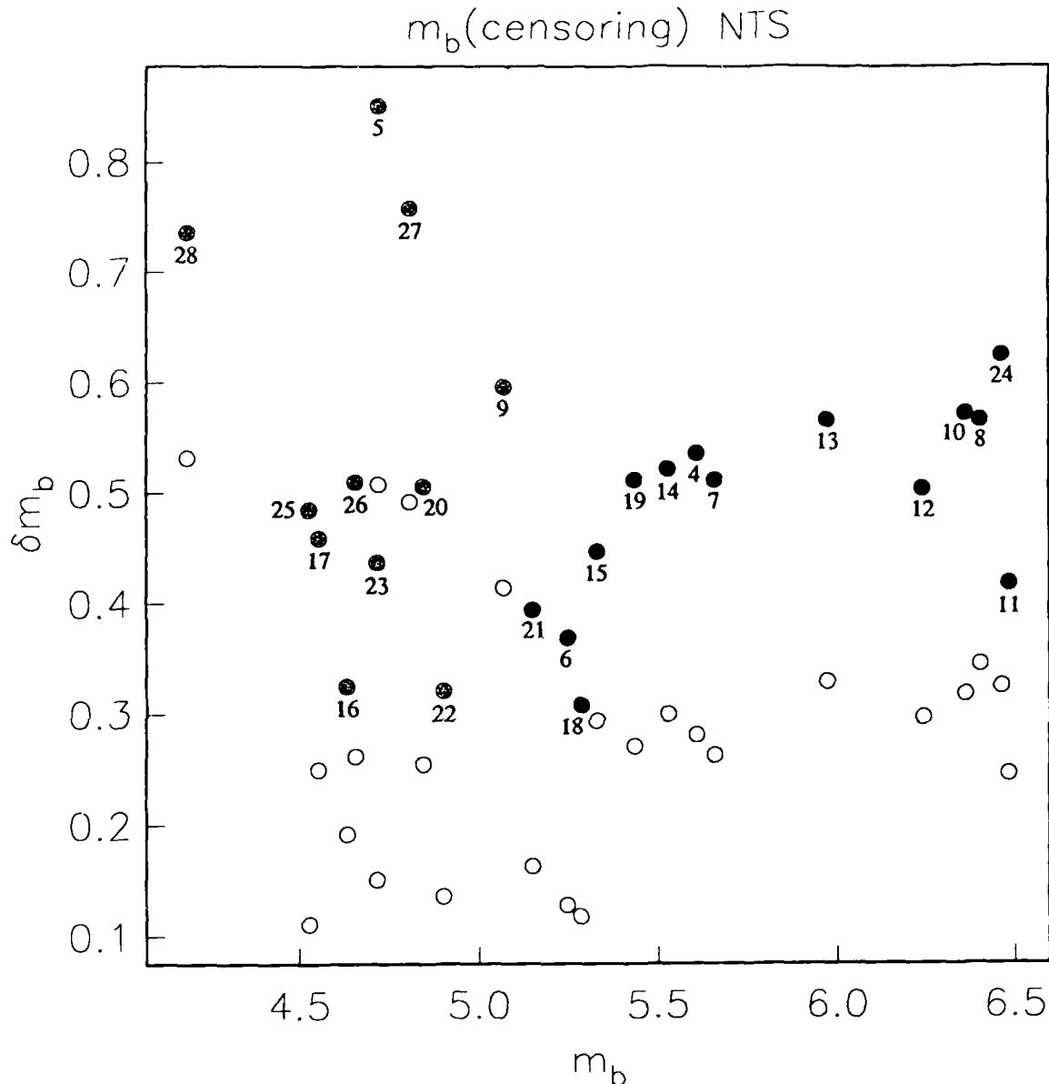
Figure 12c. m_b(\text{max}) 's plotted against \delta m_b 's for NTS. The m_b 's are maximum likelihood estimates with the censoring information. The solid circles are m_b(\text{max})-m_b(a) and the open circles are m_b(\text{max})-m_b(b) for the corresponding event. The events are listed in Table 2. The hatched circles are m_b(\text{max})-m_b(a) for which there are less than 10 "a" phase signal readings.
