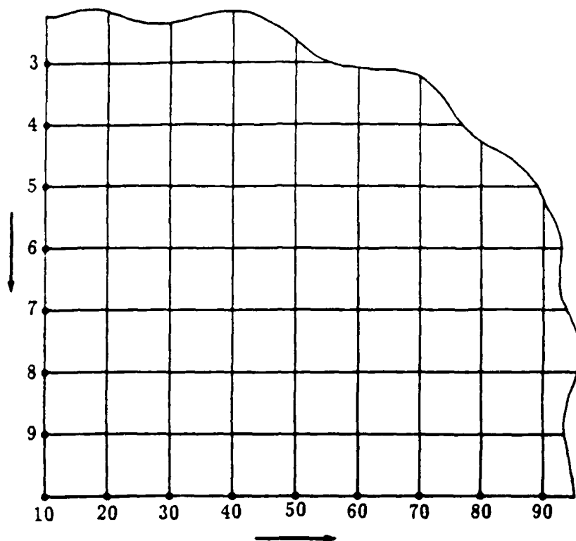
Figure 3.4 Order of Nodes Along a Nonreflecting Boundary
