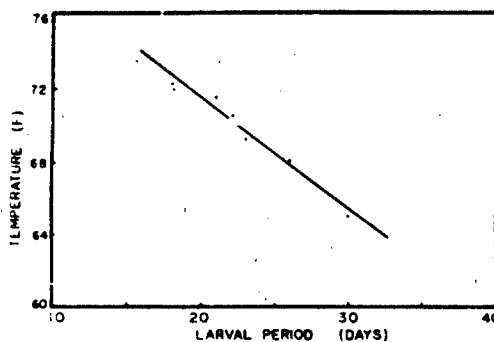
Figure 6. Duration of the larval period in Pacific oysters at various temperatures in British Columbia (after Quayle 1969a).
