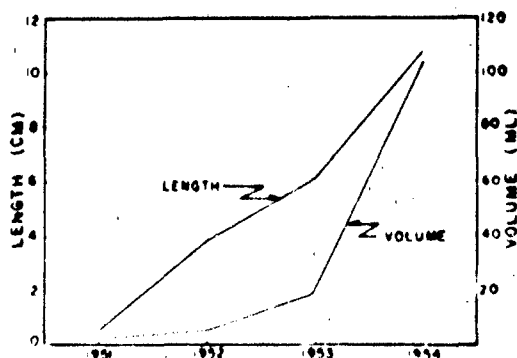
Figure 3. Length and volume increases of Pacific oysters followed over 4 consecutive years in British Columbia (after Quayle 1969a, Pacific Oyster Culture in British Columbia , Fisheries Research Board of Canada, with permission of the Department of Fisheries and Oceans).
